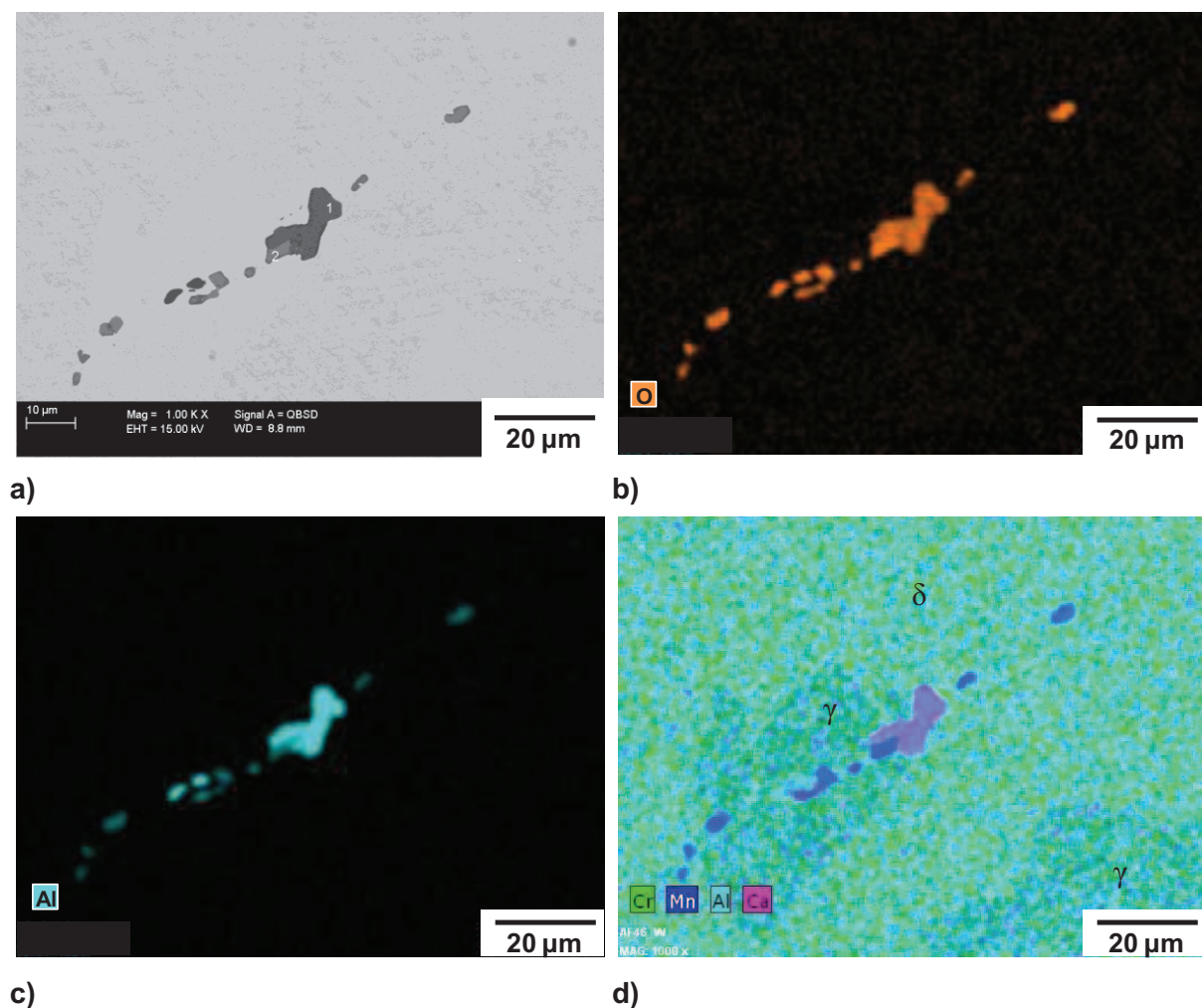
Figure III.52. Nature of the inclusions present in the D1_W and D1bis_W microstructures; a) SEM micrograph showing a string of particles; b) chemical composition map in oxygen; c) chemical composition map in aluminium; d) chemical composition map superimposing chromium, manganese, aluminium and calcium.
