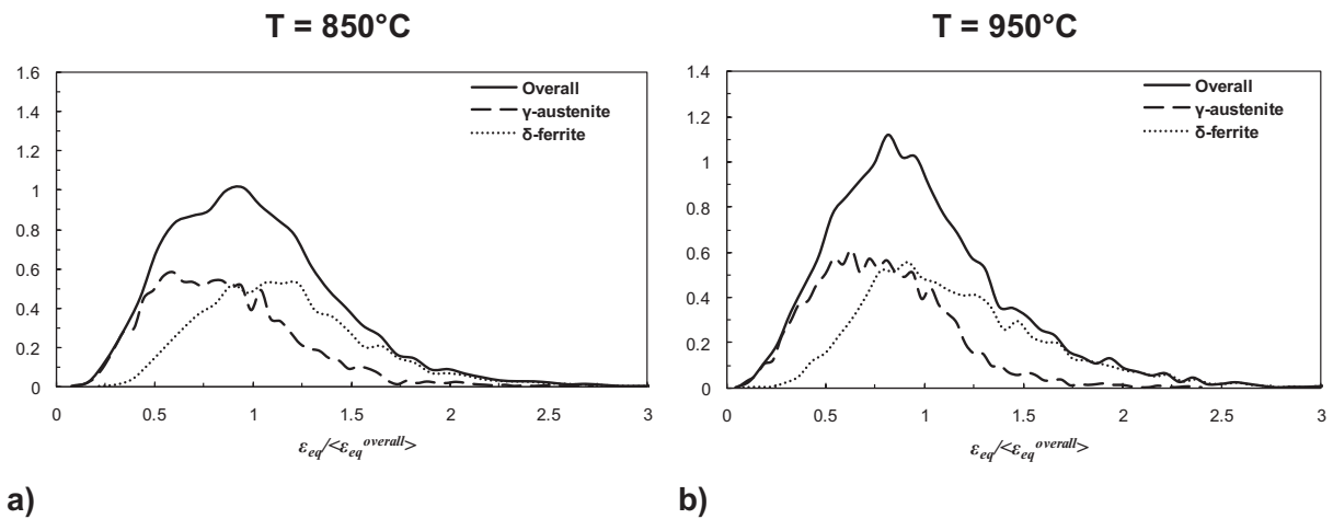
Figure IV.38. Strain distribution functions relative to the volume fraction of phase for the equiaxed morphology: D1_E. a) D1_E, T = 850^{\circ}\text{C} . b) D1_E, T = 950^{\circ}\text{C} .
