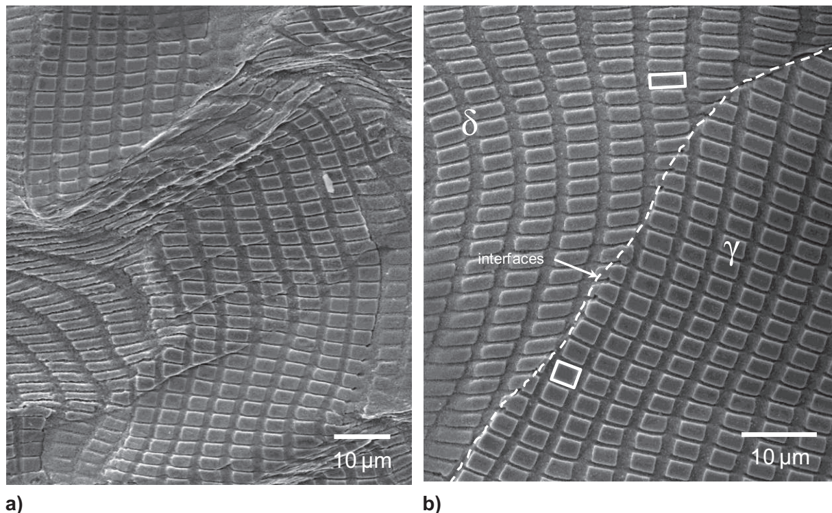
Figure IV.25. Illustration of the heterogeneity of the deformation in the D2_W microstructure after plane strain compression at 850°C and at a strain rate of 1\text{s}^{-1} ; a) SEM pictures showing strongly deformed areas and slightly distorted regions; b) SEM picture showing the strain partitioning between ferrite and austenite. The square in the austenite indicates a slight deformation in the austenite whereas the rectangle shape in the ferrite emphasizes a significant deformation in the ferrite. The compression axis is the vertical direction.
