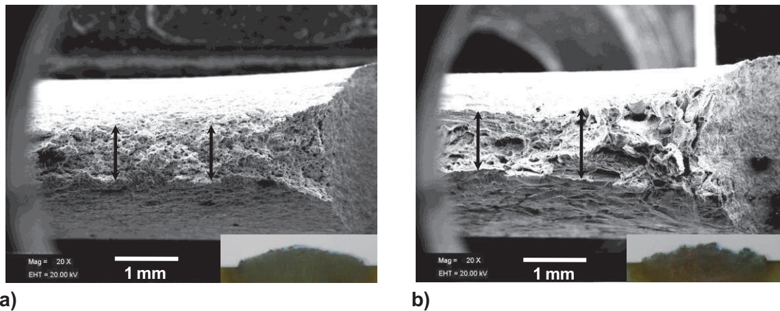
Figure III.41. Fracture micrographs and profiles of the broken DENT at 1050°C; a) D2_E ( l_0=35\text{mm} ); b) D2_W ( l_0=37\text{mm} ).
