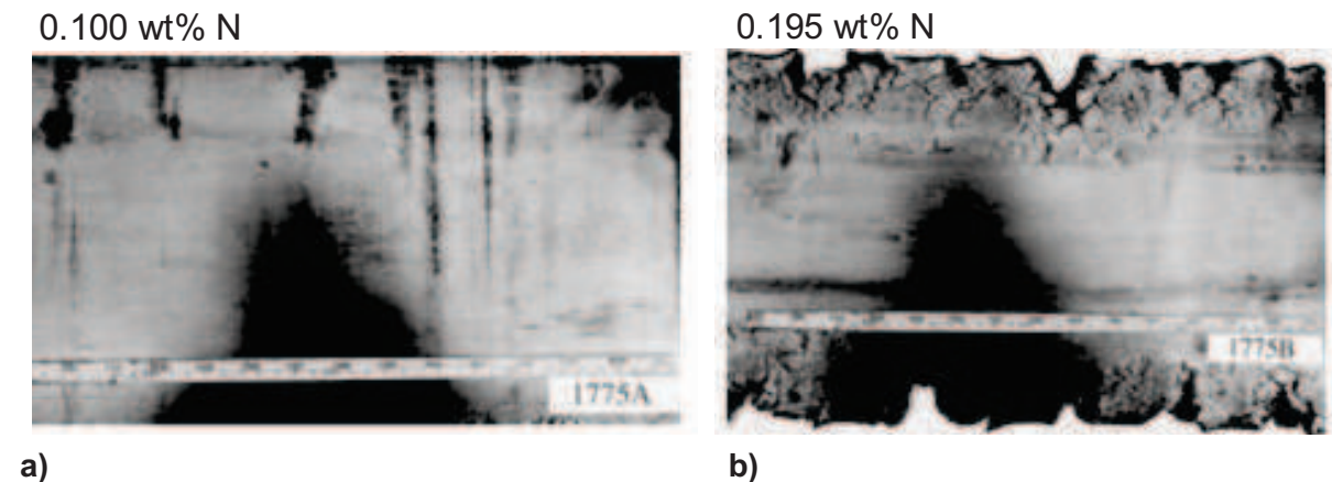
Figure II.20. Influence of N content on the hot workability of a 2205 duplex stainless steel; the level of edge cracking increases with the N content; a) 0.100 wt %N, CSI = 5.9; b) 0.195 wt %N, CSI = 7.7 [59].
