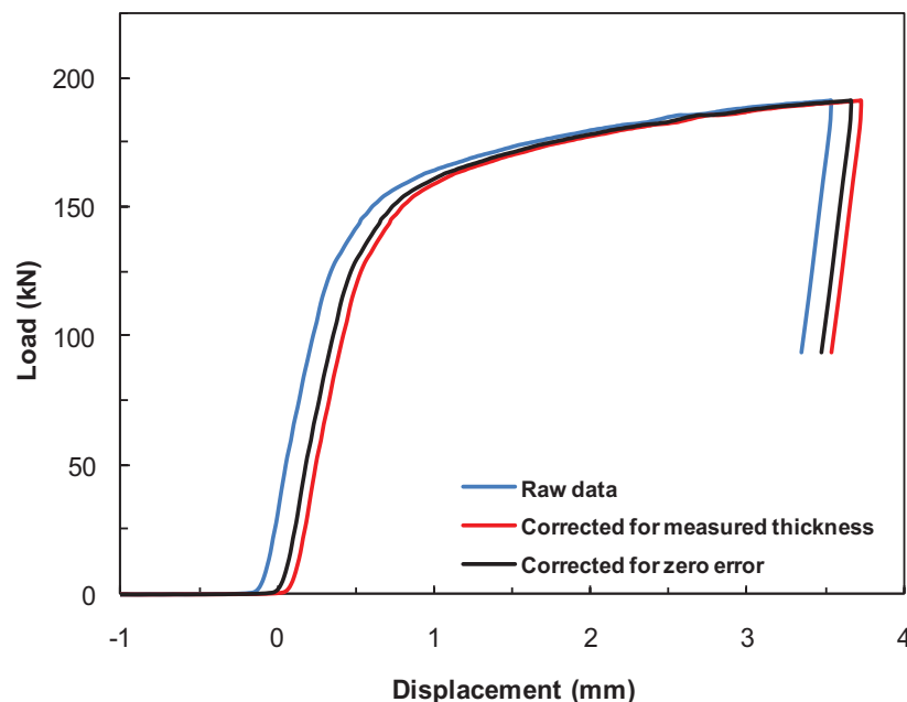
Figure A.2. Origin corrections, taken from a single deformation carried out at 850^{\circ}\text{C} and 1\text{s}^{-1} .
