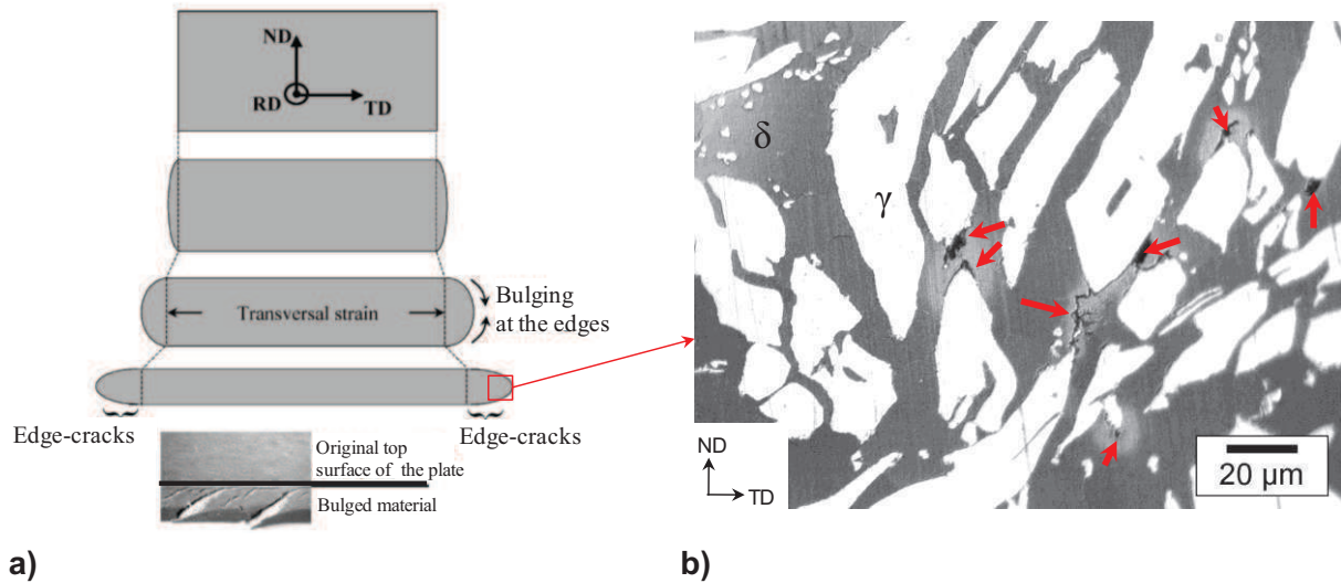
Figure I.9. a) Evolution of the transverse dimensions of the hot rolling blocks with increasing reduction; a clear transverse strain develops and cracks have been observed only in the bulged region; b) microstructure in the edge part illustrating the damage; red arrows emphasize the voids.
