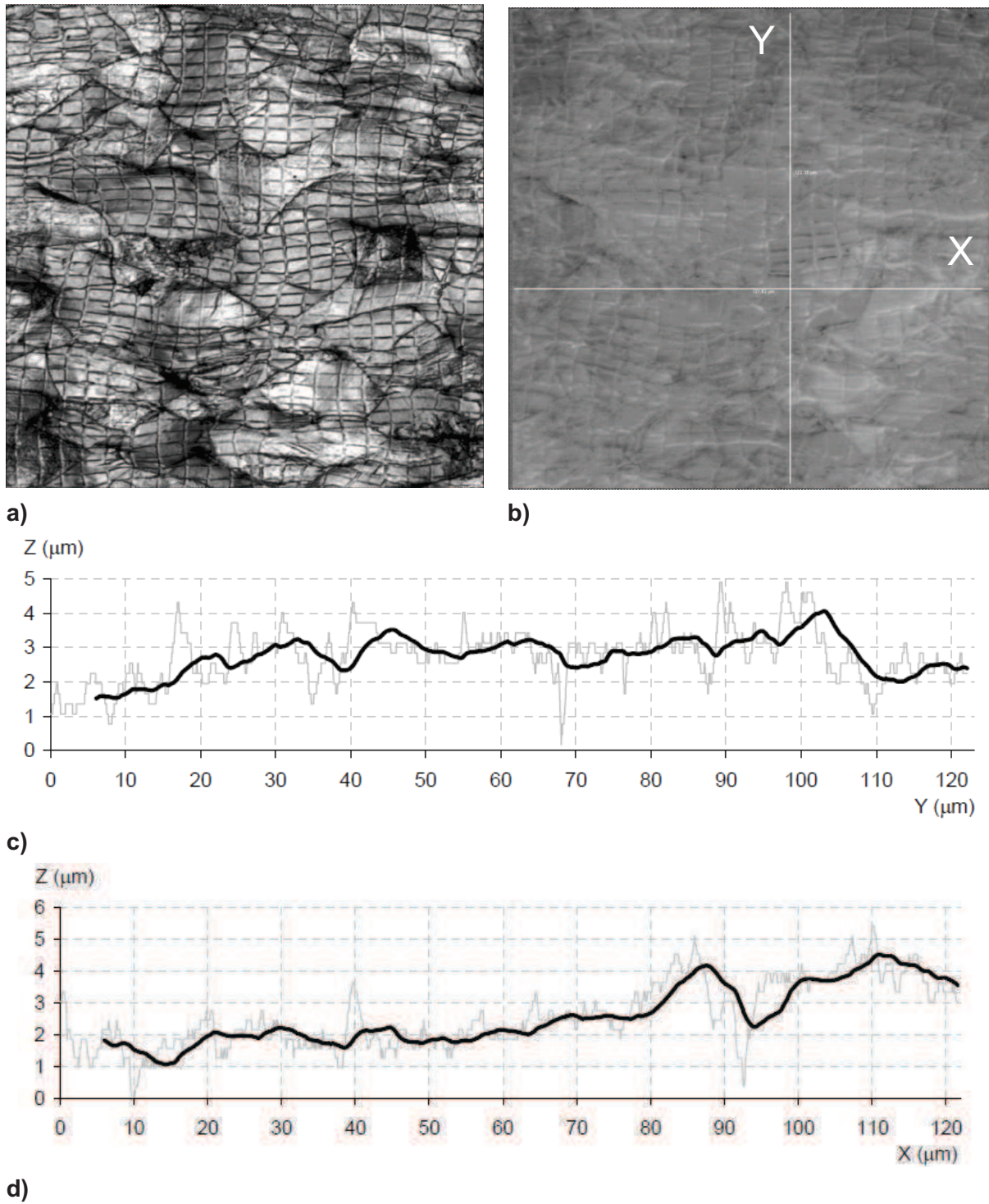
Figure IV.44. a) Optical micrograph of a small area (125x125μm) from a deformed microgrid on a laboratory duplex steel sample; b) grey scale topological image of the same area in a); c) and d) height profiles of the vertical and horizontal lines in b), respectively. The thinner and thicker lines in c) and d) correspond to the original profiles and their smoothed versions respectively.
