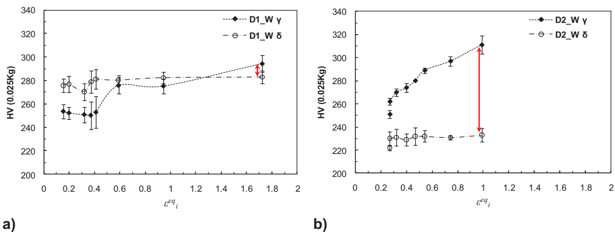
Figure III.36. Micro-hardness profiles along the homogeneous zone of DENT specimens in both phases; a) D1_W, T=1050°C; b) D2_W, T=1050°C.
