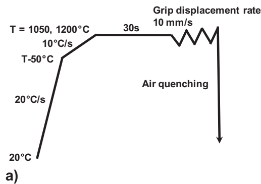
Figure III.6. a) The thermo-mechanical history path followed by the DENT specimens; b) picture showing the shape of the heated zone.
