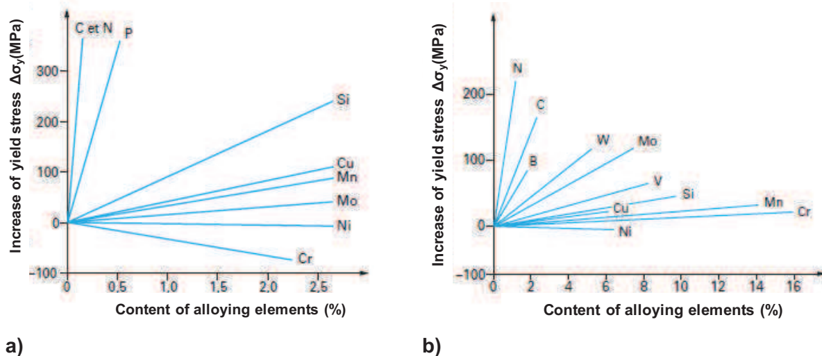
Figure IV.31. Influence of alloying content on the yield stress of a) ferrite and b) austenitic stainless steel at room temperature.
