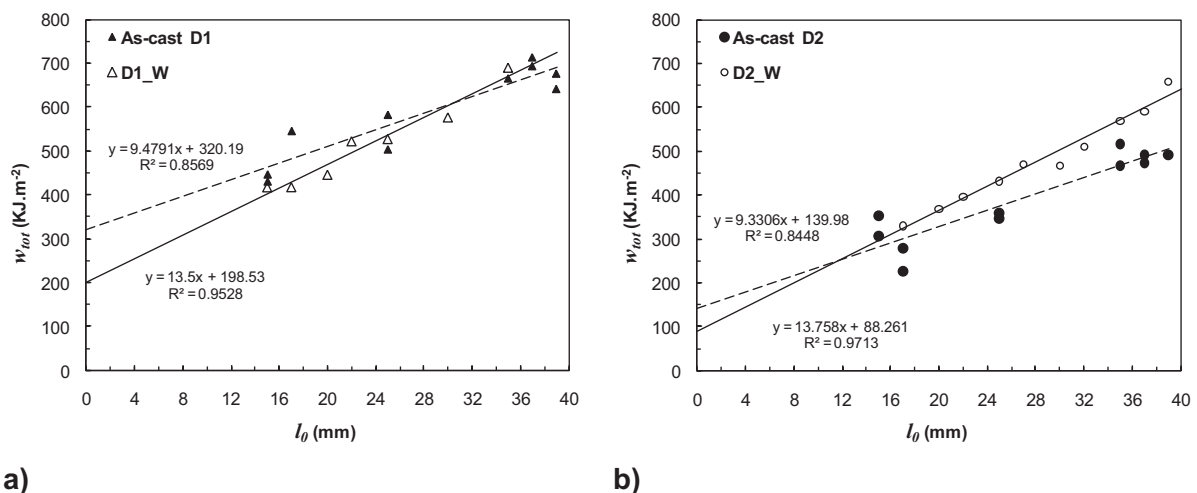
Figure III.37. Comparison of the EWF results obtained in the as-cast conditions with those obtained starting from model Widmanstätten microstructures at T=1050°C; a) Alloy D1; b) Alloy D2.
