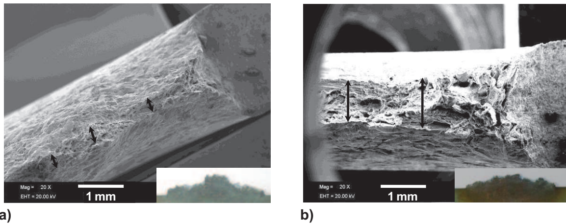
Figure III.33. Fracture micrographs of the broken DENT at 1050°C; a) D1_W ( l_0=35mm ); b) D2_W ( l_0=37mm ).
