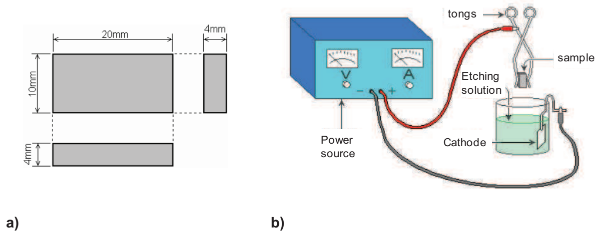
Figure IV.6. a) Dimensions of the small samples used to engrave the microgrids; b) schematic of the electro-etching circuit.
