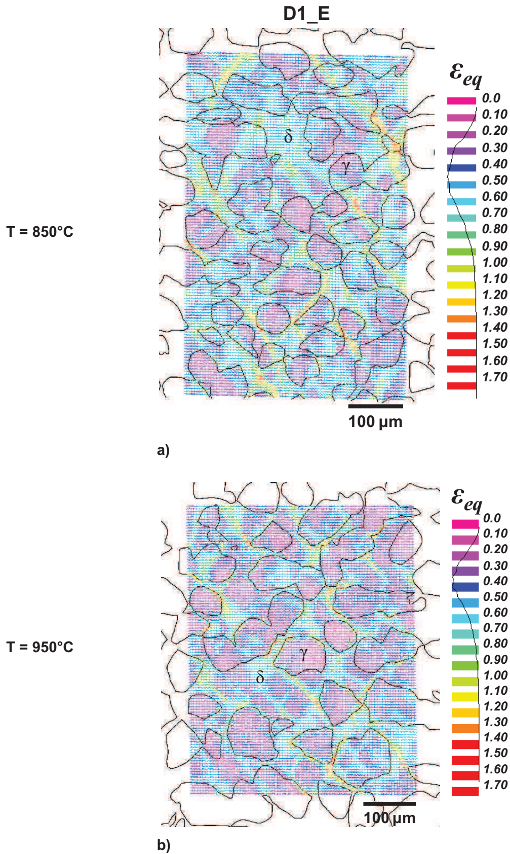
Figure IV.37. Equivalent strain distribution maps of the equiaxed morphology: D1_E at T = 850 and 950^{\circ}\text{C} for a 20% macroscopic thickness reduction; a) strain map at T = 850^{\circ}\text{C} ; b) strain map at T = 950^{\circ}\text{C} . The equivalent strain map is superimposed with the undeformed microstructure to clearly present where in the microstructure the strains are distributed. The loading direction corresponds to the vertical axis.
