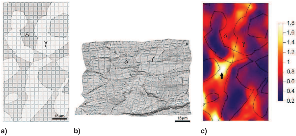
Figure II.14. Highlighting of strain partitioning via the microgrid technique in a laboratory 29.6%Cr-11.6%Ni-0.27%Mn duplex steel deformed at 950°C and 1\text{s}^{-1} ; a) undeformed state of a relatively small area; b) deformed configuration of the same area; c) distribution of the Green-Lagrange equivalent Von Mises strain [19].
