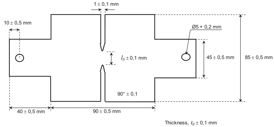
Figure III.5. Dimensions of the DENT (Double Edge Notch Tension) specimens used, t_0 = 3 \text{ mm} .
