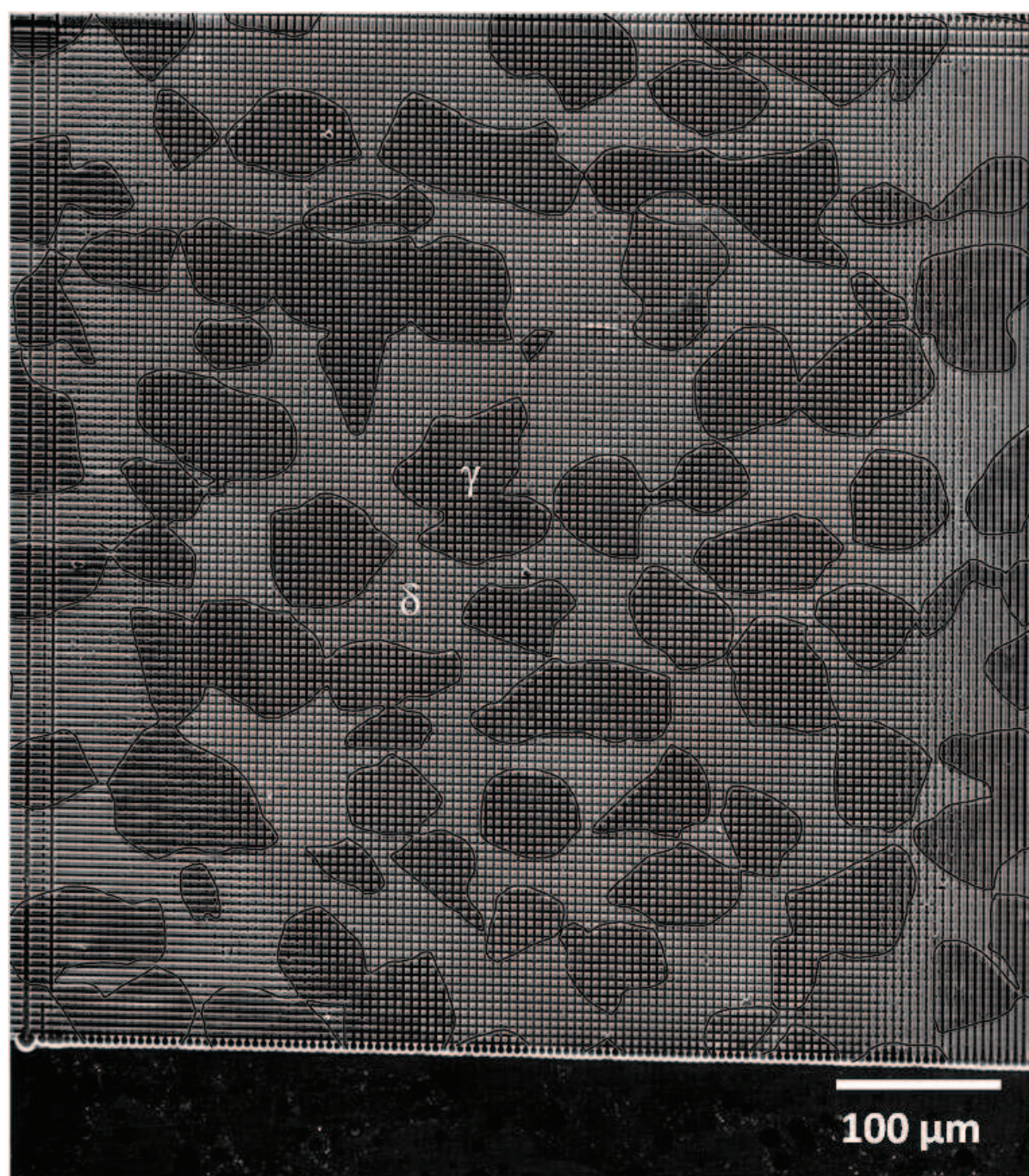
Figure C. 5. High resolution SEM micrograph of the D1_E microstructure in the undeformed configuration; sample B. The compression will be applied vertically.
