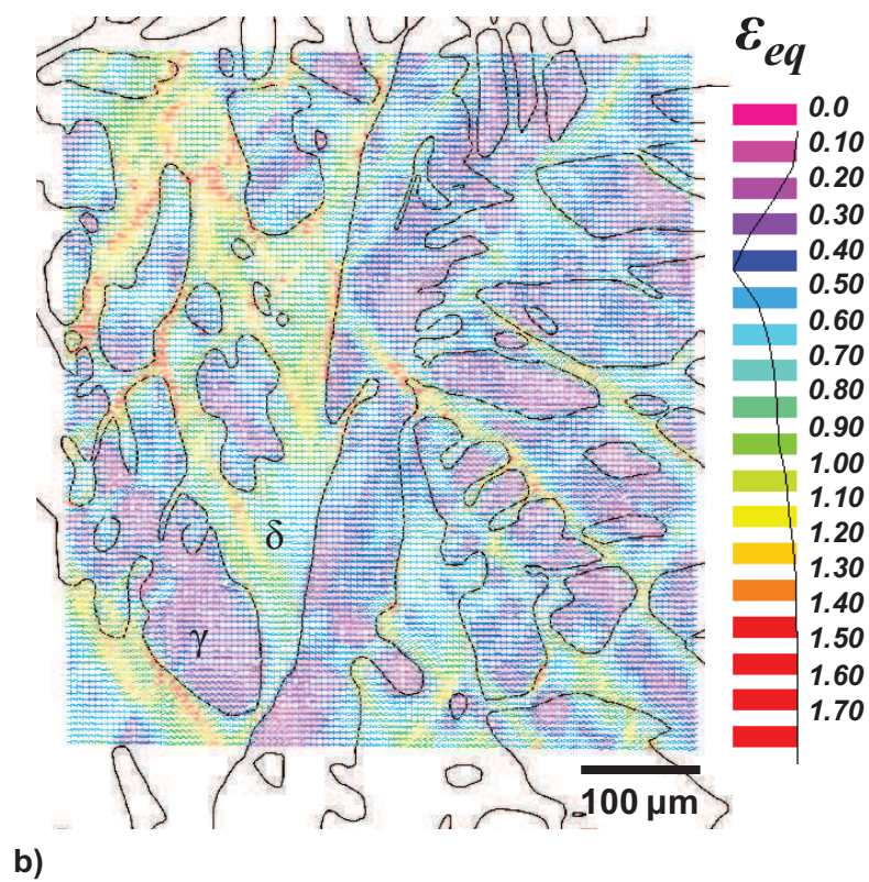
Figure IV.24. Equivalent strain distribution maps of the D2_W microstructure; a) map 1; b) map 2; the equivalent strain map is superimposed with the undeformed microstructure to clearly present where in the microstructure the strains are distributed; the compression axis corresponds to the vertical axis.
