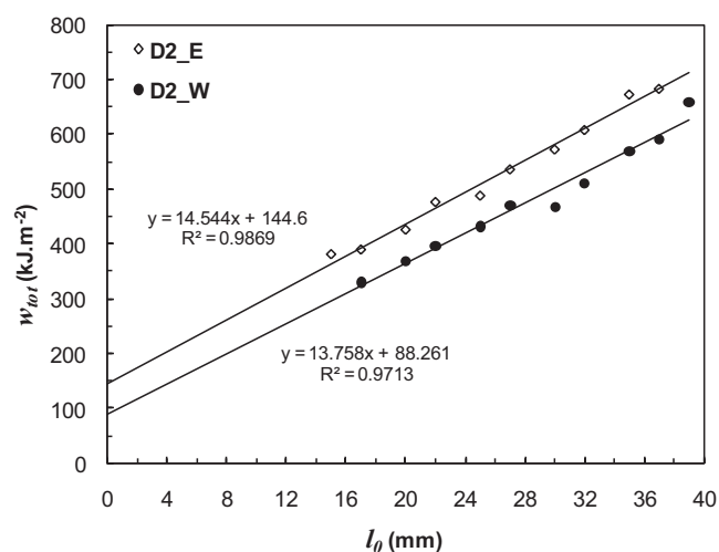
Figure III.40. Variation of the specific work of fracture as a function of the ligament length for separation of the essential work of fracture. Comparison between the two microstructures at 1050°C: D2_E and D2_W.
