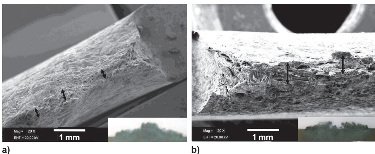
Figure III.50. Fracture micrographs and profiles of the broken DENT at 1050°C; a) D1_W ( l_0=35\text{mm} ); b) D1bis_W ( l_0=35\text{mm} ).
