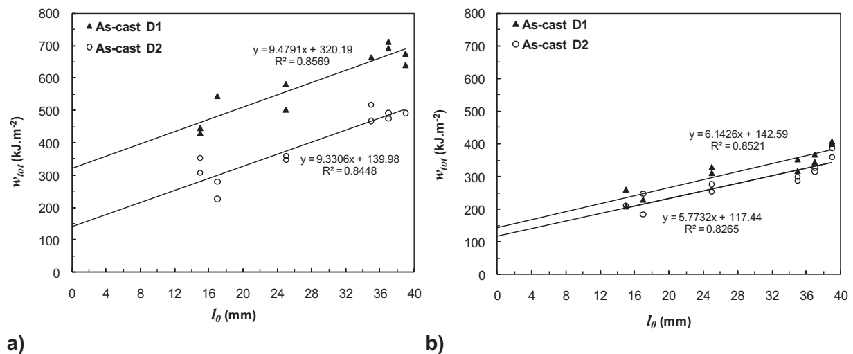
Figure III.12. Variation of the total specific work of fracture as a function of the ligament length for separation of the essential work of fracture; comparison between the two grades D1 and D2 in the as-cast conditions; a) T=1050^\circ\text{C} ; b) T=1200^\circ\text{C} .
