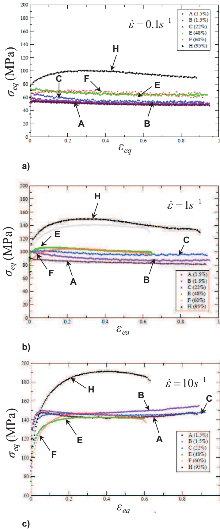
Figure II.11. Equivalent flow stress strain curves of different duplex stainless steels deformed under plane strain compression at 1050°C and at different strain rates; a) 0.1 s^{-1} ; b) 1 s^{-1} ; 10 s^{-1} . The value between the parenthesis gives the austenite content [42].
