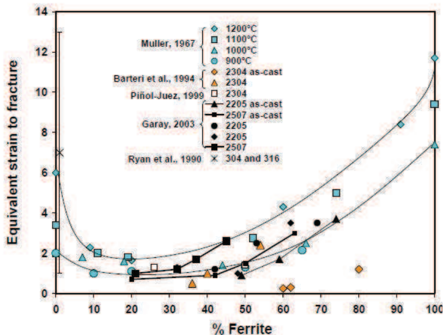
Figure II.19. Effect of the volume fraction of ferrite and temperature deformation on the strain to fracture for different duplex stainless steels [20].
