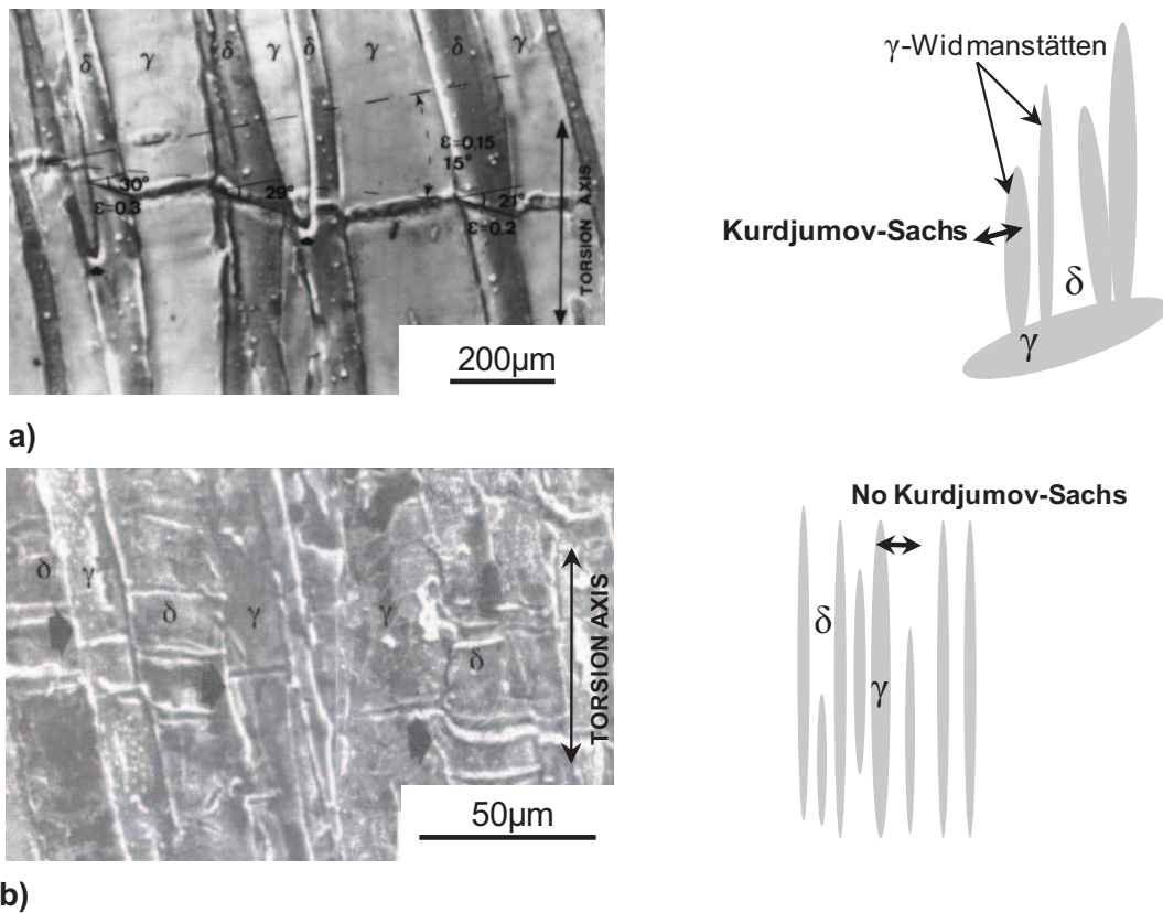
Figure II.5. SEM micrographs showing the surface of two marked specimens of a 2304 duplex stainless steel deformed to 0.17 under torsion at 1000°C and 1\text{s}^{-1} ; a) in the as-cast condition, \delta is related to \gamma by a Kurdjumov-Sachs orientation relationship; b) in the hot-rolled condition (reduction 77%), no lattice correspondence between \delta and \gamma [12].
