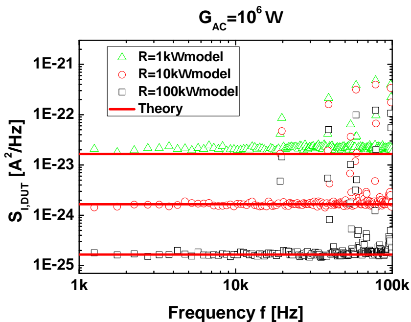
Figure 3.25: S_{I,DUT} as a function of frequency f , model -Eq.(3.34)- (dots) vs. theoretical values -Eq.(3.36)- (solid lines), for 1k\Omega , 10k\Omega and 100k\Omega resistances with G_{AC} = 10^6 \Omega .
