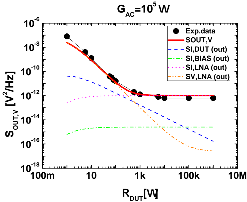
Figure 3.20: Lines: S_{OUT,V} , S_{I,DUT}(out) , S_{I,BIAS}(out) , S_{I,LNA}(out) and S_{V,LNA}(out) as a function of R_{DUT} , calculated using Eq.(3.33) and Eq.(3.35), for G_{AC} = 10^5\Omega . Dots refer to experimental S_{OUT,V} data.
