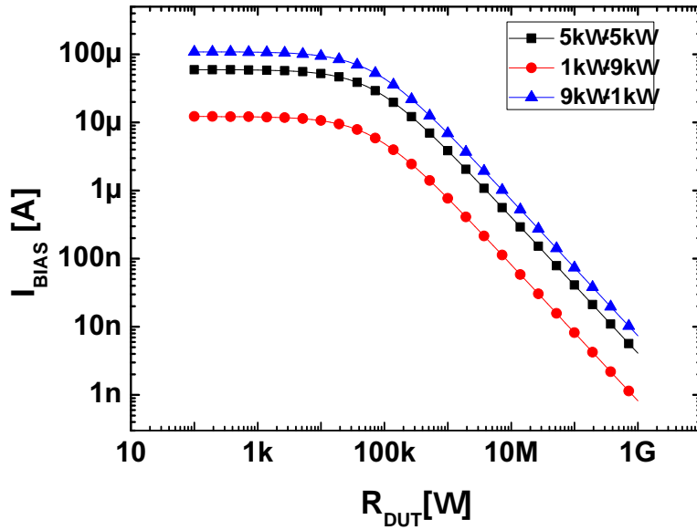
Figure 3.6: I_{BIAS} as a function of R_{DUT} for different combination of the potentiometric resistance R_P (indicated in the legend).
