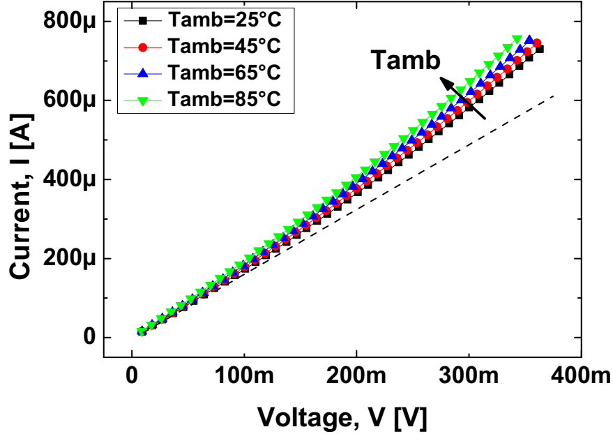
Figure 4.2: Experimental I - V characteristics at low voltages (i.e. readout region) of our f_{cc} GST-based PCM cells at T_{amb} = 25^\circ\text{C} , 45^\circ\text{C} , 65^\circ\text{C} , and 85^\circ\text{C} (symbols+line plots). In dash-type line the linear extrapolation of the ohmic region of the curve at T_{amb} = 25^\circ\text{C} .
