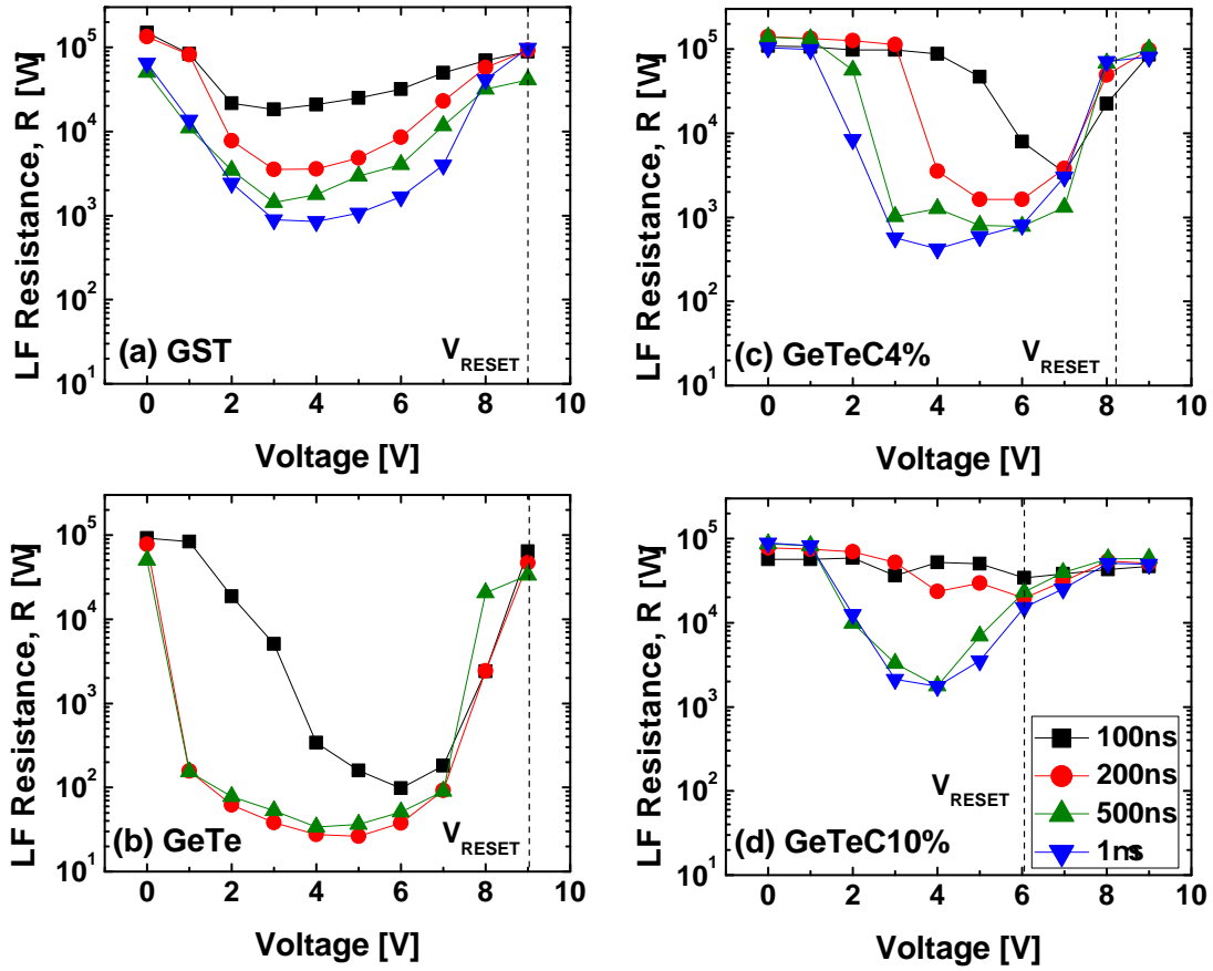
Figure 2.13: R-V characterization on PCM cells with (a) GST (b) GeTe, (c) GeTeC4% and (d) GeTeC10% materials. Different SET time pulse widths (100 ns, 200 ns, 500 ns, and 1 \mu s) have been applied to the cells and then LF resistance is read. Each SET pulse is preceded by a fixed RESET pulse (amplitude= 9V, width= 100ns, fall= 10ns). The voltage values V_{RESET} needed to obtain the RESET state are indicated by dash-type vertical lines for each R-V characteristics.
