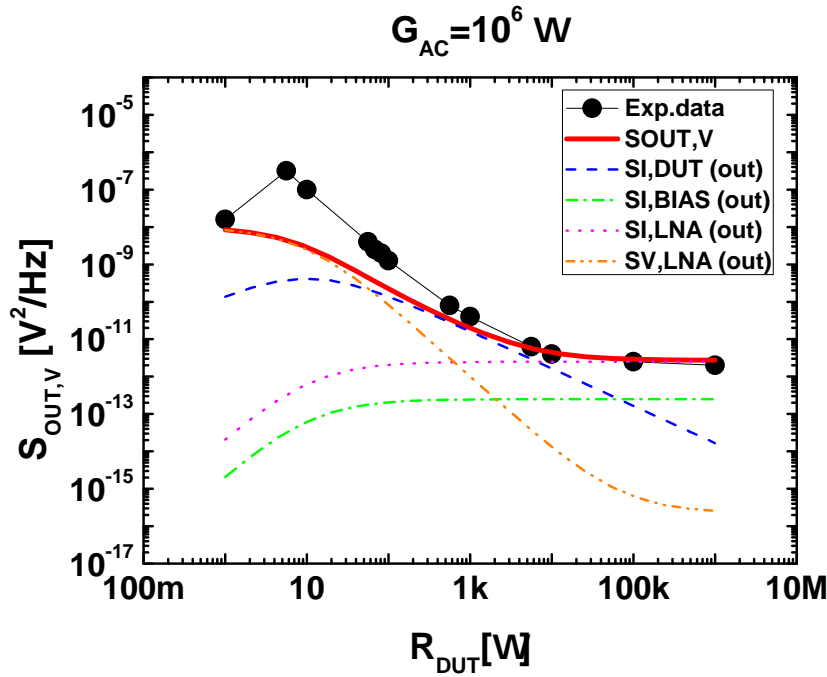
Figure 3.21: Lines: S_{OUT,V} , S_{I,DUT}(out) , S_{I,BIAS}(out) , S_{I,LNA}(out) and S_{V,LNA}(out) as a function of R_{DUT} , calculated using Eq.(3.33) and Eq.(3.35), for G_{AC} = 10^6\Omega . Dots refer to experimental S_{OUT,V} data.
