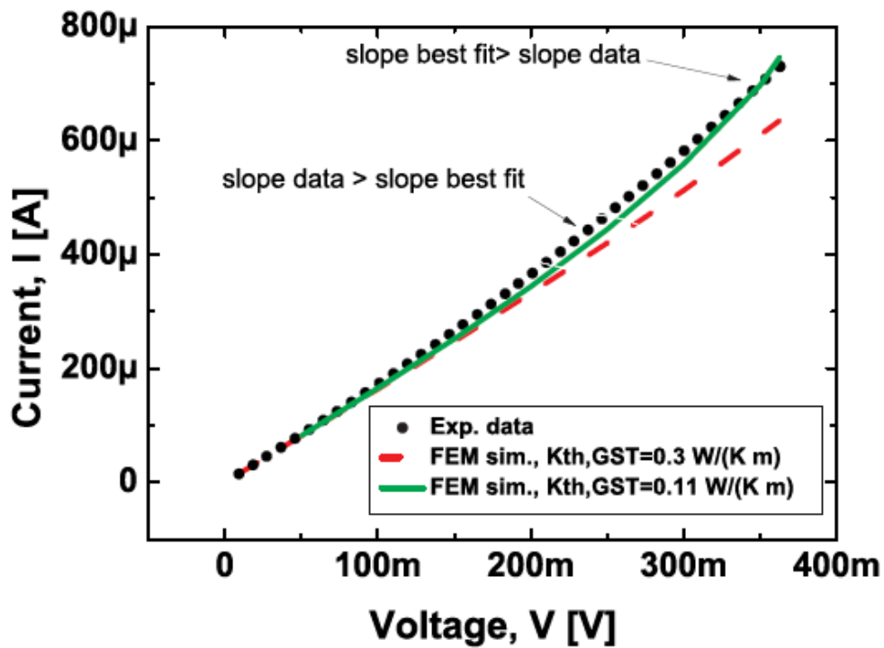
Figure 4.5: Electro-thermal FEM simulations of I - V curve with \kappa_{th,GST}=0.3 \text{ W}/(\text{m}\cdot\text{K}) (dash line, red), \kappa_{th,GST}=0.11 \text{ W}/(\text{m}\cdot\text{K}) (solid line, green), and experimental data (dots). Both data and simulations refer to T_{amb}=25^\circ\text{C} . The best fit curve ( \kappa_{th,GST}=0.11 \text{ W}/(\text{m}\cdot\text{K}) ) at "medium" V range ( 150\text{mV} < V < 300\text{mV} ) underestimates the slope of experimental data. The opposite happens at V > 350\text{mV} , where model increases quicker than data.
