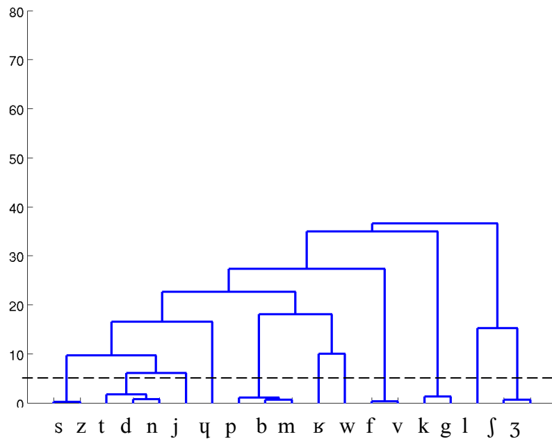
Figure 3.3-14. Confusion tree of articulatory parameters of consonants in EMA-PB-2009 corpus (the smaller ordinate, the more confused the two categories are). The dashed line corresponds to a threshold level of 5 that leads to eleven classes.
