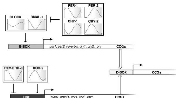
Fig. 2. Schematic representation of the ubiquituous transcription control of clock genes and clock-controlled genes through cyclic induction or inhibition of transcription by clock proteins, acting through specific promoters, E-boxes or ROR elements. Among the clock-controlled genes, other transcriptional factors, such as DBP, HLF, TEF or E4PB4, regulate the oscillatory transcription of clock-controlled genes through D-boxes. The curves show relative mRNA amount of main clock genes throughout the 24-h span. CGS: clock-controlled genes. Adapted from [30,68].
