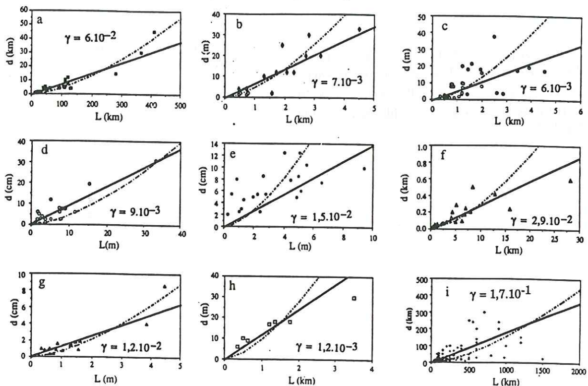
Fig. 1. Plots of maximum fault displacement vs fault length for nine different data sets: (a) Elliott (1976); (b) Krantz (1988); (c) Walsh & Watterson (1987); (d) Peacock & Sanderson (1991); (e) Peacock (1991); (f) Villemin et al. (in press); (g) Muraoka & Kamata (1983); (h) Opheim & Gudmundsson (1989); (i) MacMillan (1975).
