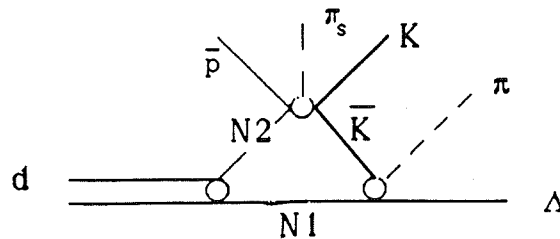
Figure 1.5: Rediffusion de \bar{K} de \bar{p}d \rightarrow \Lambda \bar{K} \pi ,
