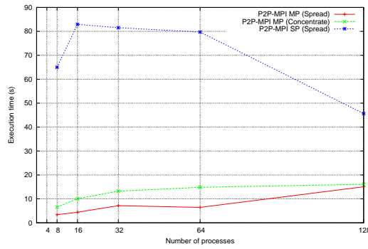
(b) lufact
