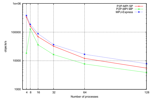
(h) gather-o-46340
