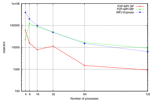
(g) gather-o-2048
