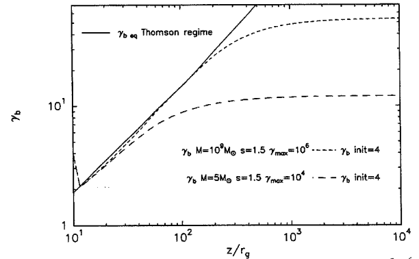
Figure 13. Solutions of the equation of motion for a supermassive black hole ( M = 10^9 M_\odot ) and a stellar black hole ( M = 5 M_\odot ) with a compact accretion disc. r_e = 10 r_g and L = L_{\text{Edd}} . \gamma_{\text{b,init}} is the initial condition of the solution. We also represent the equilibrium Lorentz factor in the Thomson regime.
