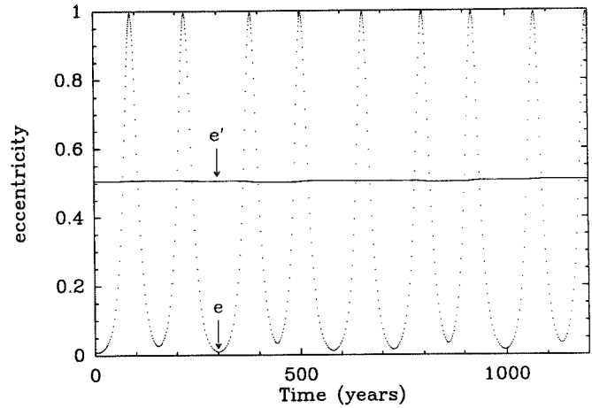
Fig. 3. Evolution of the eccentricities of the close binary ( e ) and the tertiary orbit ( e' ) as a function of time for 1200 years under the effects of pure 3-body dynamics. A quasi-periodic behavior (confirmed by integration over a longer time scale) is clearly detected; the close binary becomes very eccentric every \sim 150 years. Conversely, the eccentricity of the tertiary orbit is very stable. Only very small variations are recorded
