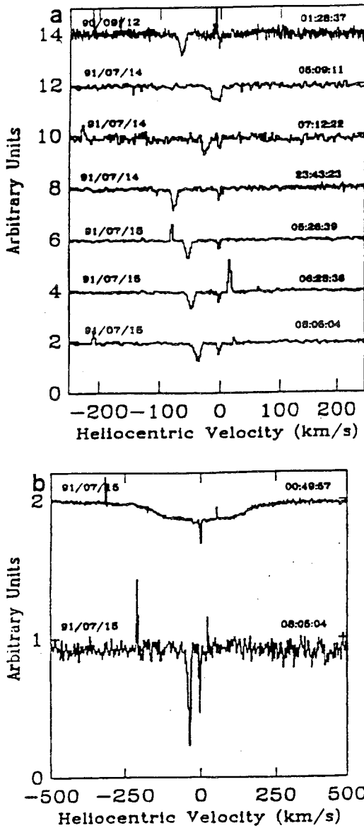
Fig. 2. a and b . High resolution spectra of the Ca II K line towards TY CrA. Same units as in Fig. 1. Two narrow absorption lines are observed in the spectrum of TY CrA, one stable in time, and the other variable in velocity. b Superposition of the Ca II line towards HD 176386 (top) and one of TY CrA (bottom). The narrow and stable component observed towards TY CrA is also present in the direction of HD 176386, which indicates an IS origin
