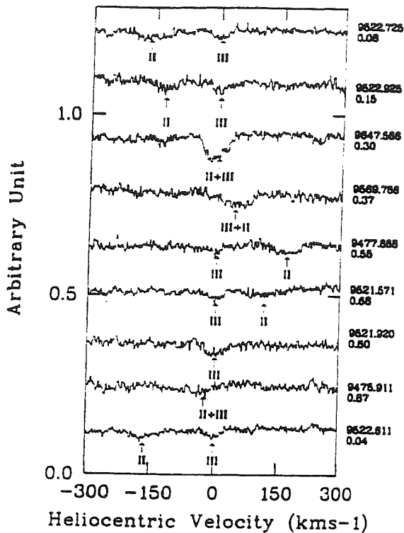
Fig. 1. High resolution spectra of Li I: the spectra are on an heliocentric velocity scale (not corrected for the binary center-of-mass motion). Arrows indicate the line of the secondary (II) and the tertiary (III); Julian Day and phase are given on the right side of the graph for each spectrum
