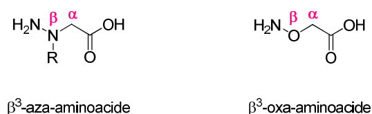
Figure 35 – Structures des \beta^3 -aza et \beta^3 -oxa-aminoacides
