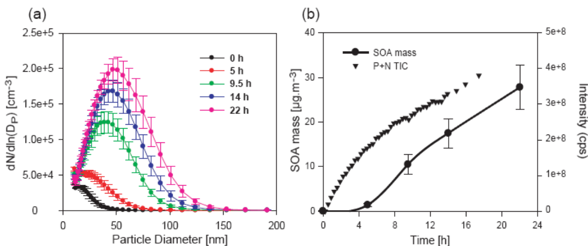
Figure 6. (a) Evolution of the particles size number distributions of the generated SOA as a function of reaction time during the aqueous phase OH-oxidation of methacrolein. SOA was generated using the experimental setup described in Figure 1. The particles number distributions of the generated SOA are an average of several distributions measured at the corresponding reaction times; the error bars represent the standard deviation of these averages. (b) Evolution of the SOA mass compared to the sum of the MS total ion current of the aqueous samples in the positive and the negative mode (P+N TIC) with the reaction time. The SOA mass are calculated using the SMPS data and assuming a particle density of 1 \text{ g}\cdot\text{cm}^{-3} .
