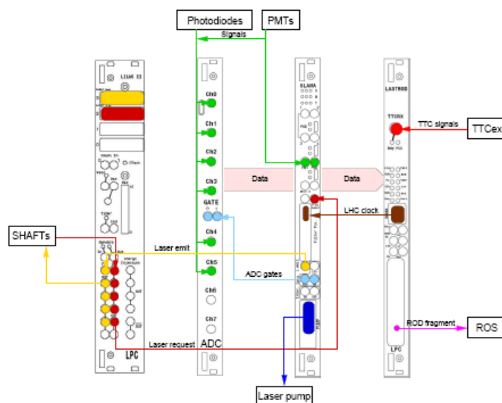
Figure 4.7: LASER system hardware involved in LASER mode. On the left is shown the SHAFT, on the center ADC and on the right the LASTROD.
