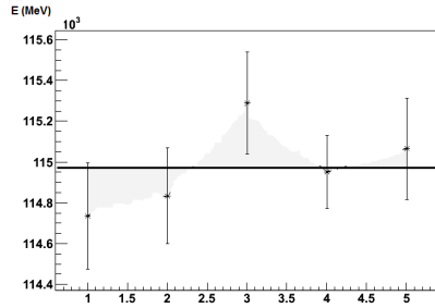
Figure 5.16: Distribution of energy values for different runs at 150 and eta 0.35. The result of the fit is quoted as E_{rec} .
