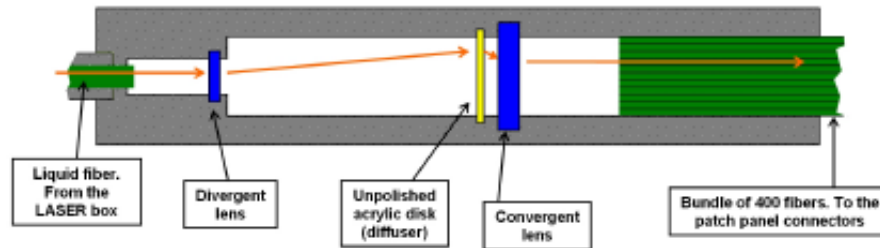
Figure 4.4: The Coimbra box.
