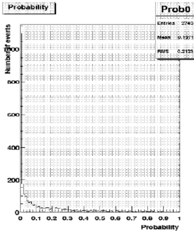
Figure 4.17: Hypothesis test: slopes distribution and chi-square probability distribution. The test is performed on the distribution of the ratio PMTtile/D1 versus the time.
