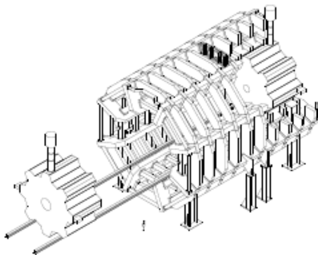
Figure 2.6: View of the superconducting air-core toroid magnet system
