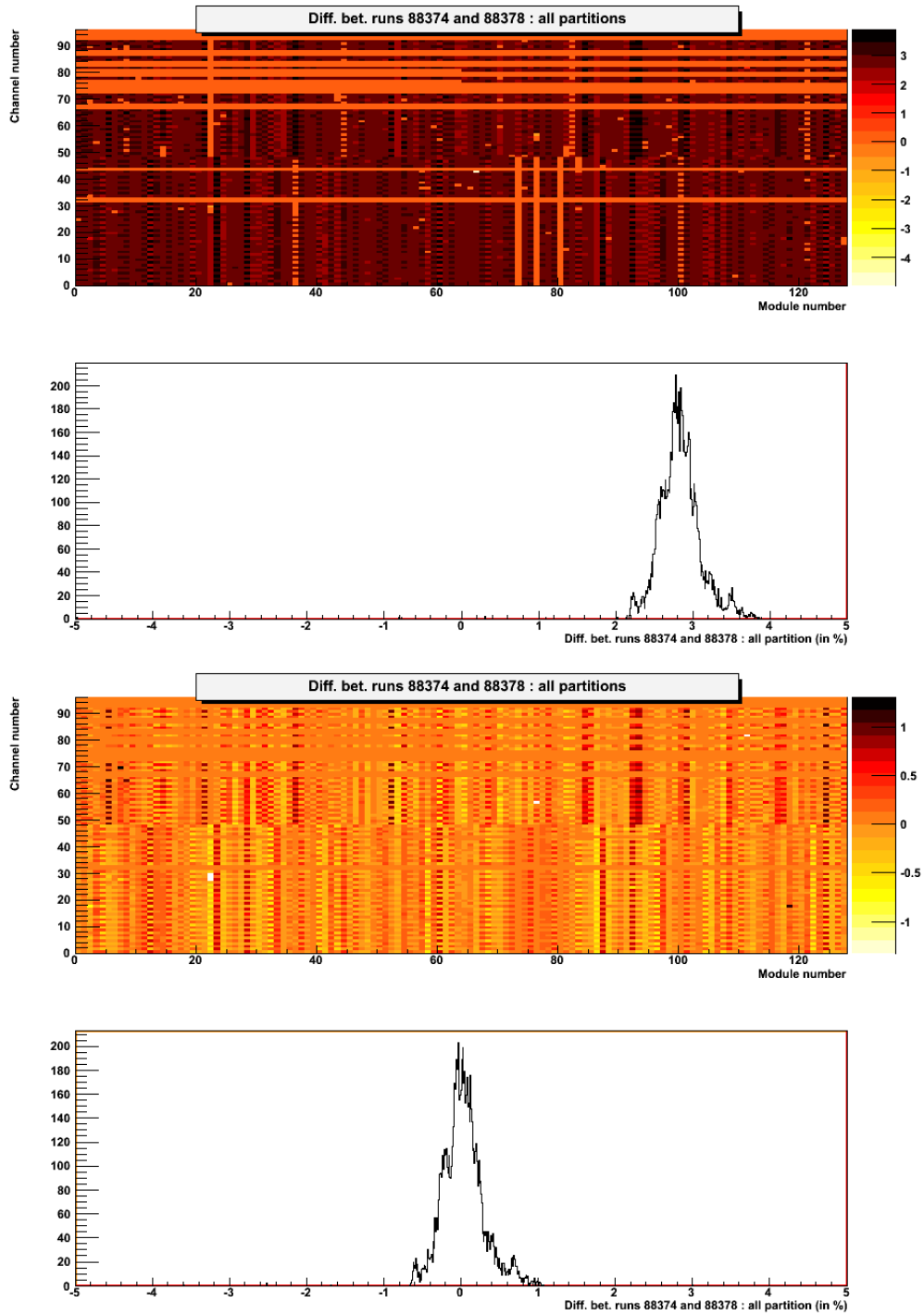
Figure 4.14: Evolution of the parameter \Delta_{n+1}^{filter} . In the top plot the shift due to the filter wheel is shown. In the bottom plot the result when this effect is removed. The two dimensional plots are a map the amount of light measured in a TileCal partition. On the x axis there is the module number and on y axis there is the photomultipolier number. The spread present here is related to miscalibration of the reference diode.
