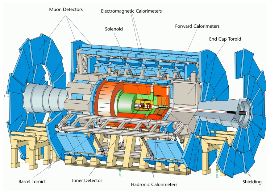
Figure 2.3: The ATLAS detector
