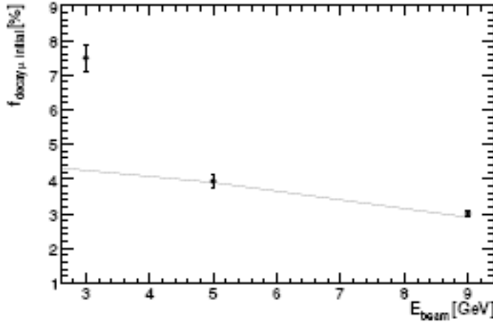
Figure 6.9: Fraction of the decay muons in the pion sample at the front of the calorimeter as a function of the beam momentum. The fraction f_{decay\mu initial} is defined as the number of muons triggering the DAQ divided by the number of pions. The full points show the result of the data-based analysis (method 1 in the text) and the solid curve represents the results obtained by the simulation (method 2 in the text).
