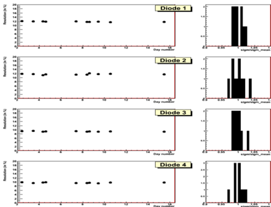
Figure 4.11: RMS/Mean stability distribution. On the left is shown the resolution as a function of the time, on the right is shown the resolution value measured w.r.t. resolution for the considered diode.
