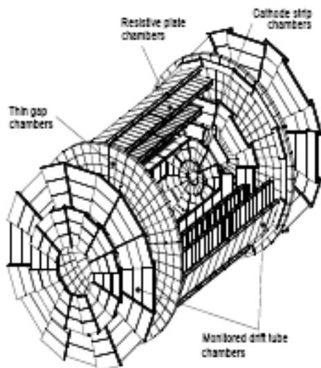
Figure 2.10: The ATLAS muon spectrometer
