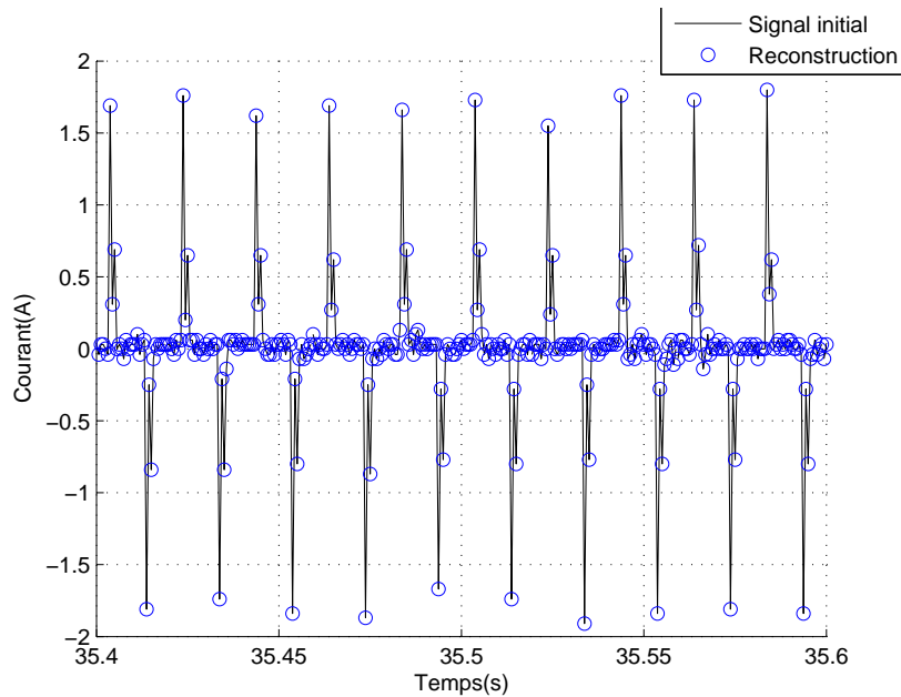
FIGURE 5.18 – Courant reconstruit
