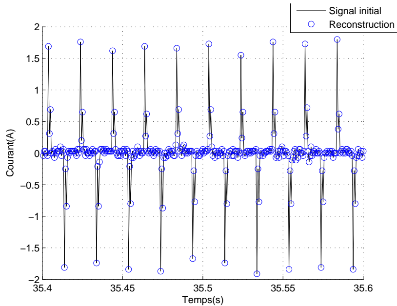
FIGURE 5.18 – Courant reconstruit
