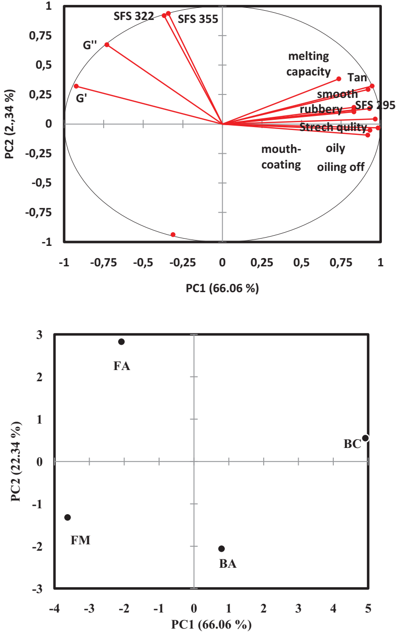
Figure 6: Principal component analysis biplot of sensory and instrumental parameters used to differentiate Fourme d’Ambert (FA), Fourme de Montbrison (FM), Bleu d’Auvergne (BA) and Bleu des Causses (BC) cheeses.
