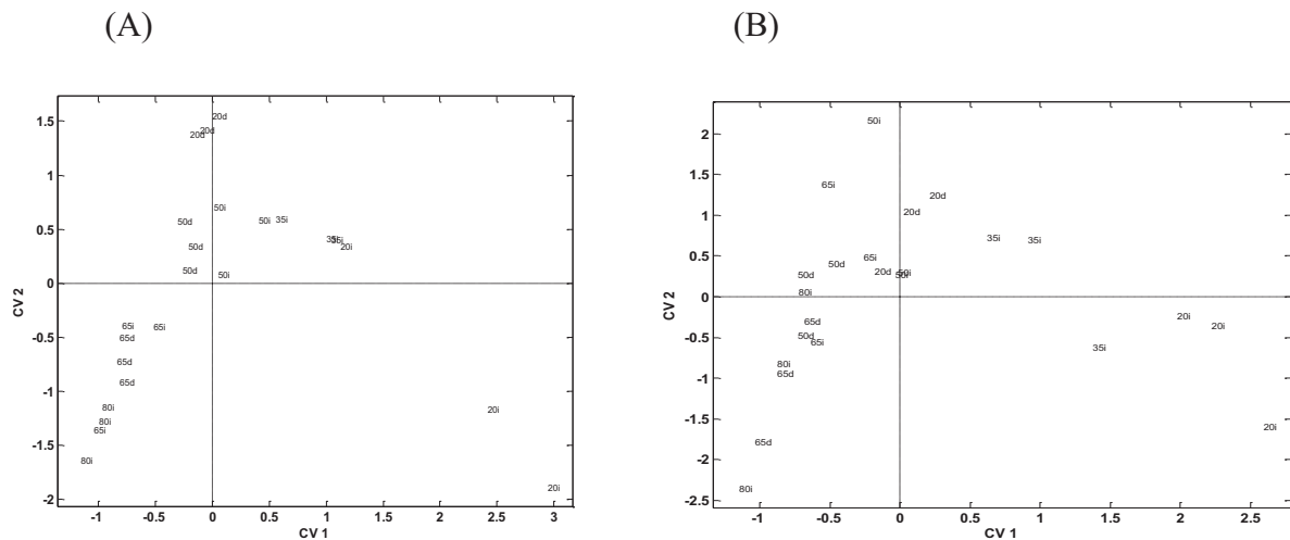
Figure 6. Canonical correlation analysis of the synchronous fluorescence spectral data and the rheology data during heating and cooling. (A) Similarity map defined by the canonical variates 1 and 2 of the CCA for the rheology data. (B) Similarity map defined by the canonical variates 1 and 2 for the synchronous fluorescence data.
