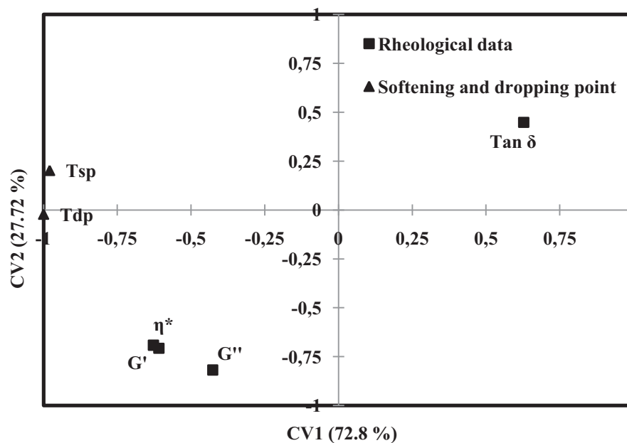
Figure 8: Similarity map of CCA applied to the rheological and the meltability data sets of Blue veined cheeses.
