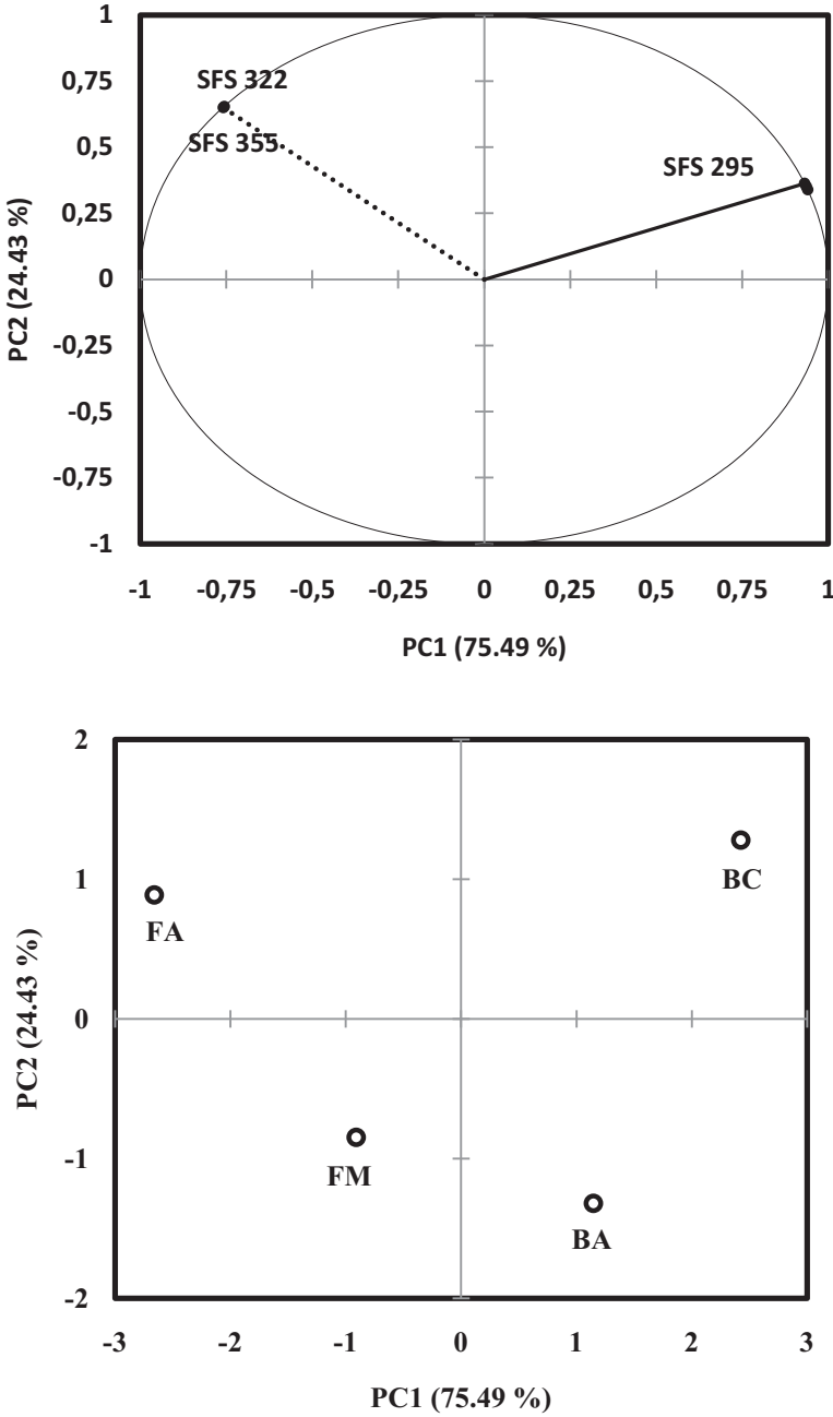
Figure 4: Principal component analysis map of the spectral data used to differentiate heated Fourme d’Ambert (FA), Fourme de Montbrison (FM), Bleu d’Auvergne (BA) and Bleu des Causses (BC) cheeses.
