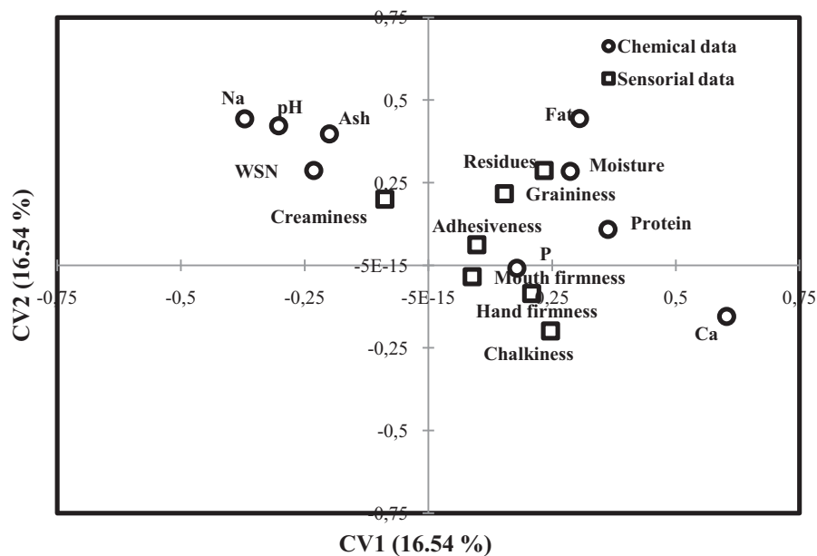
Figure 6: Similarity map of CCA applied to the physico-chemical data and the sensory texture data sets of Blue veined cheeses.
