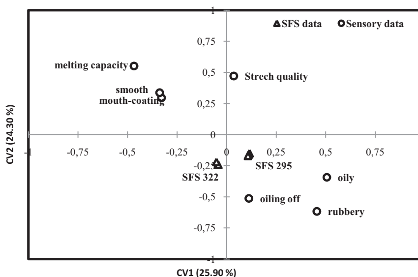
Figure 8: Similarity map of CCA applied to the fluorescence data and the sensory data sets of blue-veined cheeses.
