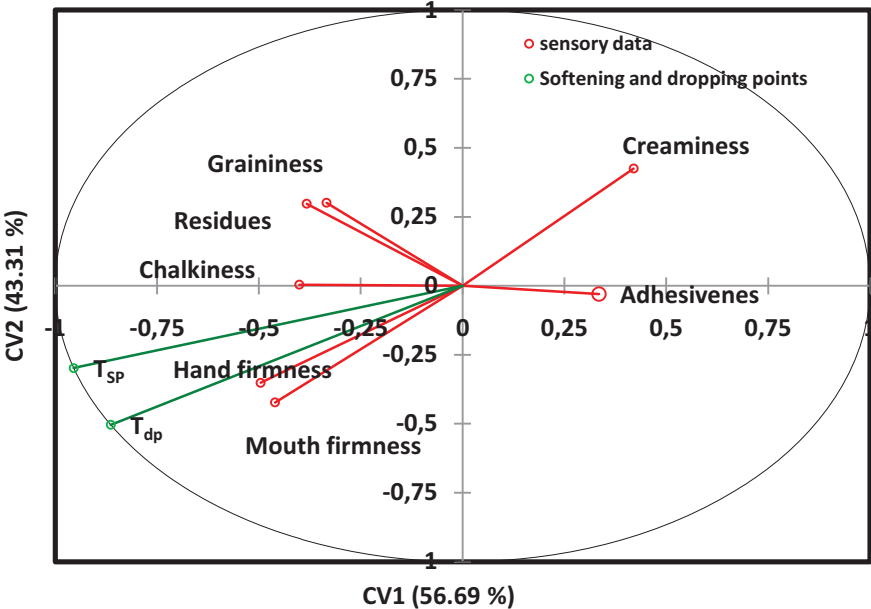
Figure 9: Similarity map of CCA applied to the sensorial and the meltability data sets of Blue veined cheeses.
