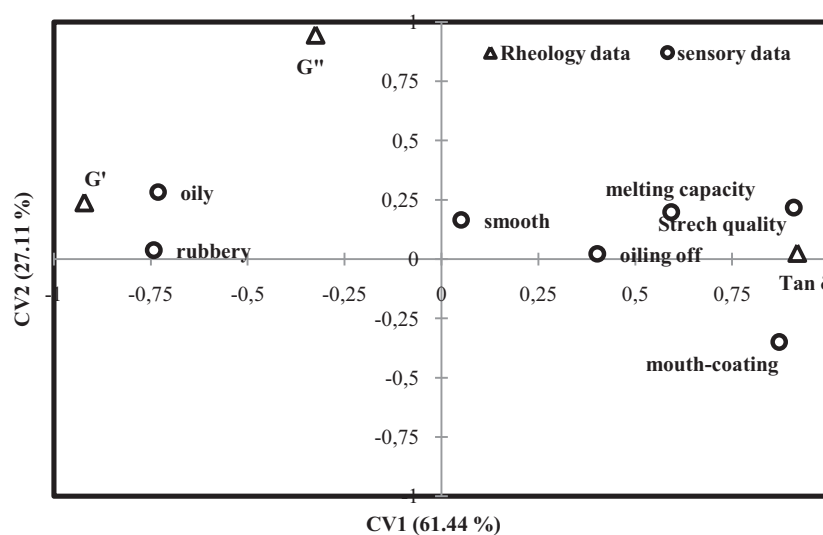
Figure 7: Similarity map of CCA applied to the rheology data and the sensory data sets of Blue veined cheeses.
