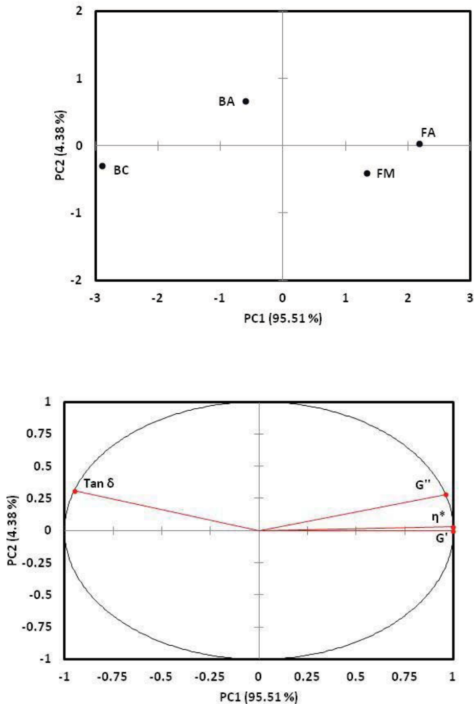
Figure 2: PC 1 and PC 2 similarity map determined by principal components 1 (95.51%) and 2 (4.38%) and correlation circle associated obtained after principal components analysis of rheological attributes ( G' , G'' , \tan \delta , and \eta^* ) measured on Blue-veined cheeses (FA: Fourme d'Ambert, FM: Fourme de Montbrison, BA: Bleu d'Auvergne; BC: Bleu des Causses).
