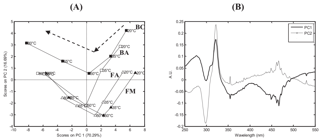
Figure 4. PC1 and PC2 Similarity maps (A) and associated spectral loadings (B) obtained after PCA of SF spectra recorded during heating (from 20 to 80°C) for the different blue cheeses obtained from pasteurized milk (FA: Fourme d’Ambert , FM: Fourme de Montbrison , BA: Bleu d’Auvergne ; BC: Bleu des Causses )
