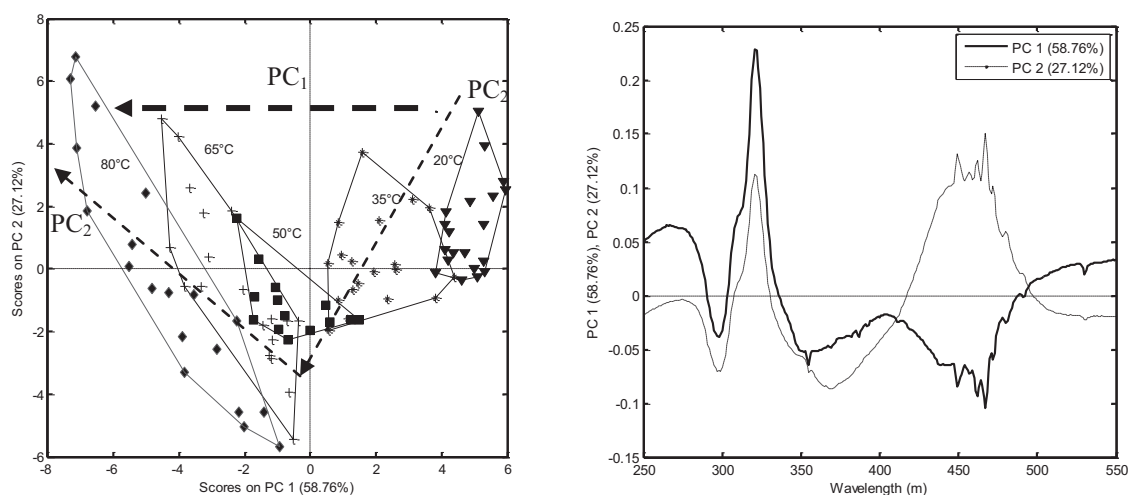
Figure 7. PC1 and PC2 Similarity maps and associated spectral loadings obtained after PCA of SF spectra recorded during heating (from 20 to 80°C) for the Fourme de Montbrison cheese
