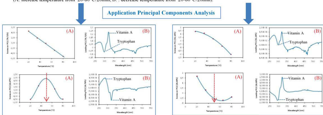
Fig.2.A: Evaluation of sample scores of Bleu d'Auvergne cheese as a function of temperature according to PC 1 and PC 2 B: Evaluation of loading spectra of Bleu d'Auvergne cheese as a function of temperature according to PC 1 and PC 2
