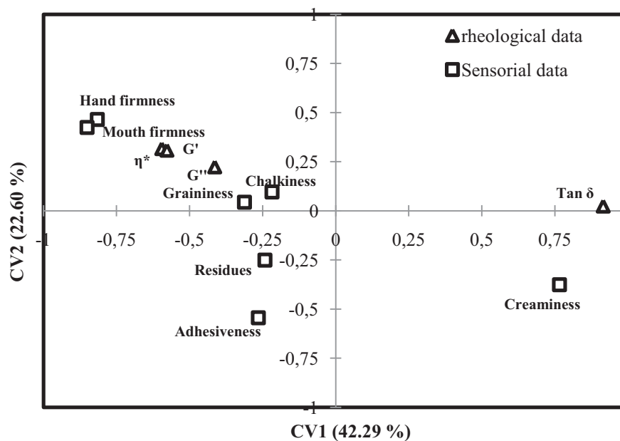
Figure 7: Similarity map of CCA applied to the rheological data and the sensory texture data sets of Blue veined cheeses.
