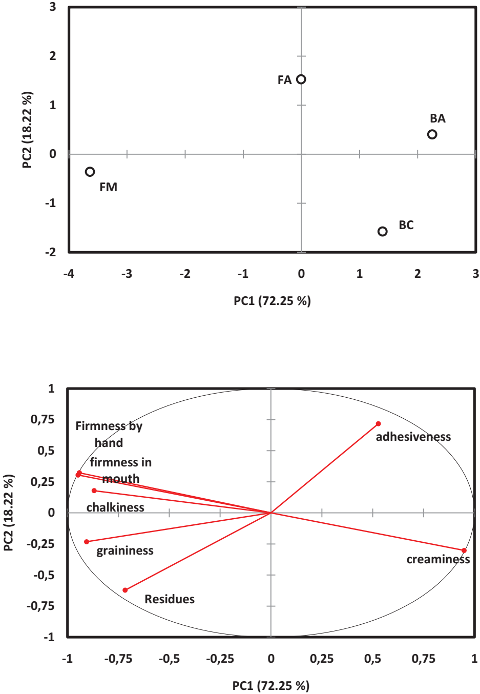
Figure 3: Principal components plot of sensory texture attributes used to differentiate of four Blue-veined cheeses (FA: Fourme d’Ambert, FM: Fourme de Montbrison, BA: Bleu d’Auvergne; BC: Bleu des Causses).
