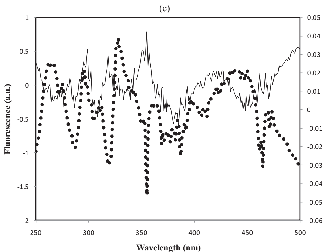
Fig. 4 (suite) Regression coefficient distribution over the 250-500 nm spectra of Partial least squares regression models of (a) Ash, (b) Fat, and (c) protein for Fourme cheeses (--) and Bleu cheeses classes (•••).
