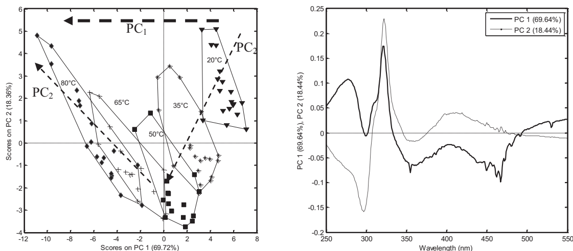
Figure 8. PC1 and PC2 Similarity maps and associated spectral loadings obtained after PCA of SF spectra recorded during heating (from 20 to 80°C) for the Bleu d'Auvergne cheese
