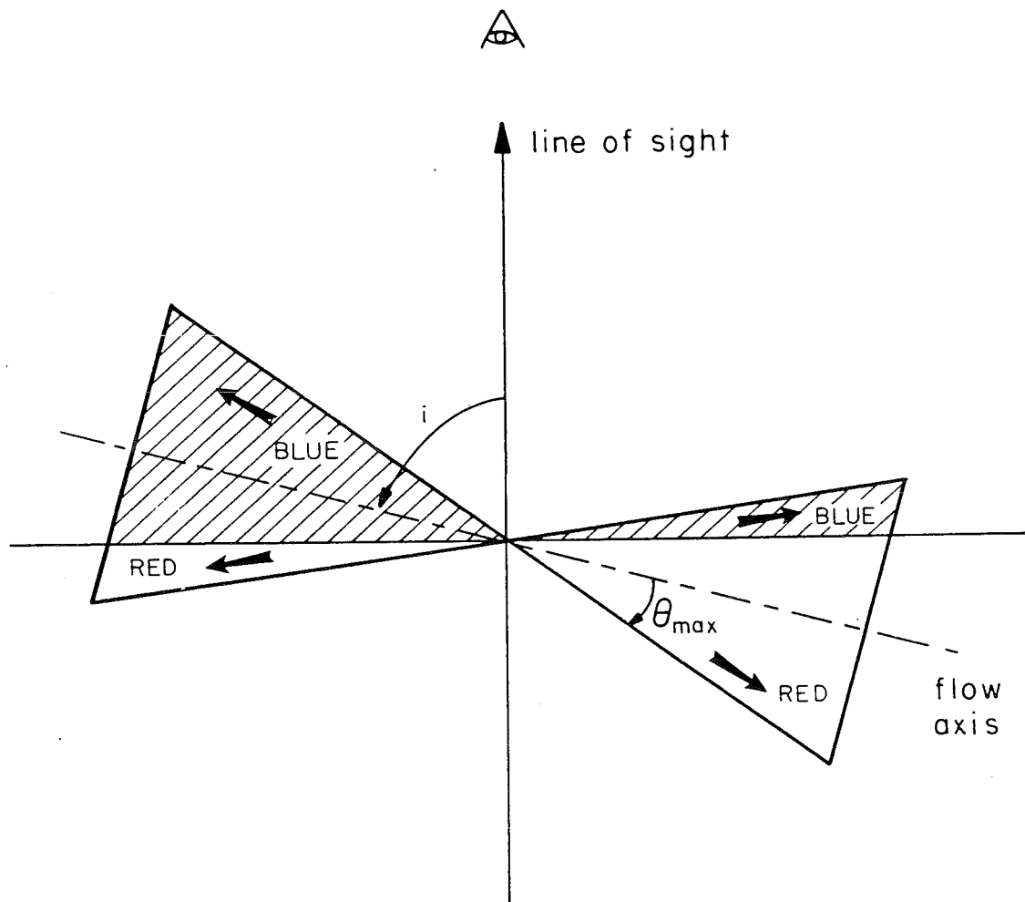
FIG. 1.—This diagram illustrates the geometry of the “face-on” configuration studied in this paper, here for a biconical outflow with radial expansion. The velocity vectors (arrows) are making a maximum angle \theta_{\max} with the flow axis. The view angle i between the line of sight and the flow axis is greater than 90^\circ - \theta_{\max} , so that material in the front part of the lobes (shaded areas) is approaching us, while material in the back part of the lobes is receding from us. The observer therefore sees redshifted emission in the blue lobe and blueshifted emission in the red lobe.
