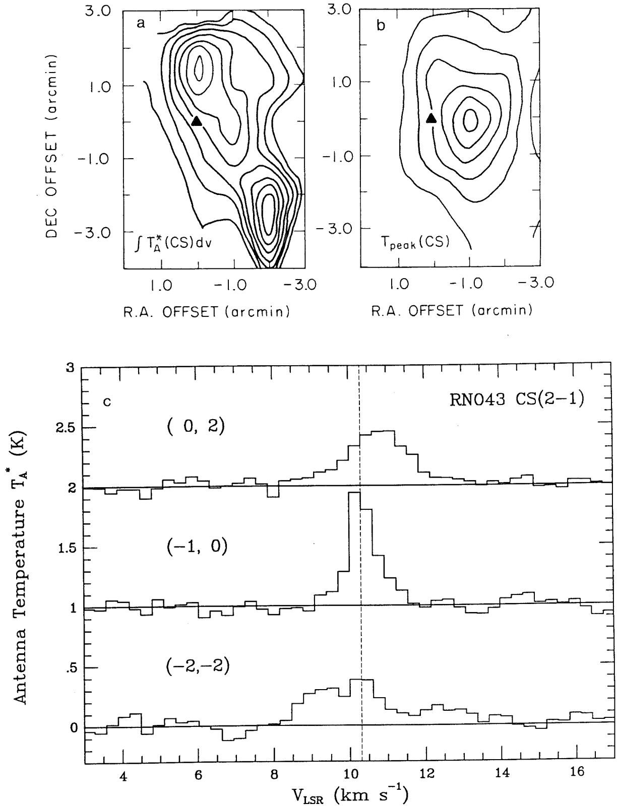
FIG. 5a–b.—Maps of the CS J=2 \rightarrow 1 total integrated intensity (left) and maximum antenna temperature (right) near the far-infrared source driving the RNO 43 outflow. The IRAS position of the source is shown as a filled triangle. The contour levels start at 0.3 \text{ K km s}^{-1} in Fig. 5a and 0.2 \text{ K} in Fig. 5b and are spaced by 0.1 \text{ K km s}^{-1} in Fig. 5a and by 0.1 \text{ K} in Fig. 5b. (c)—CS J=2 \rightarrow 1 spectra obtained at three different positions along the flow axis: in the blue lobe (top), toward the peak of the CS emission (middle), and in the red lobe (bottom). The velocity resolution is 0.31 \text{ km s}^{-1} . The dashed line indicates the cloud systemic velocity. Note the extended blueshifted and redshifted wings in the top and bottom spectra.
