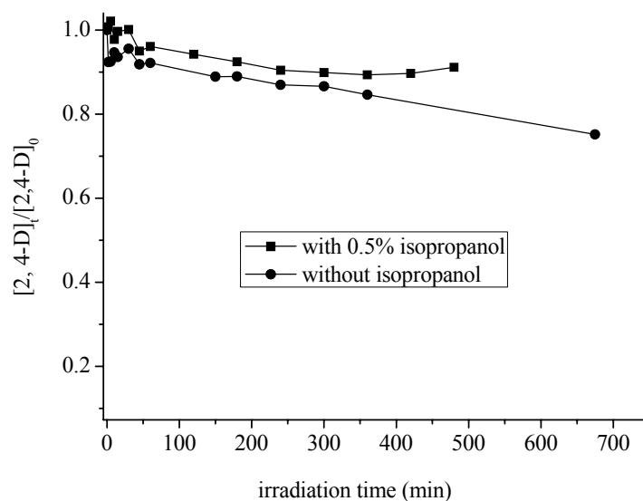
Figure V-B-7 Influence of isopropanol on the photodegradation of 2, 4-D in suspension of goethite at pH 4.0 ( [\text{goethite}] = 0.2 \text{ g L}^{-1} , [2, 4\text{-D}]_0 = 0.1 \text{ mmol L}^{-1} )
