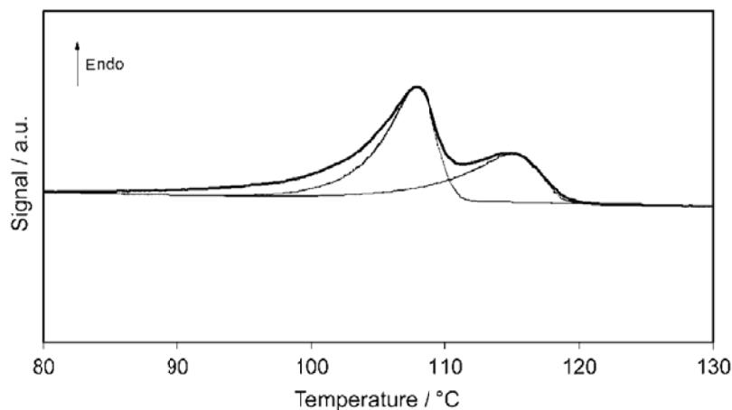
Fig. 9 Deconvolution of the DSC curve obtained by PEAK-FIT V4 [105]
