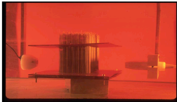
Linear array, 128 transducers Element size \frac{3}{8}\lambda
