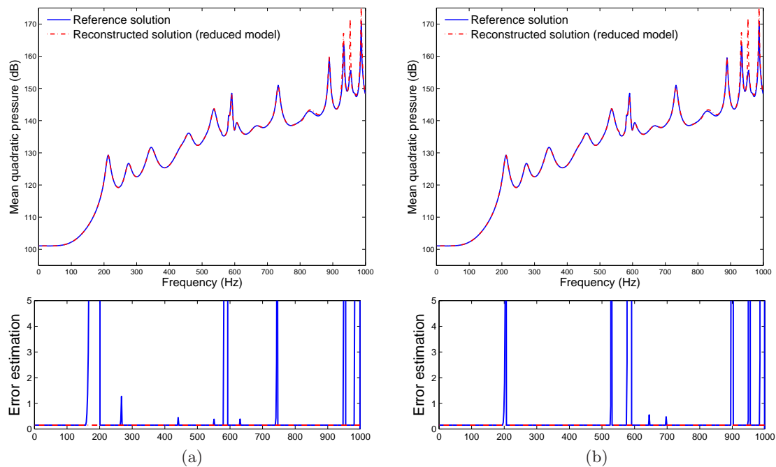
Figure 5.10: Adaptive reconstructed solution for 3D problem from optimized reduced problem: (a) L = 3 , M = 4 ; (b) L = 5 , M = 6 .
