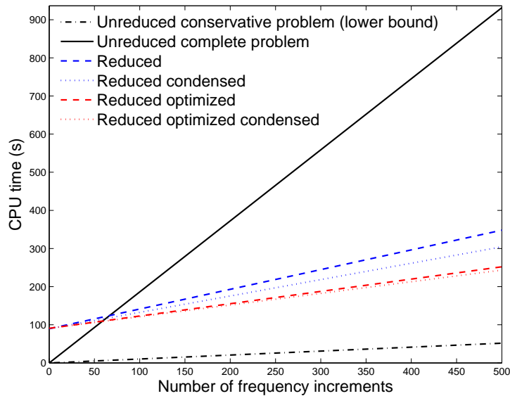
Figure 4.15: Computation time comparison for 3D problem - \chi_{\max} = 0.4
