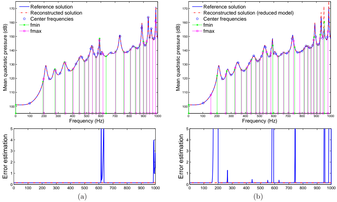
Figure 5.8: Adaptive reconstruction procedure applied to 3D problem with L = 3 , M = 4 : (a) from non-reduced problem; (b) from optimized reduced problem.
