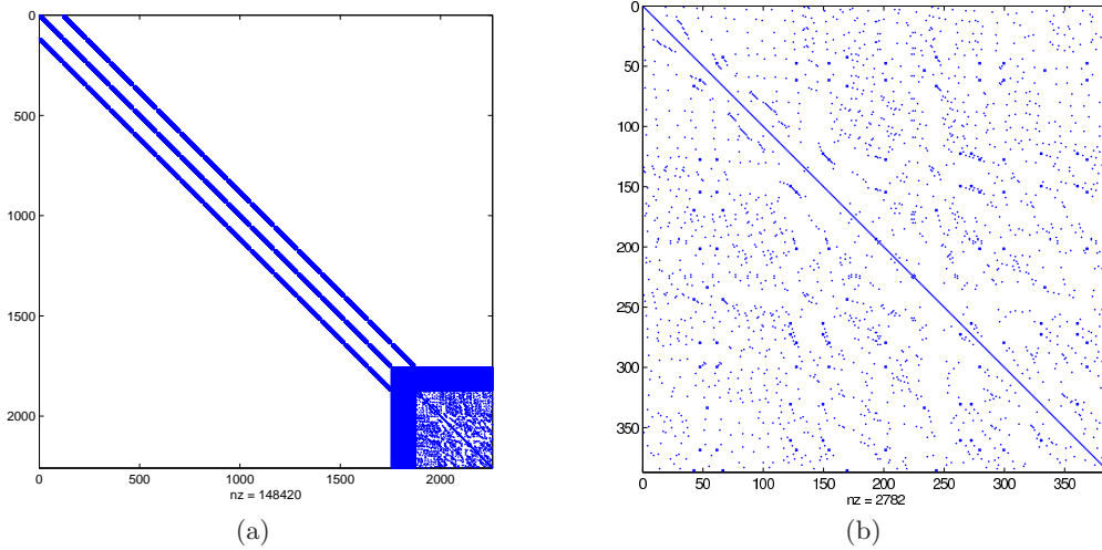
Figure 3.16: (a) Sparsity of system matrix for reduced poroelastic domain with condensed “orthogonal” modal unknowns and (b) focus on the sparsity for the “non-orthogonal” modal unknowns
