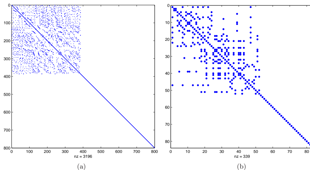
Figure 4.17: Detailed sparsity corresponding to the modal dofs, before and after mode selection procedure: (a) 800 modes, (b) 83 modes
