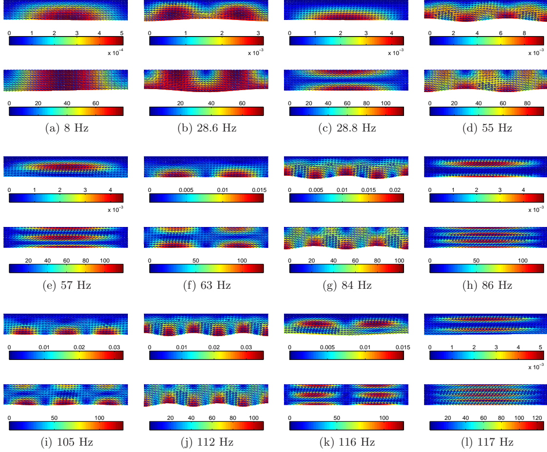
Figure 4.13: Porous 2D mode shapes: solid (top) and fluid (bottom) phases. Deformed mesh and norm of displacement.
