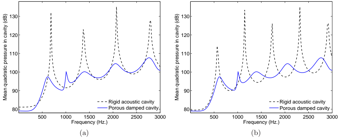
Figure 3.4: Mean quadratic pressure reference FRF, 1D problem, with for rigid cavity: (a) poroelastic volume not replaced by acoustic volume; (b) poroelastic volume replaced by acoustic volume.
