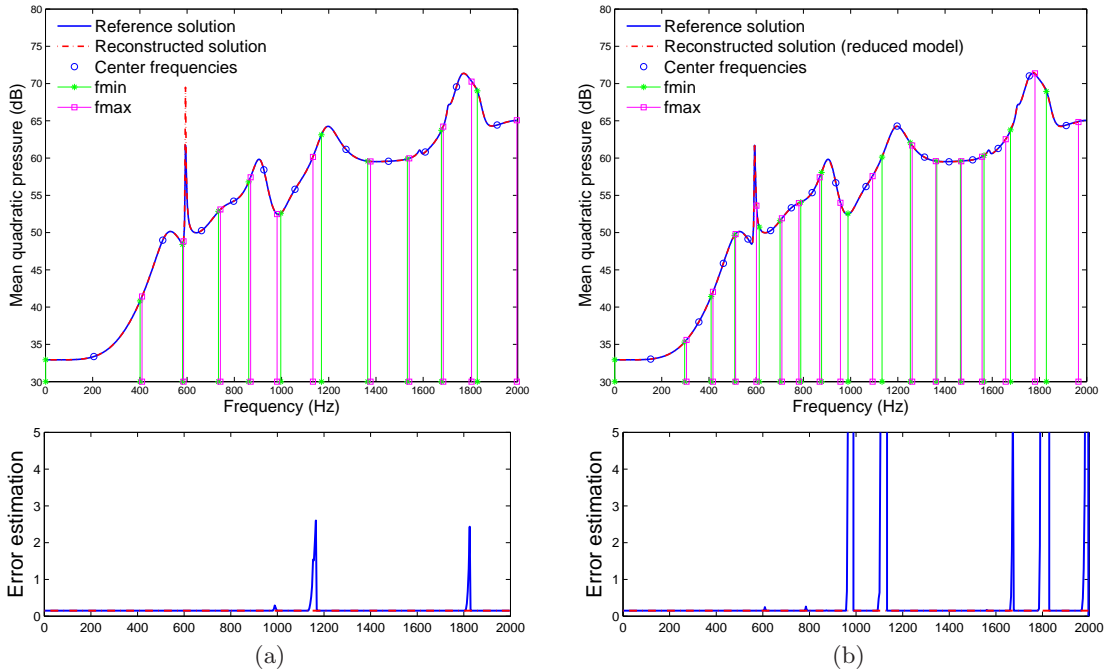
Figure 5.5: Adaptive reconstruction procedure applied to 2D problem: (a) from non-reduced problem; (b) from optimized reduced problem.
