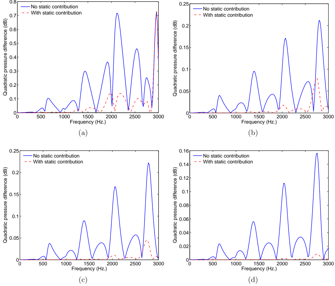
Figure 3.10: Error to reference solution (dB difference) with and without orthogonalized static response, including (a) 3 modes, (b) 4 modes, (c) 5 modes, (d) 6 modes
