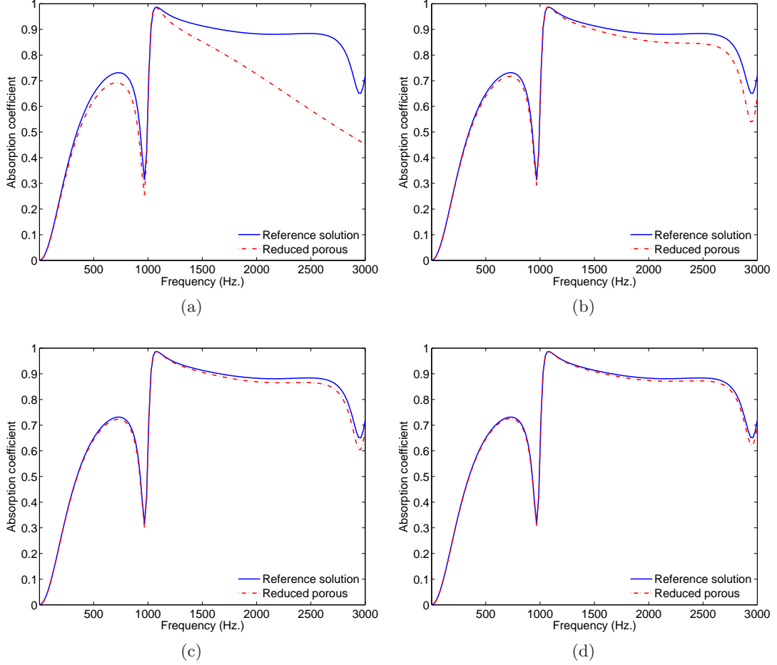
Figure 3.9: Absorption coefficient; Convergence of the reduced model to the reference solution with added modes in the basis: (a) 2 modes, (b) 4 modes, (c) 6 modes, (d) 8 modes
