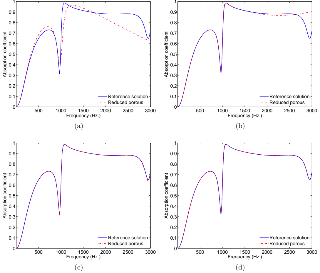
Figure 3.11: Absorption coefficient; Convergence of the reduced model to the reference solution with added modes in the basis and a low frequency correction vector: (a) 1 mode, (b) 2 modes, (c) 4 modes, (d) 6 modes
