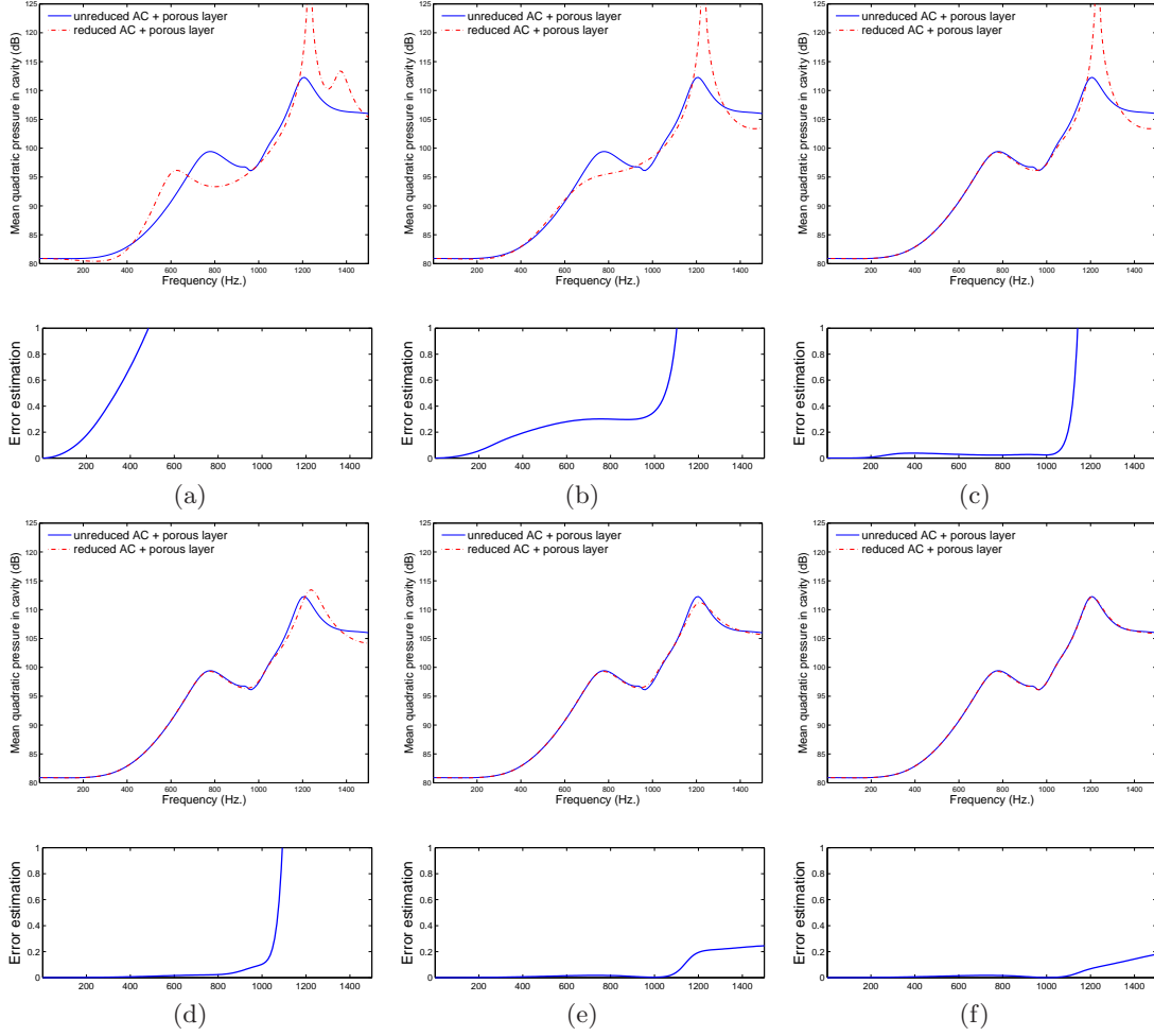
Figure 4.8: Convergence with modal superposition of selected modes for \chi_{\max} = 0.4 : (a) Mode 1, (b) Modes 1, 2, 21; (c) Modes 1, 2, 21, 15; (d) Modes 1, 2, 21, 15, 4; (e) Modes 1, 2, 21, 15, 4, 12, 26; (f) Modes 1, 2, 21, 15, 4, 12, 26, 16
