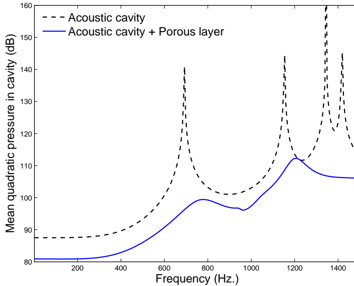
Figure 4.2: Mean quadratic pressure in the acoustic domain
