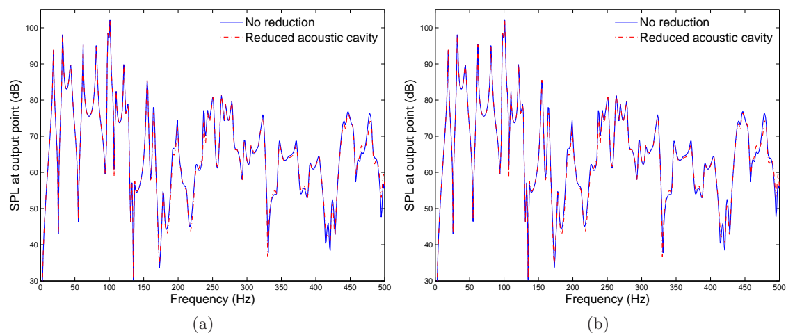
Figure 6.5: Sound pressure level at output point: dynamic condensation of acoustic domain, (a) modal truncation at 1060 Hz; (b) modal truncation at 1250 Hz.
