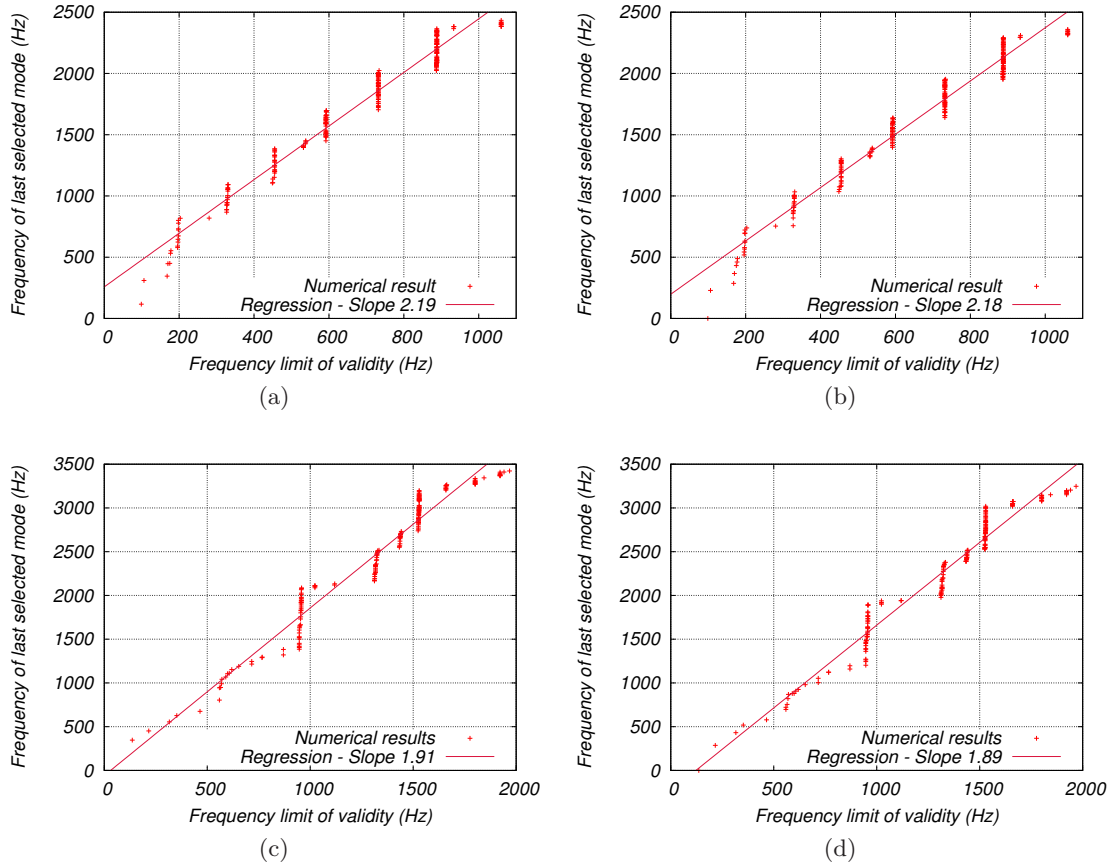
Figure 2.16: Effect of boundary conditions on truncation criterion, error tolerance of 0.1 dB: (a) Restrained-interface eigenfrequencies for largest cavity, (b) Free-interface eigenfrequencies for largest cavity, (c) Restrained-interface eigenfrequencies for smallest cavity, (d) Free-interface eigenfrequencies for smallest cavity
