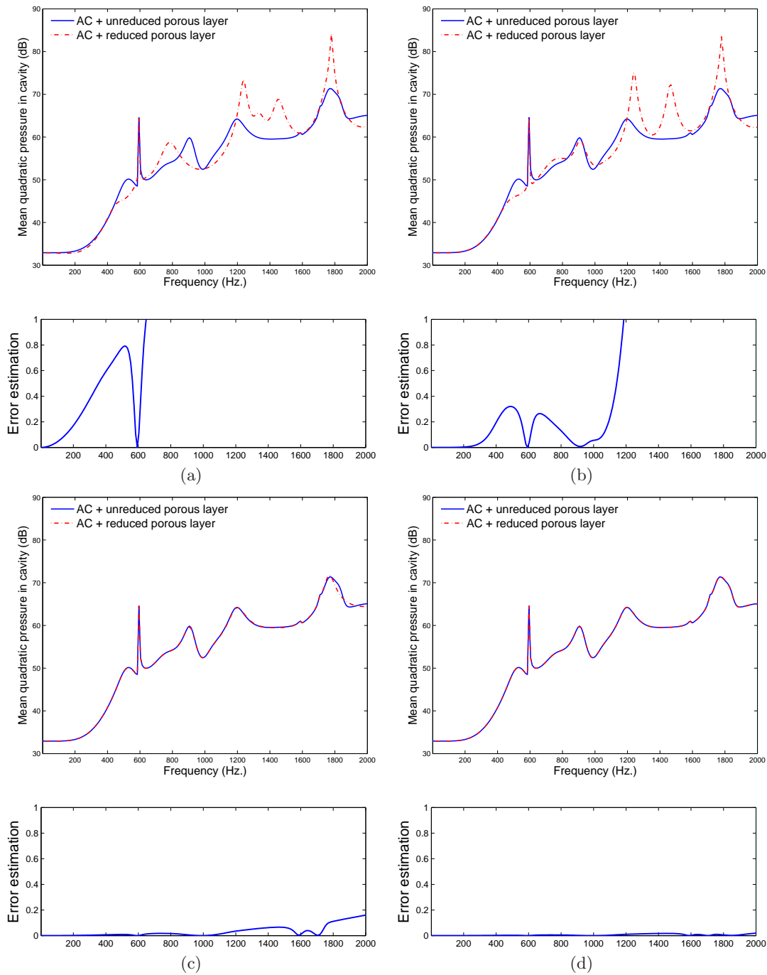
Figure 4.11: Solution convergence for the reduced model: (a) 90 modes, (b) 130 modes; (c) 180 modes; (d) 355 modes
