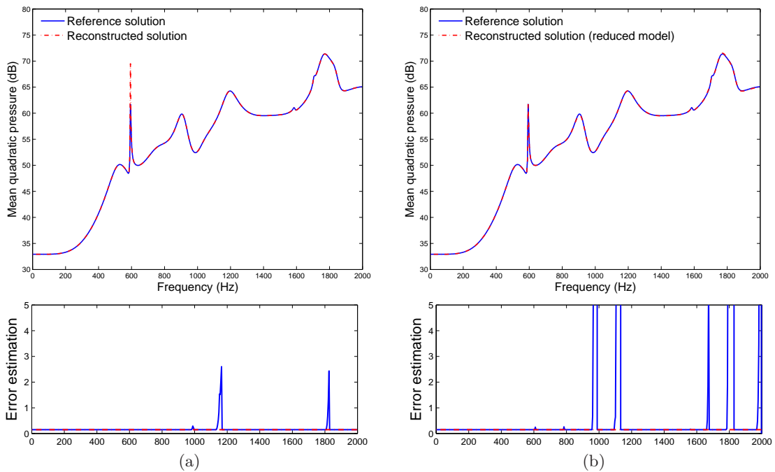
Figure 5.6: Adaptive reconstructed solution for 2D problem: (a) from non-reduced problem; (b) from optimized reduced problem.
