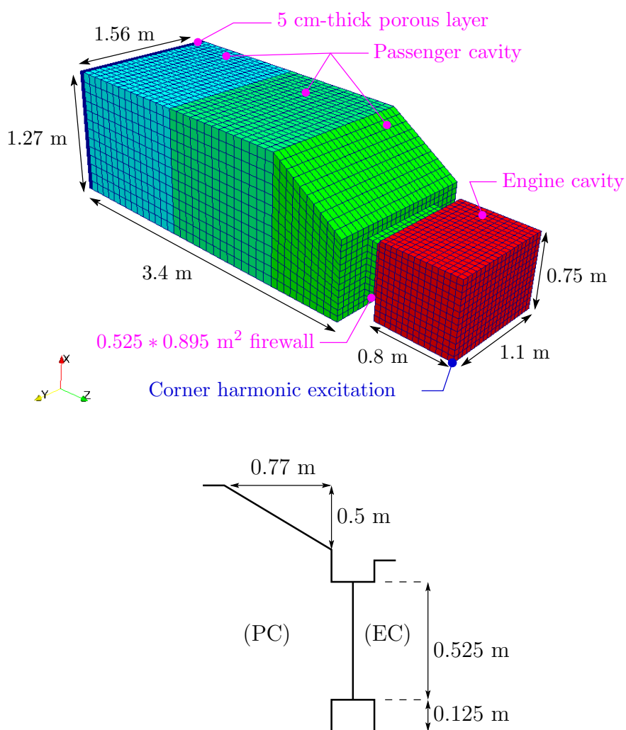
Figure 2.17: Concrete car FE model and external dimensions.
