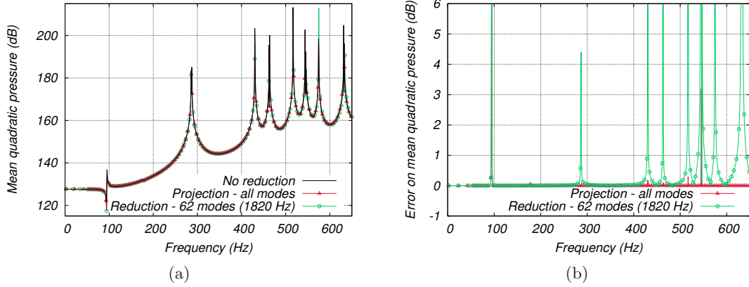
Figure 2.6: Convergence of reduction in excited cavity: (a) Mean quadratic pressure in dB versus frequency (b) dB difference to unreduced problem
