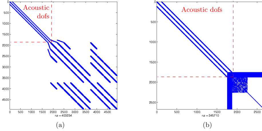
Figure 3.15: Sparsity of system matrix for (a) unreduced and (b) reduced poroelastic domain
