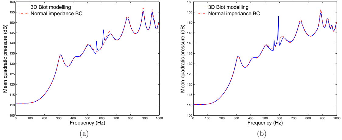
Figure 1.3: Comparison of the mean quadratic pressure in the cavity using a 3D model or normal impedance boundary condition, Lz_p = 0.05 m: (a) (Lx_a, Ly_a, Lz_a) = (0.28, 0.4, 0.5) m; (b) (Lx_a, Ly_a, Lz_a) = (0.3, 0.4, 0.5) m.
