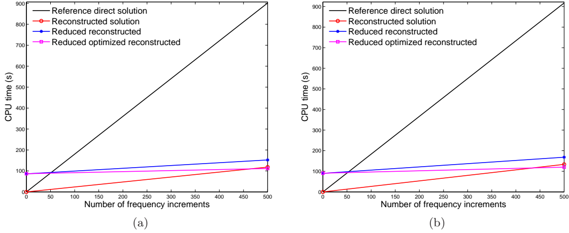
Figure 5.11: CPU time comparison for reconstructed solution from non-reduced, reduced, and optimized reduced 3D problems: (a) L = 3, M = 4 ; (b) L = 5, M = 6 .
