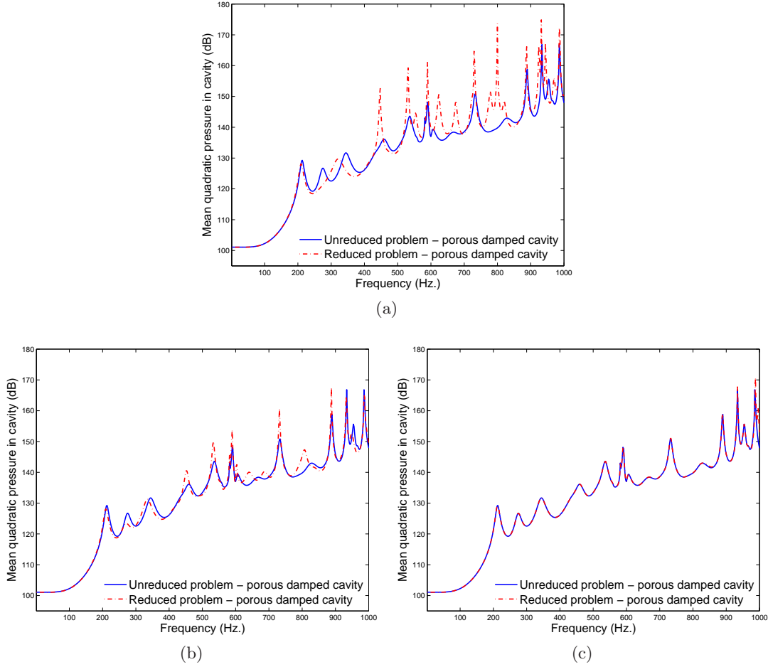
Figure 3.14: Mean quadratic pressure FRF. Convergence of the reduced model to the reference solution with added modes in the basis: (a) 100 modes, (b) 500 modes, (c) 800 modes.
