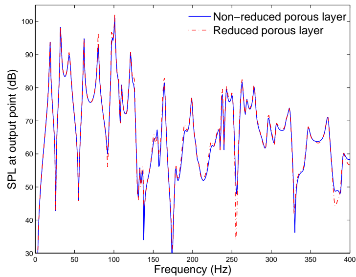
Figure 6.9: Modal reduction of porous domain, modal truncation at 800 Hz.
