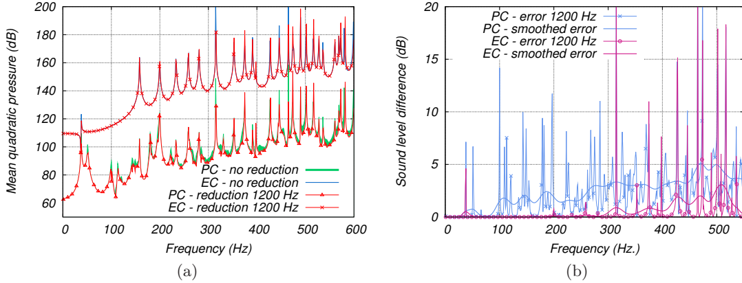
Figure 2.21: Results with truncation at 1200 Hz: (a) FRF of mean quadratic pressure (b) dB difference to unreduced problem
