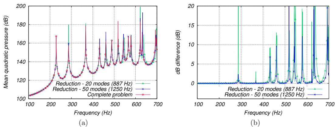
Figure 2.11: Decomposition into two subdomains of the conservative problem: (a) FRF with 20 and 50 modes per component, (b) dB difference to unreduced problem
