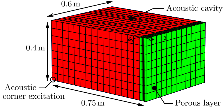
Figure 2.8: Acoustic cavity mesh and dimensions
