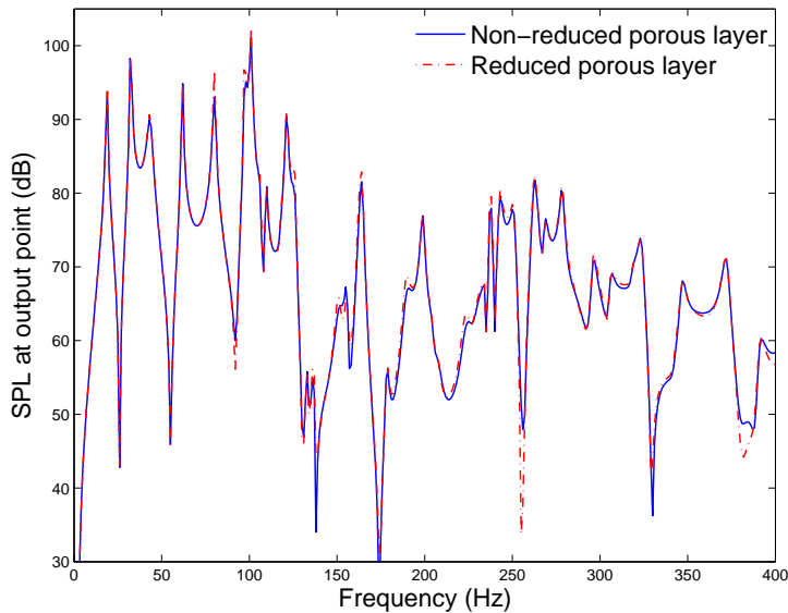
Figure 6.10: Sound pressure level at output point: modal reduction of porous domain, truncation at 400 Hz.
