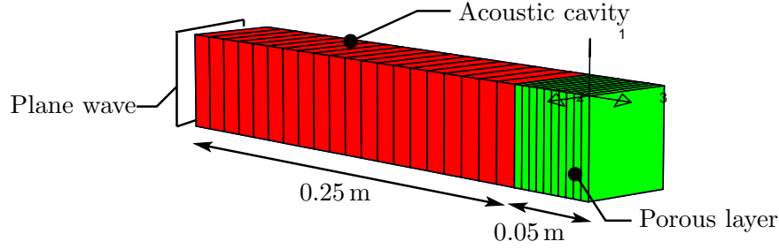
Figure 3.3: Acoustic cavity mesh and dimensions for 1D problem
