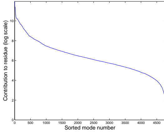
Figure 6.12: Normalized mode participations to the real part of the first residual response (100 Hz), logarithmic scale.
