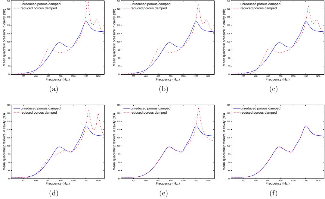
Figure 4.5: Convergence with modal superposition of manually selected modes: (a) Mode 1, (b) Modes 1, 2; (c) Modes 1, 2, 4, 12; (d) Modes 1, 2, 4, 12, 15; (e) Modes 1, 2, 4, 12, 15, 16, 21; (f) Modes 1, 2, 4, 12, 15, 16, 21, 26
