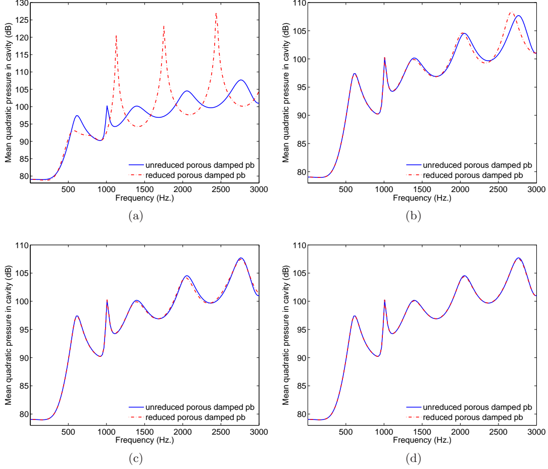
Figure 3.8: Mean quadratic pressure FRF; Convergence of the reduced model to the reference solution with added modes in the basis: (a) 1 mode, (b) 2 modes, (c) 3 modes, (d) 4 modes
