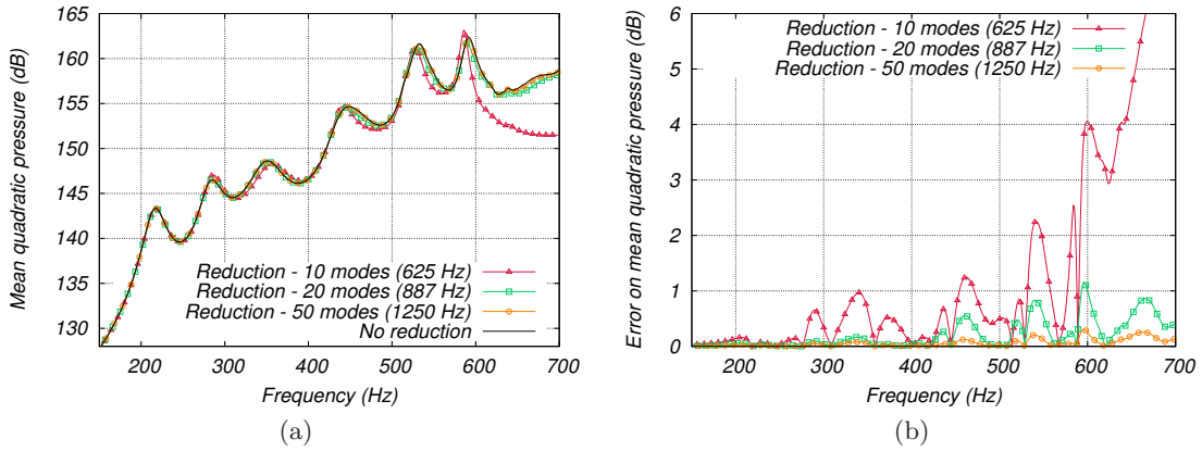
Figure 2.12: Reduction of the acoustic component to its interface with porous: (a) FRF with 10, 20 and 50 modes, (b) dB difference to unreduced problem
