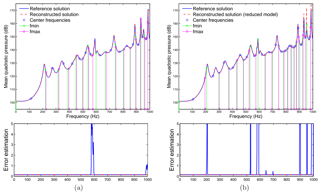
Figure 5.9: Adaptive reconstruction procedure applied to 3D problem with L = 5 , M = 6 : (a) from non-reduced problem; (b) from optimized reduced problem.
