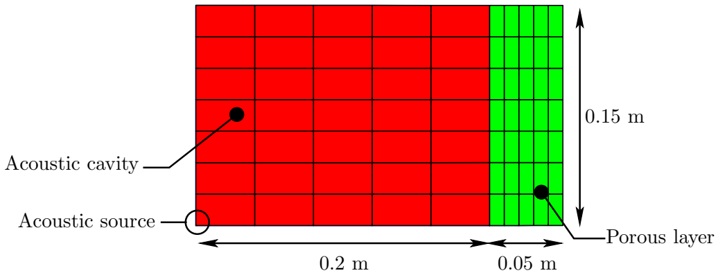
Figure 4.1: Mesh and dimensions of small 2D application
