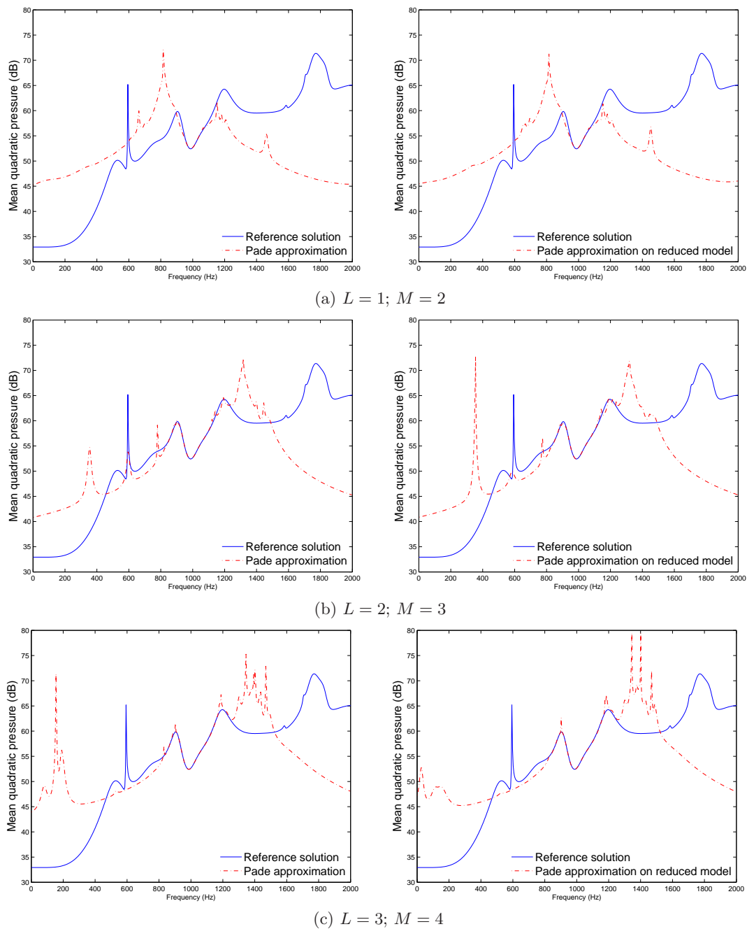
Figure 5.4: Impact of increasing truncation order for power series - 2D poro-acoustic problem. Left: Padé on complete problem; Right: Padé on reduced problem.
