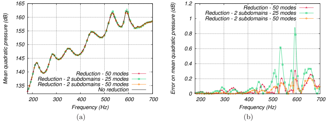
Figure 2.13: Reduction with 2 acoustic components, and a porous layer: (a) FRF with 25 and 50 modes, (b) dB difference to unreduced problem
