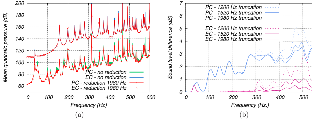
Figure 2.22: Results with truncation up to 1980 Hz: (a) FRF of mean quadratic pressure (b) dB difference to unreduced problem
