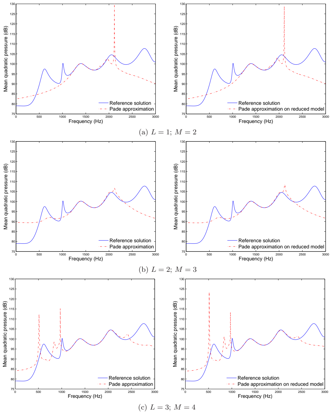
Figure 5.2: Impact of increasing truncation order for power series - 1D poro-acoustic problem. Left: Padé on complete problem; Right: Padé on reduced problem.
