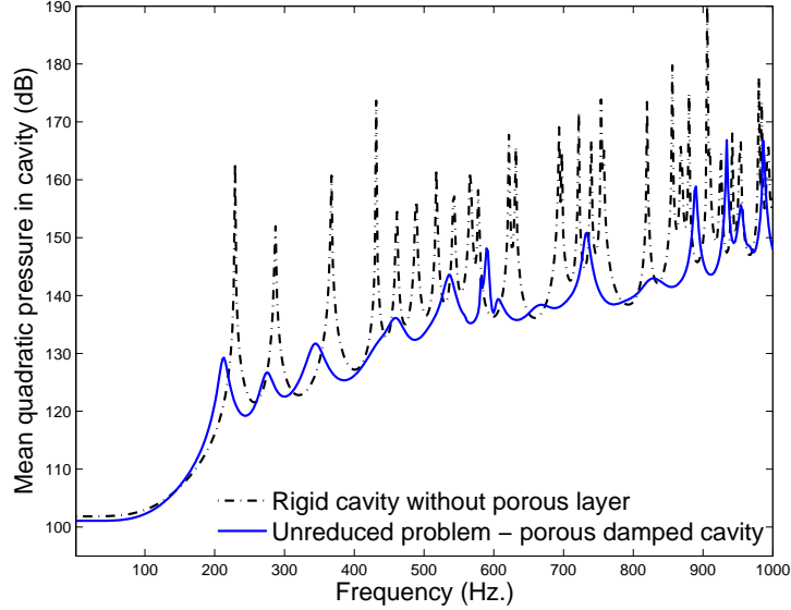
Figure 3.13: Mean quadratic pressure reference FRF, 3D problem
