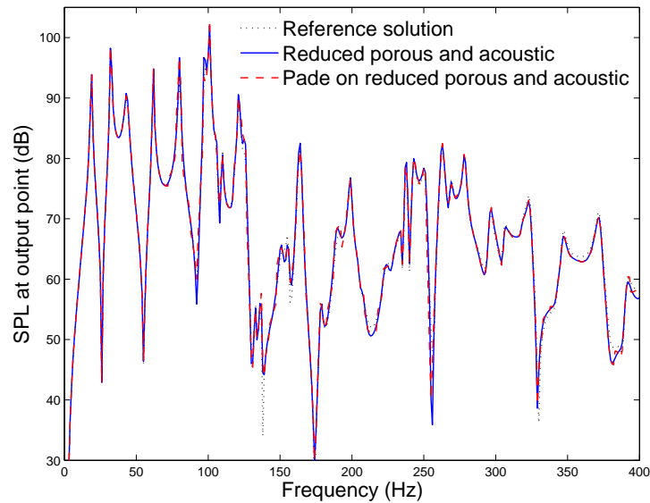
Figure 6.18: Sound pressure level at output point: Padé reconstruction on modal reduction of acoustic (truncation 1250 Hz) and porous (truncation 400 Hz) domains.
