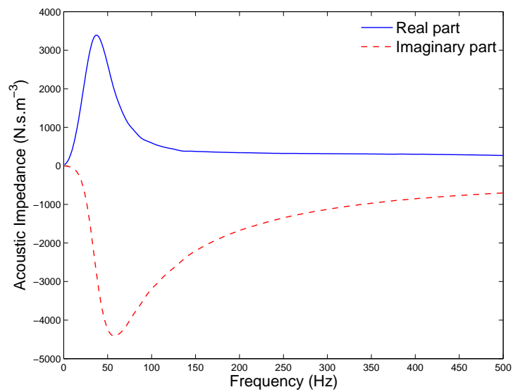
Figure 6.2: Normal acoustic impedance boundary condition.
