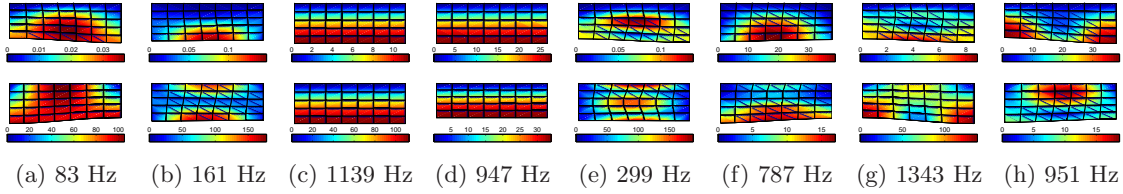
Figure 4.7: Porous 2D selected and sorted mode shapes 1, 2, 21, 15, 4, 12, 26, 16: solid (top) and fluid (bottom) phases. Deformed mesh and norm of displacement.
