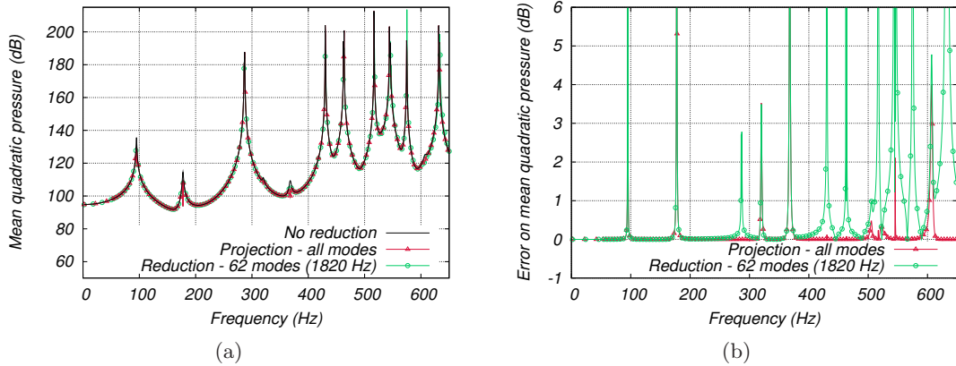
Figure 2.7: Convergence of reduction in receiving cavity: (a) Mean quadratic pressure in dB versus frequency (b) dB difference to unreduced problem
