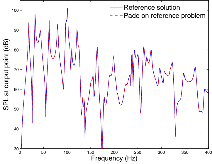
Figure 6.17: Sound pressure level at output point: Padé reconstruction on reference solution.
