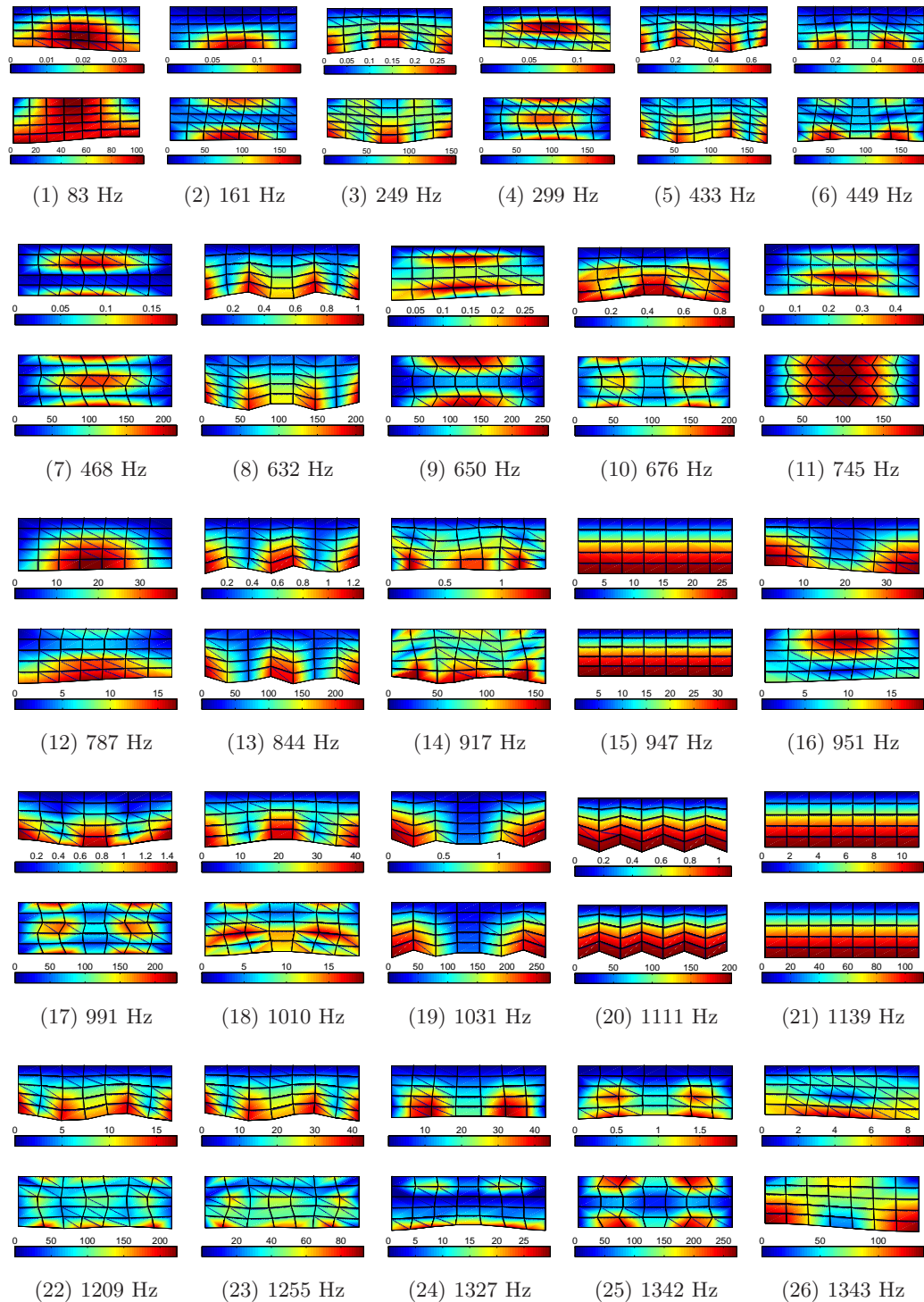
Figure 4.4: Porous 2D mode shapes of modes 1-26: solid (top) and fluid (bottom) phases. Deformed mesh and norm of displacement.
