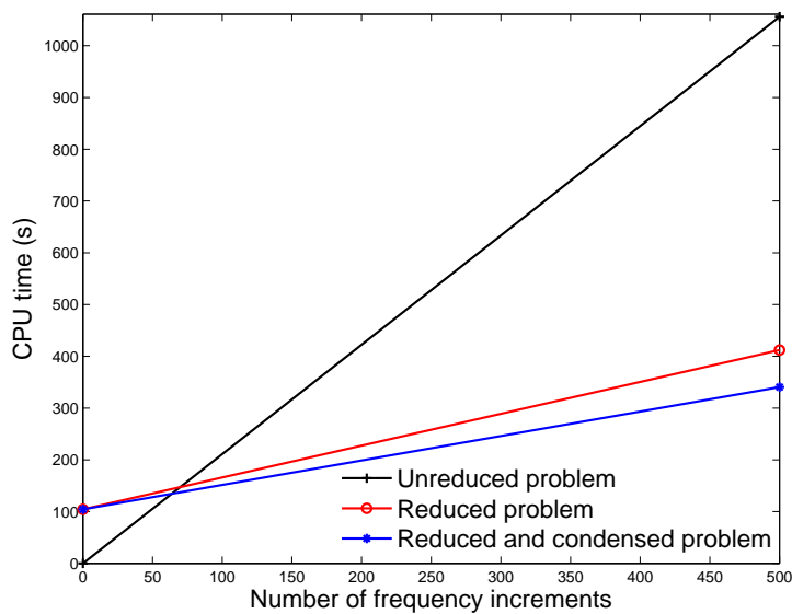
Figure 3.17: CPU time comparison for FRF computation
