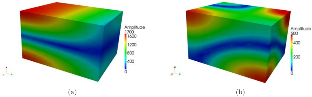
Figure 1.4: Amplitude of the pressure field in the cavity (Lx_a, Ly_a, Lz_a) = (0.3, 0.4, 0.5) m, Lz_p = 0.05 m, at 593 Hz: (a) 3D modelling of porous layer; (b) Normal acoustic impedance boundary condition.
