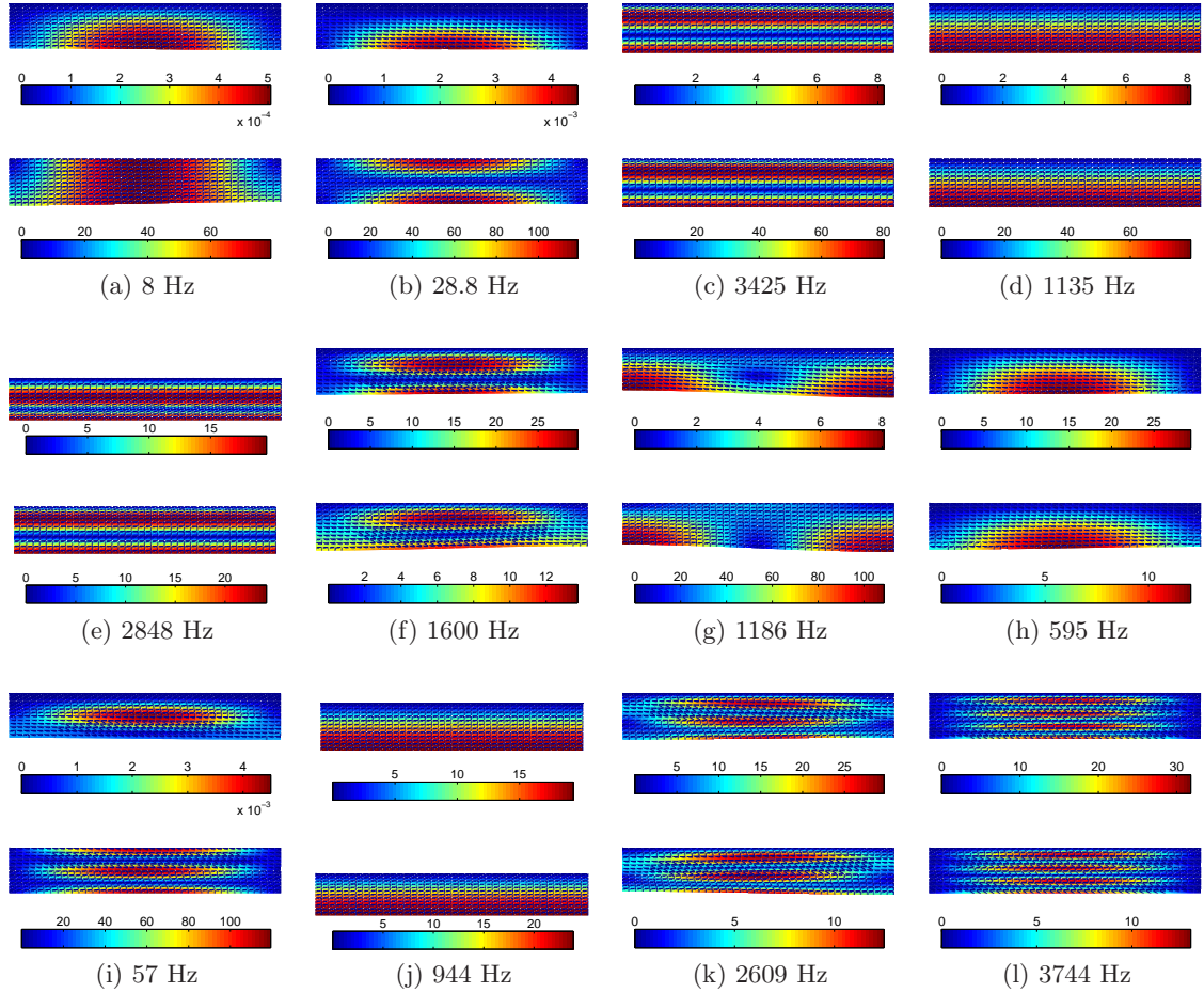
Figure 4.14: Porous 2D selected and sorted mode shapes: solid (top) and fluid (bottom) phases. Deformed mesh and norm of displacement.
