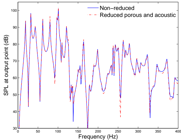
Figure 6.14: Sound pressure level at output point: modal reduction of acoustic (truncation 1250 Hz) and porous (truncation 400 Hz) domains.
