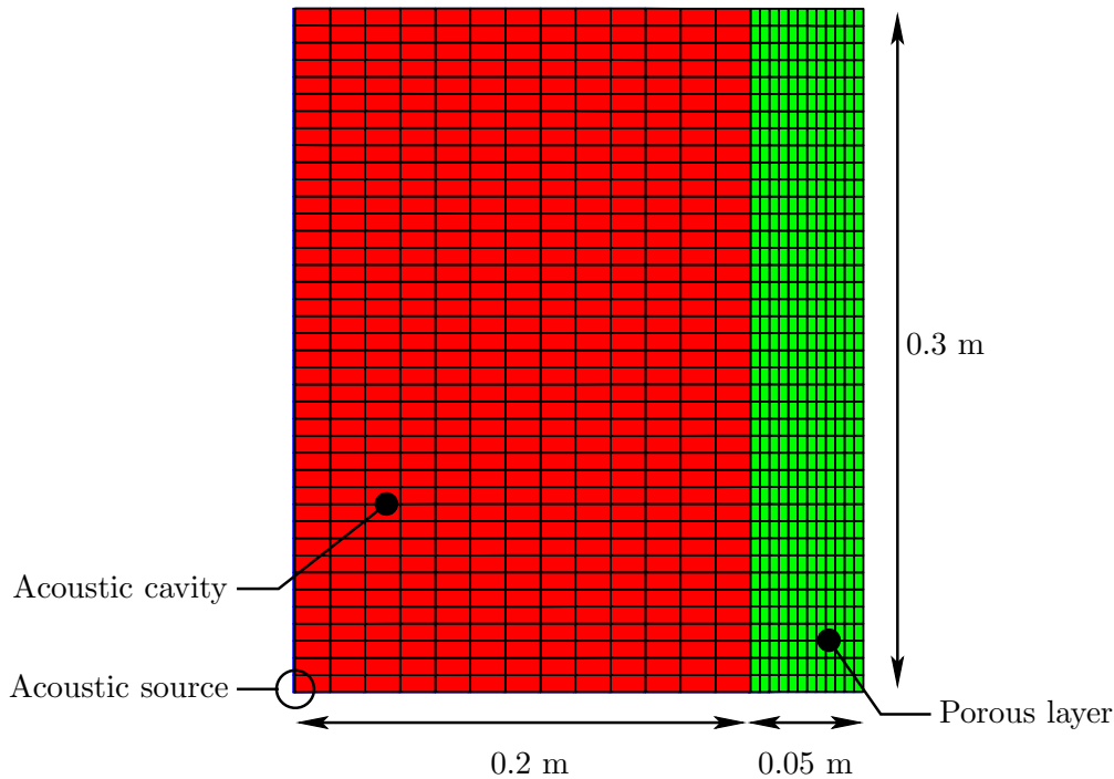
Figure 4.9: Mesh and dimensions of larger 2D application
