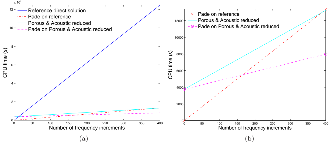
Figure 6.19: Computational time comparison with Padé reconstruction: (a) comparison with reference solution, (b) detailed comparison for acoustic and porous reduced domains.
