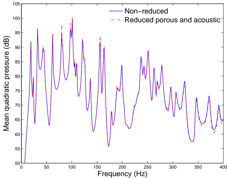
Figure 6.15: Mean quadratic pressure in cavity: modal reduction of acoustic (truncation 1250 Hz) and porous (truncation 400 Hz) domains.
