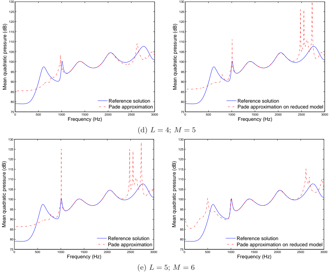
Figure 5.2: Impact of increasing truncation order for power series - 1D poro-acoustic problem. Left: Padé on complete problem; Right: Padé on reduced problem.
