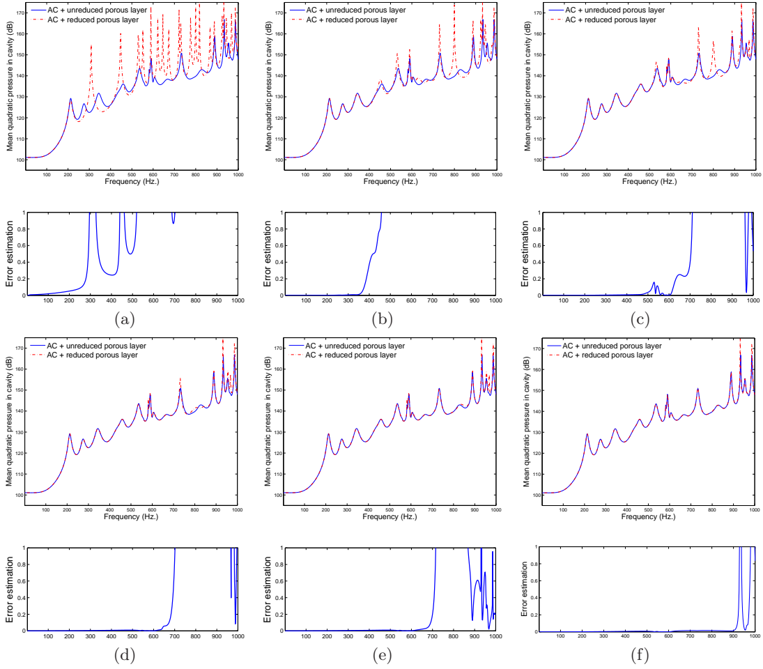
Figure 4.18: Convergence with modal superposition of selected modes for \chi_{\max} = 0.27 : (a) 2 modes, (b) 35 modes; (c) 58 modes; (d) 71 modes; (e) 79 modes; (f) 83 modes
