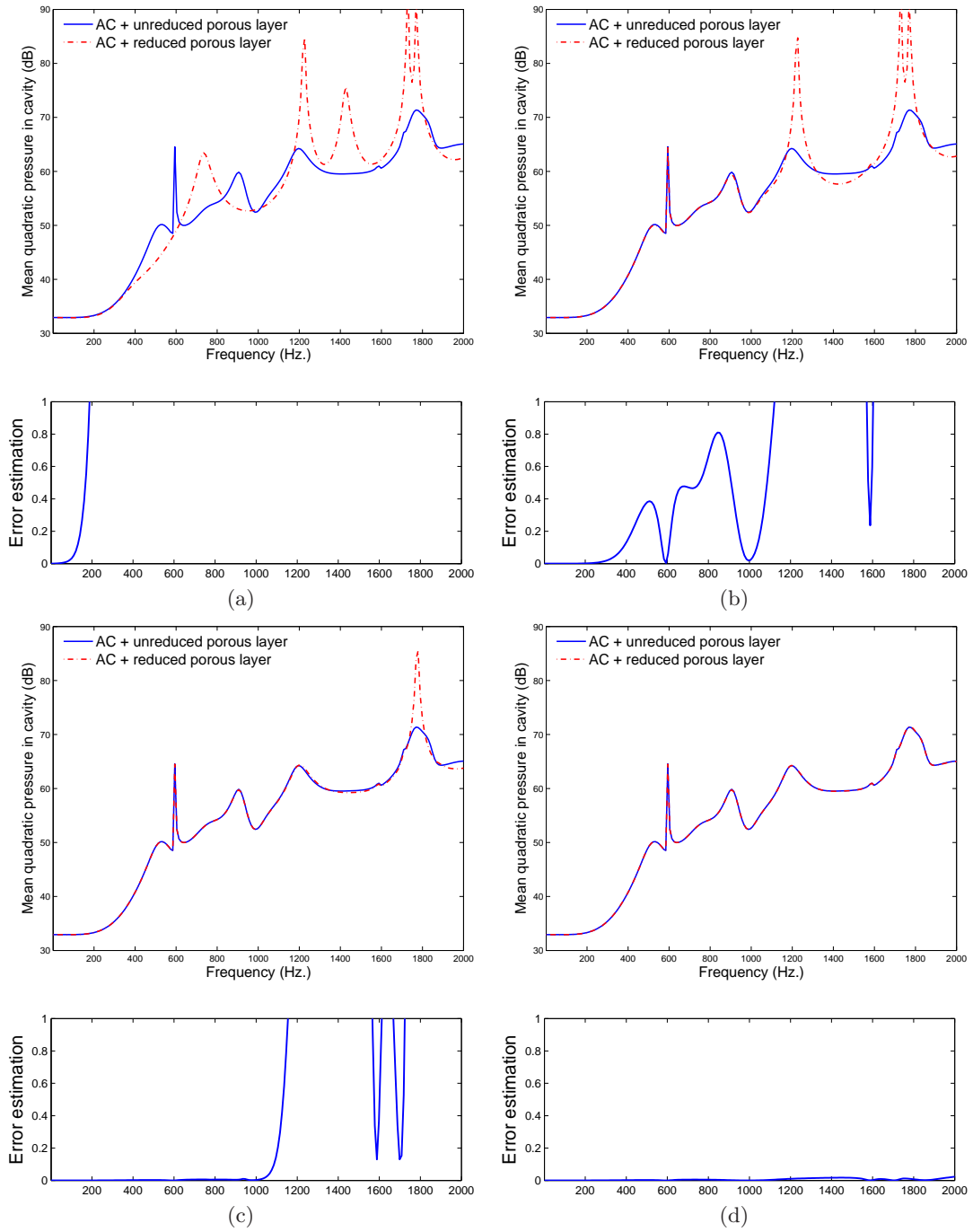
Figure 4.12: Solution convergence for the processed reduced model: (a) 4 modes, (b) 14 modes; (c) 59 modes; (d) 88 modes
