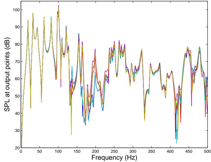
Figure 6.4: Spatial sensitivity of the response, 6 points in a cubic zone of 10 \times 10 \times 10 \text{ cm}^3 .
