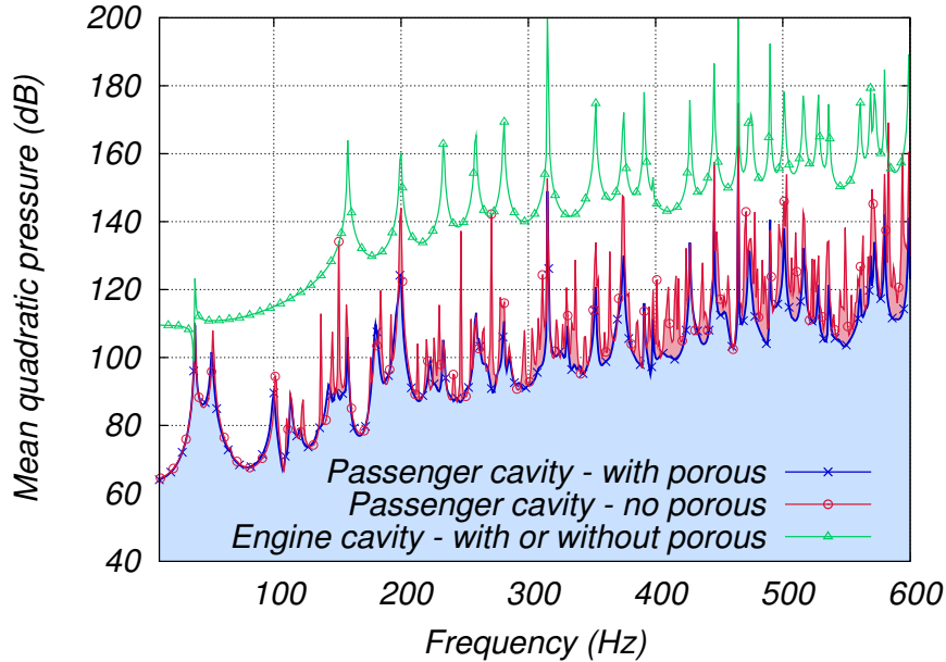
Figure 2.18: Reference FRF with and without porous layer
