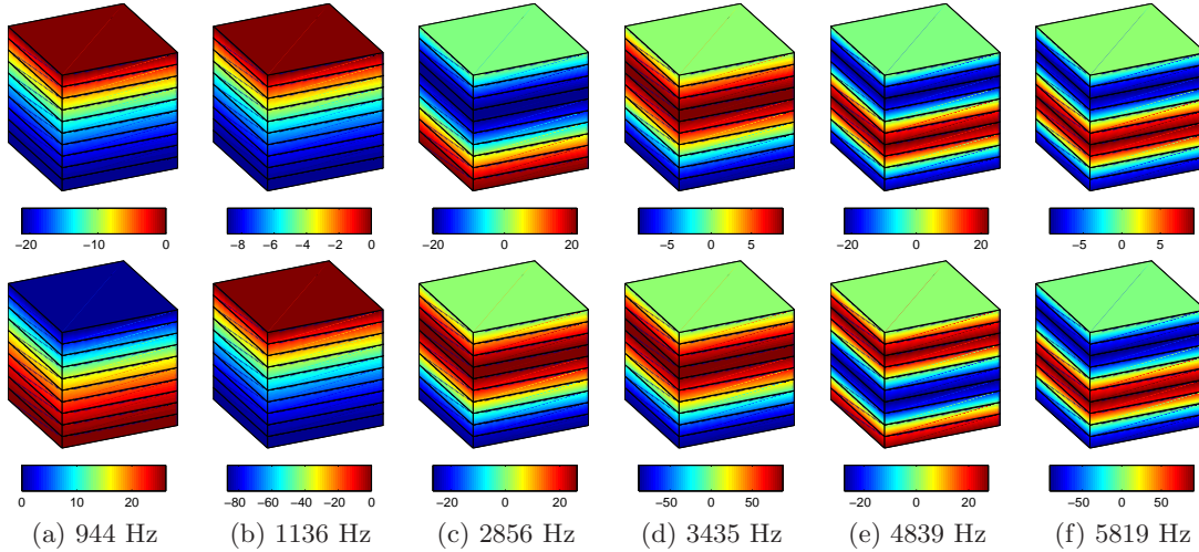
Figure 3.7: First 6 coupled mode shapes of the 1D porous layer (a) – (f), solid (top) and fluid (bottom) phases. Mesh and displacement field.
