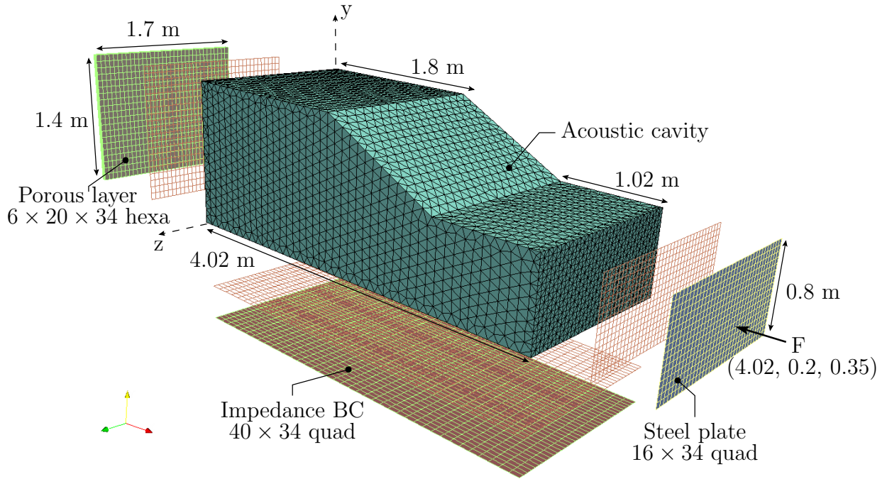
Figure 6.1: Geometry and mesh of the finite element model.
