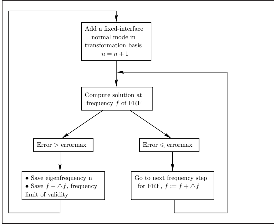
Figure 2.15: Iterative procedure to test influence of restrained or free interface truncation criterion
