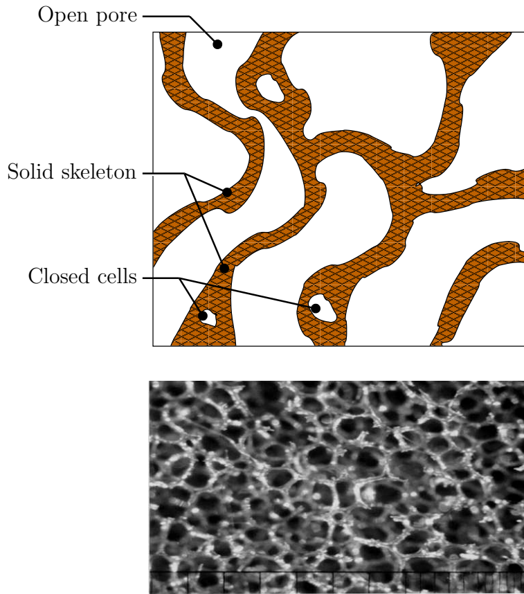
Figure 1.1: A porous material: Top, 2D illustration; Bottom, picture (Courtesy of KU Leuven Laboratory of Acoustics and Thermal Physics).
