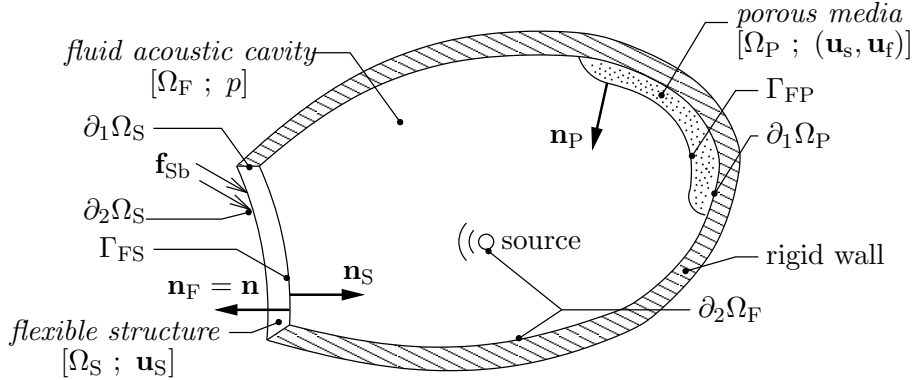
Figure 2.1: Description and notations of the elasto-poro-acoustic interaction problem
