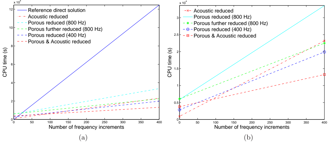
Figure 6.16: Computational time comparison: (a) comparison with reference solution, (b) detailed comparison for acoustic and/or porous reduced domains.
