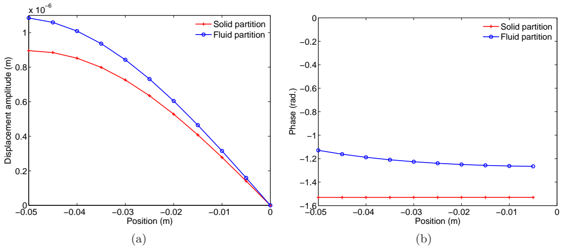
Figure 3.5: Response of the solid and fluid porous partitions at 1010 Hz: (a) Displacement amplitude; (b) Phase.
