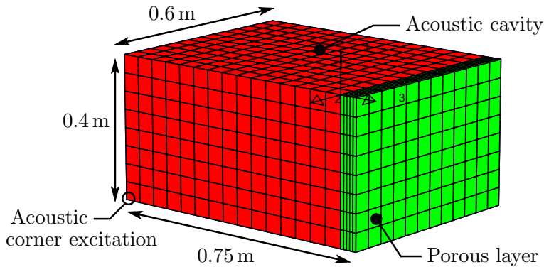
Figure 3.12: Acoustic cavity mesh and dimensions for 3D problem
