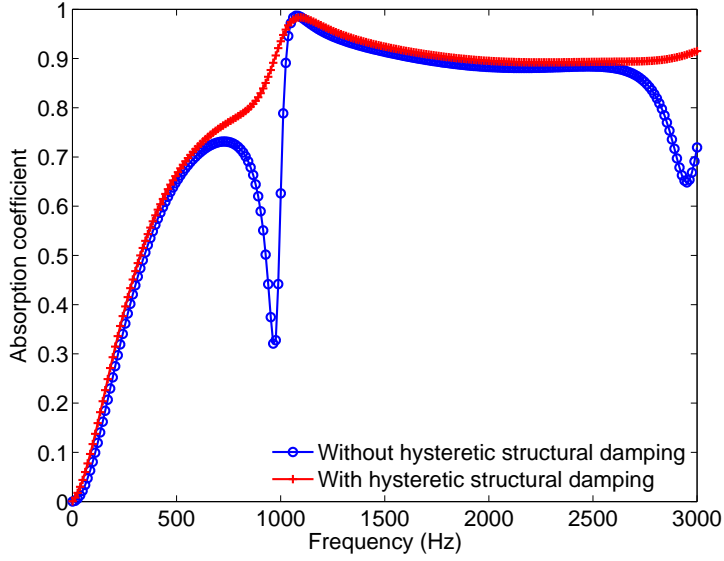
Figure 3.6: Absorption coefficient at normal incidence, impact of the structural damping ( \eta_s = 0.1 ).
