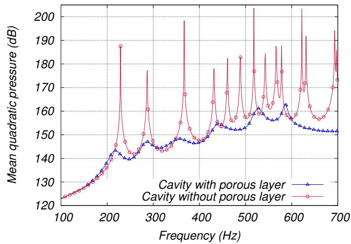
Figure 2.9: Mean quadratic pressure in cavity, with and without the porous layer
