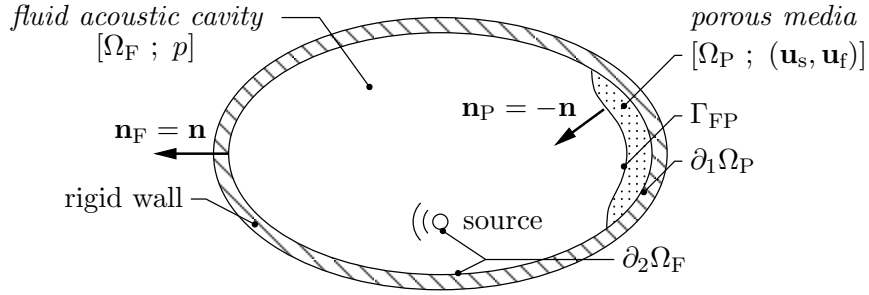
Figure 3.1: Description and notations of the poro-acoustic interaction problem
