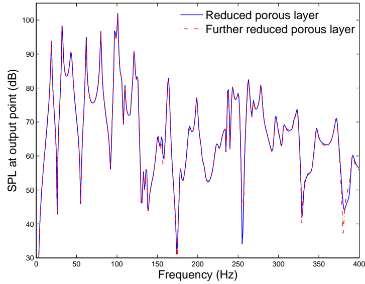
Figure 6.13: Sound pressure level at output point: response with modal truncation at 800 HZ, and further reduction with \chi_{\max} = 0.45 .
