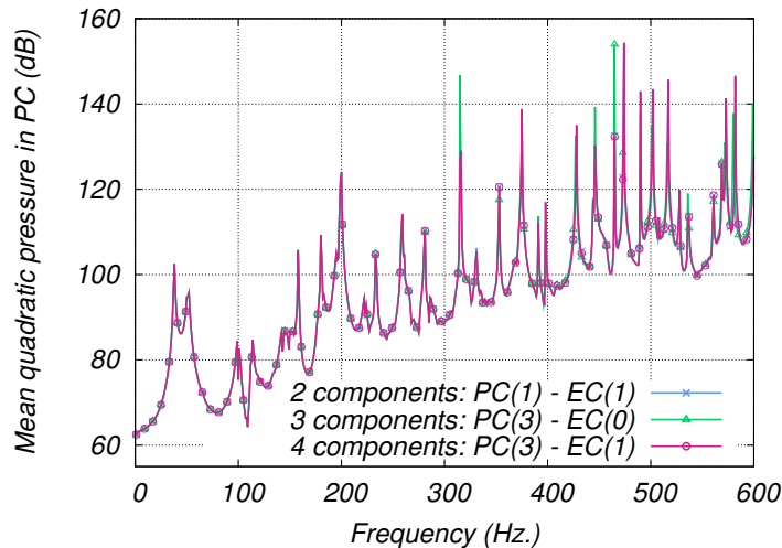
Figure 2.24: FRF in passenger cavity for different decompositions, truncation at 1200 Hz
