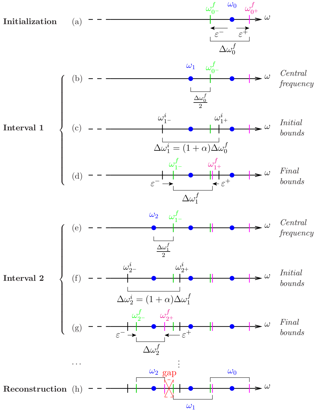
Figure 5.1: Adaptive frequency interval decomposition: blue: central frequency; magenta: upper limit; green: lower limit
