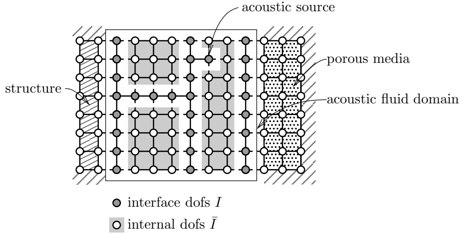
Figure 2.2: Problem description of the substructuring strategy
