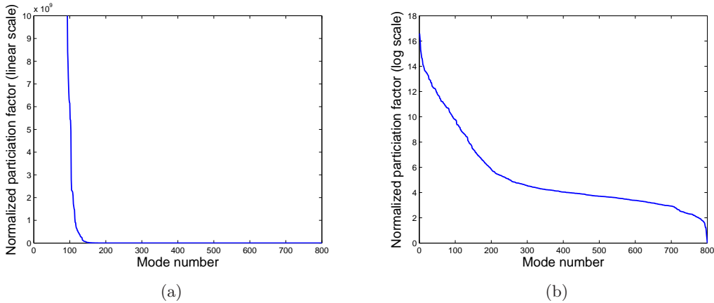
Figure 4.6: Example of normalized modal participation factors: (a) linear scale and (b) logarithmic scale
