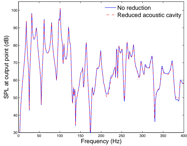
Figure 6.8: Sound pressure level at output point: dynamic condensation of acoustic domain, modal truncation at 1250 Hz.
