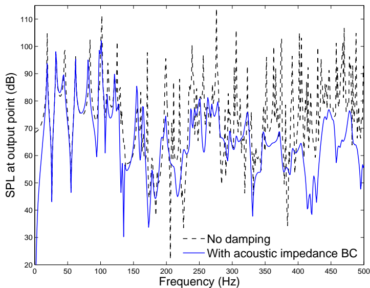
Figure 6.3: Reference sound pressure level response at output point, without 3D porous layer.
