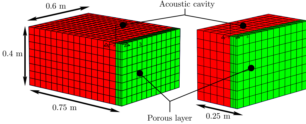
Figure 2.14: Rigid acoustic cavities used for testing the truncation limit criteria
