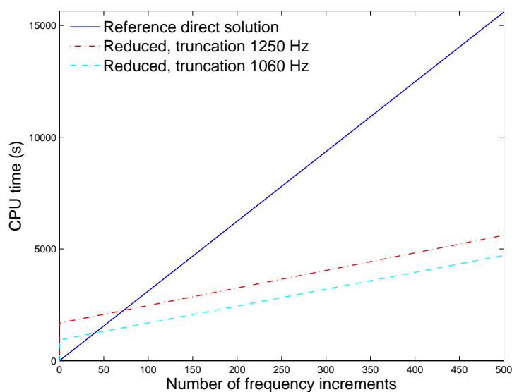
Figure 6.6: Computational time comparison, reference problem without 3D porous layer and dynamic condensation of acoustic domain.
