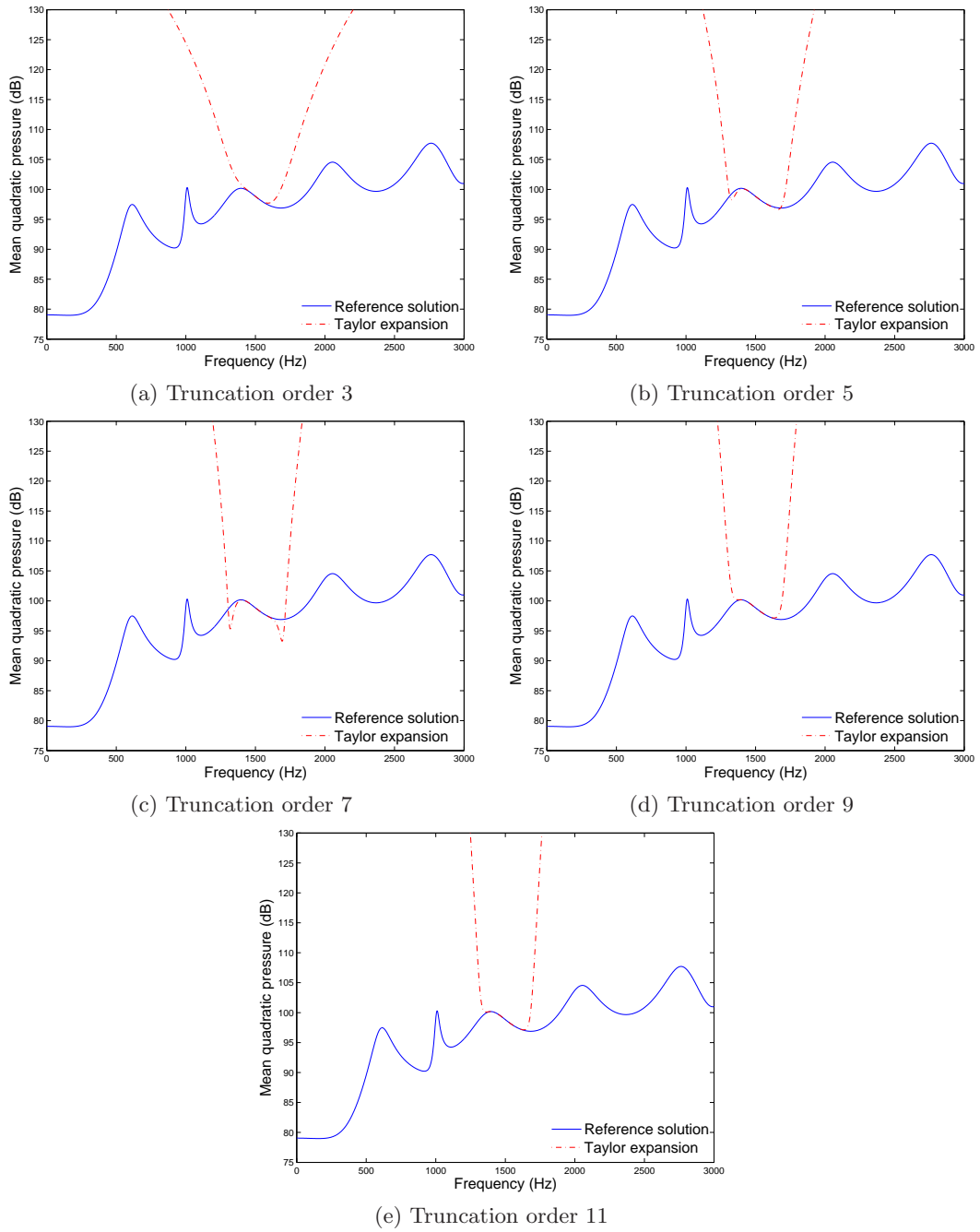
Figure 5.3: Approximation using Taylor expansions - 1D poro-acoustic problem
