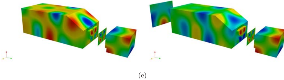
Figure 2.19: Solution without (left) and with (right) porous layer, pressure field in the acoustic cavities, normal displacement in the plate and porous domain. (a) f = 38 Hz, (b) f = 52 Hz, (c) f = 151 Hz, (d) f = 247 Hz, (e) f = 315 Hz
