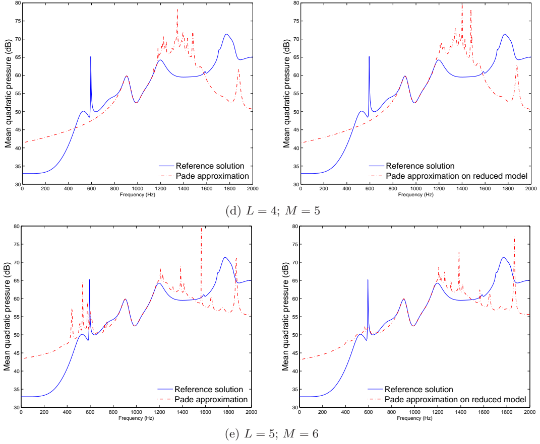
Figure 5.4: Impact of increasing truncation order for power series - 2D poro-acoustic problem. Left: Padé on complete problem; Right: Padé on reduced problem.
