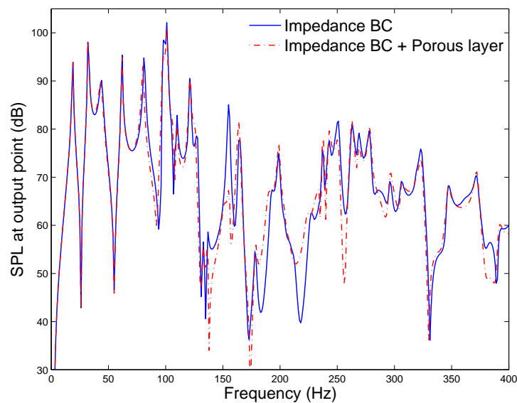
Figure 6.7: Reference sound pressure level response at output point, with 3D porous layer.
