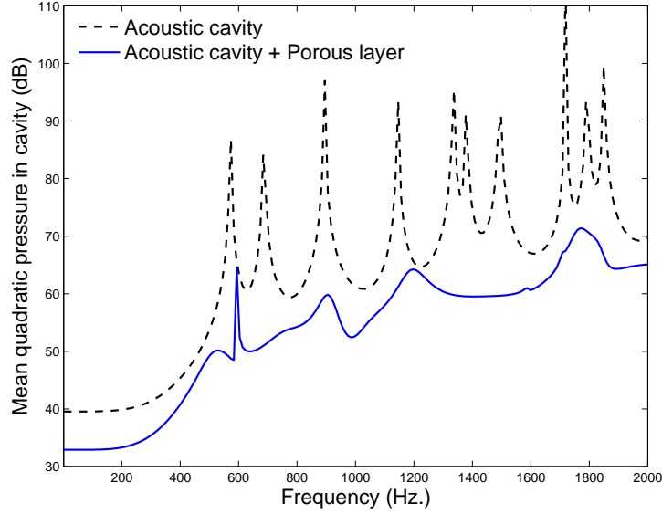
Figure 4.10: Mean quadratic pressure in the acoustic domain
