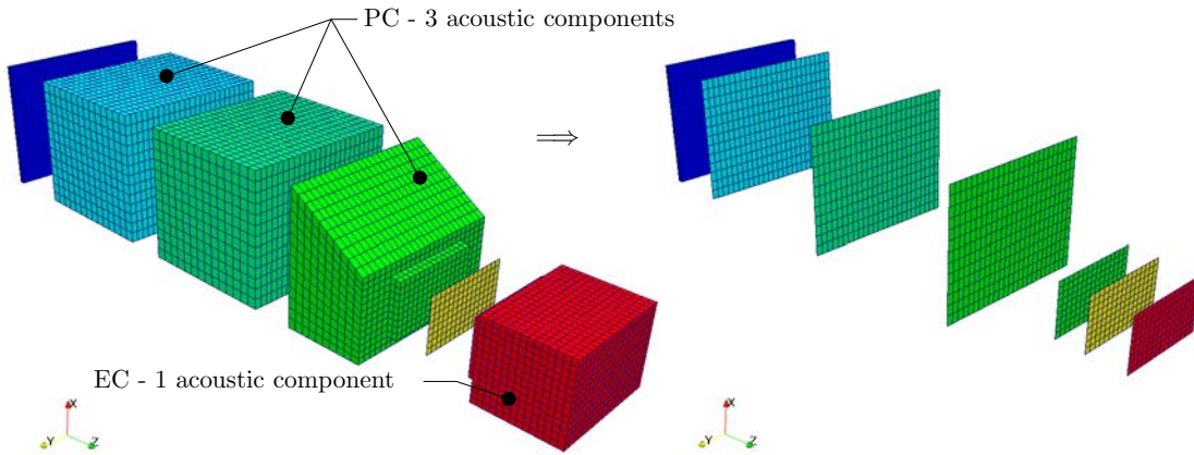
Figure 2.20: Decomposition of the concrete car into 4 acoustic components, and illustration of the reduced problem
