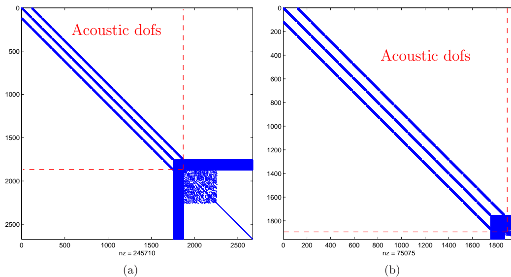
Figure 4.16: Sparsity of the system matrix before and after mode selection procedure: (a) 800 modes, (b) 83 modes
