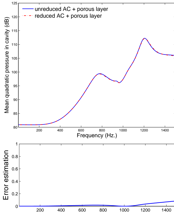
Figure 4.3: Mean quadratic pressure convergence with 26 modes and error estimation
