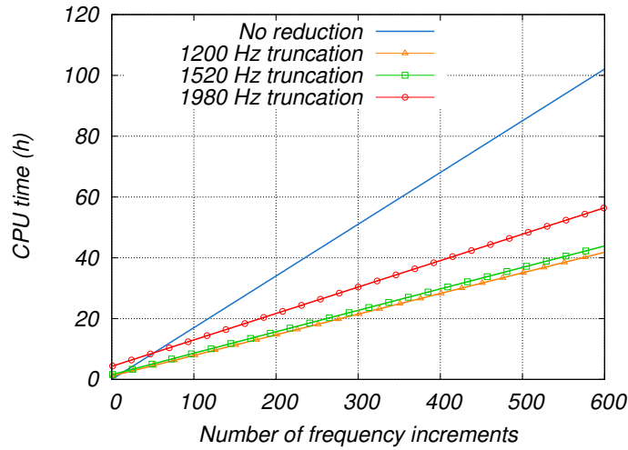
Figure 2.23: CPU time comparison
