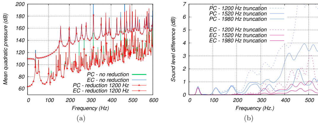
Figure 2.25: Results without porous layer: (a) Mean quadratic pressure, truncation at 1200 Hz, (b) dB difference to unreduced problem, truncation up to 1980 Hz
