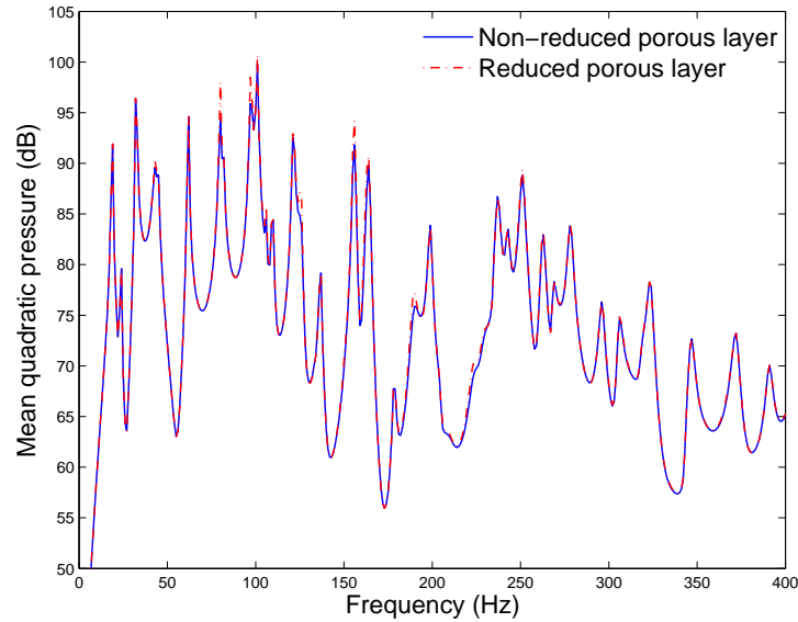
Figure 6.11: Mean quadratic pressure in cavity: reference solution and modal reduction of porous domain, truncation at 400 Hz.
