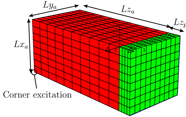
Figure 1.2: Typical poro-acoustic geometry used for comparison between acoustic impedance and 3D poroelastic modelling
