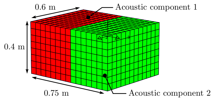
Figure 2.10: Rigid acoustic cavity decomposition into two components
