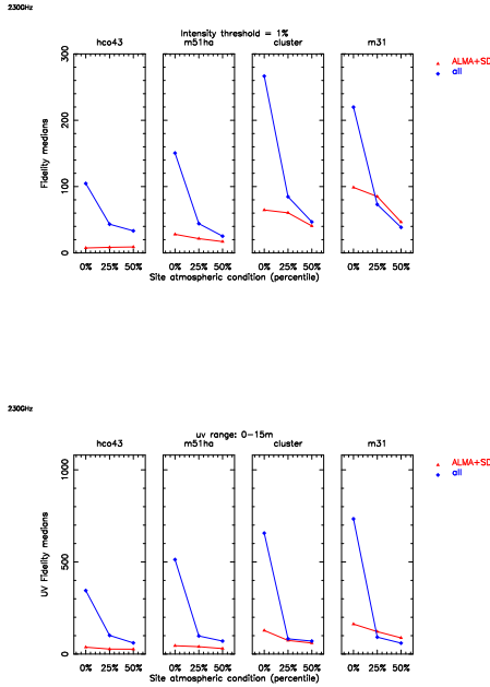
Figure 12: 230 GHz fidelity versus the atmospheric condition. upper panel: Image fidelity medians including all the errors. lower panel: uv-domain fidelity medians in uv range of 0-15m. The red lines: ALMA+SD; the blue lines: ALMA+ACA+SD by the hybrid method
