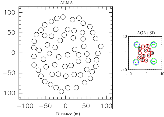
Figure 8: Selected ALMA and ACA configurations. The ALMA compact configuration was designed by M.Yun, and include 64 12-m antennas. The ACA is made of 12 7-m antennas, with close packing limited to 1.25 times the diameter, with 4 12-m antennas used as single-dish.
