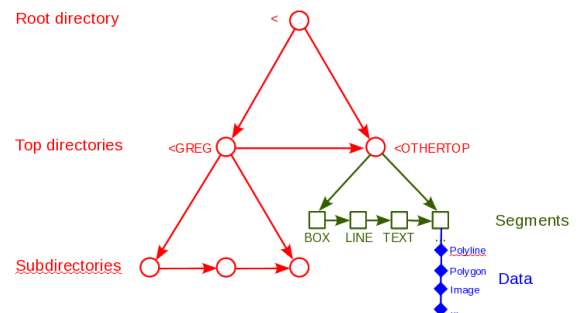
Figure 1: The tree and linked lists structure of the metacode storing the plots in the GTV, with a basic example of top directories, subdirectories, and segments. The relationship presented here between the various elements is not exhaustive.
