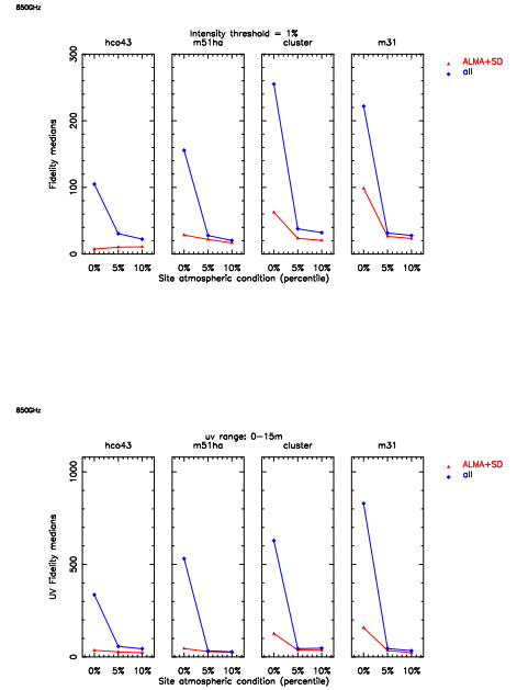
Figure 13: 850 GHz fidelity versus the atmospheric condition. upper panel: Image fidelity medians including all the errors. lower panel: uv-domain fidelity medians in uv range of 0-15m. The red lines: ALMA+SD; the blue lines: ALMA+ACA+SD by the hybrid method
