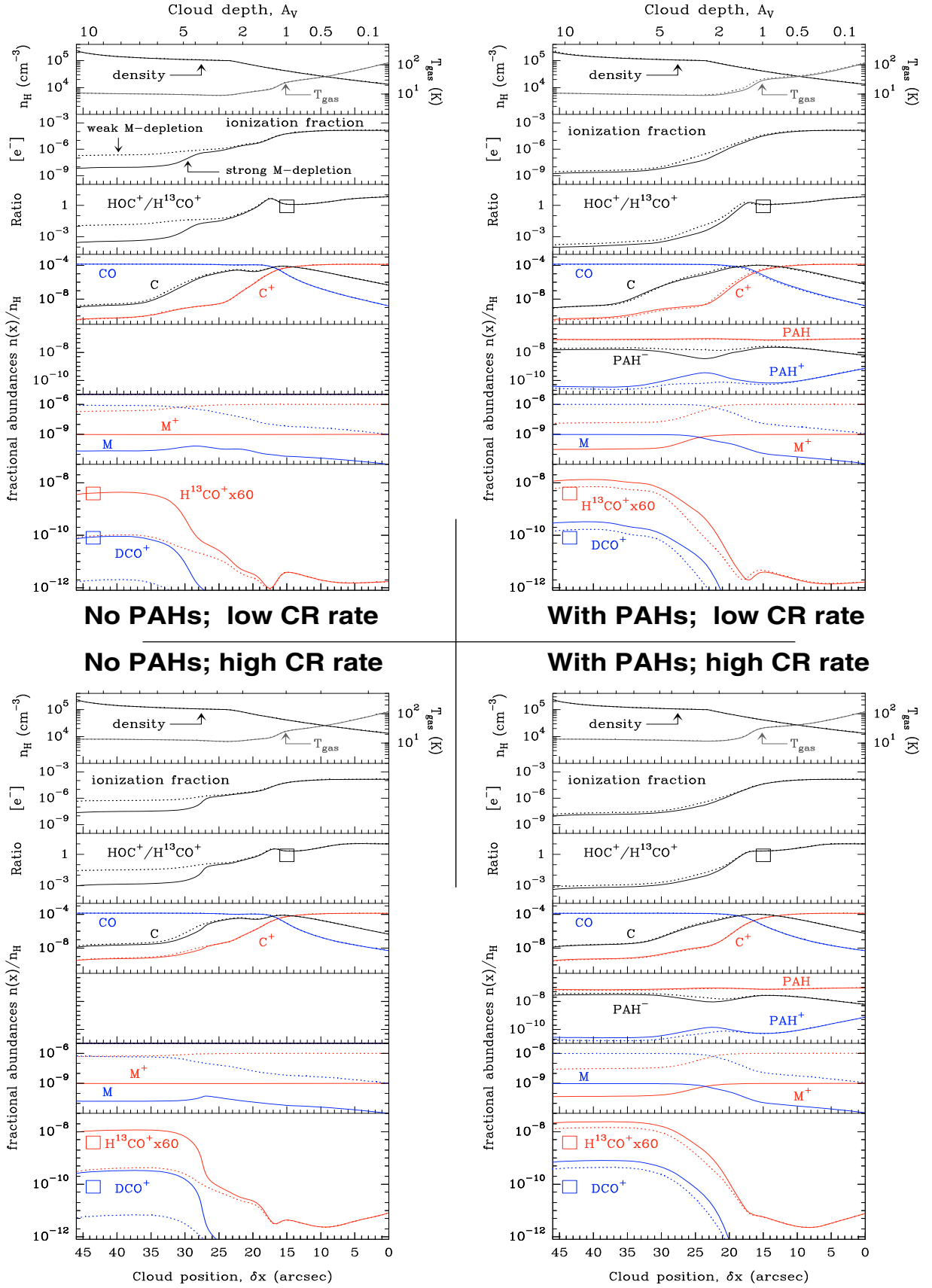
Fig. 4. Grid of chemical models for 2 different metal abundances, low-metallicity with [M] = 10^{-9} ( strong metal depletion case , solid curves) and high-metallicity with [M] = 10^{-6} ( weak metal depletion case , dashed curves). “Low CR rate” refers to models with \zeta = 3 \times 10^{-17} \text{ s}^{-1} while models with “high CR rate” refer to \zeta = 3 \times 10^{-16} \text{ s}^{-1} . Models “with PAH” include PAH-gas interactions in the chemical network (with [\text{PAH}] = 10^{-7} ) while models with “no PAH” are pure gas-phase models. The black empty square represents the [\text{HOC}^+]/[\text{H}^{13}\text{CO}^+] abundance ratio inferred towards the PDR from observations. The blue and red empty squares represent the \text{DCO}^+ and \text{H}^{13}\text{CO}^+ abundances derived towards the core.
