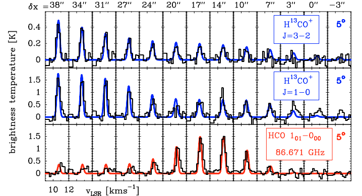
Fig. 3. Observations along a horizontal cut through “the HCO peak” (histograms). The \text{H}^{13}\text{CO}^+ J = 1-0 and HCO 1_{01}-0_{00} lines were mapped with the PdBI at an angular resolution of 6.8'' , whereas the \text{H}^{13}\text{CO}^+ J = 3-2 line was mapped with HERA-30 m (and smoothed to a spatial resolution of 13.5'' ). Radiative transfer models of an edge-on cloud with a line of sight extinction of A_{\text{V}} = 20 , inclined 5^\circ relative to the line of sight for HCO (red curve), and \text{H}^{13}\text{CO}^+ (blue curves) are shown. The single- T_{\text{ex}} HCO model assumes a 12'' width filament with a column density of 3.2 \times 10^{13} \text{ cm}^{-2} , while N(\text{HCO}) is 4.6 \times 10^{12} \text{ cm}^{-2} behind the filament. The \text{H}^{13}\text{CO}^+ model assumes a constant density of n(\text{H}_2) = 5 \times 10^4 \text{ cm}^{-3} with T_{\text{k}} = 60 \text{ K} and N(\text{H}^{13}\text{CO}^+) = 5.8 \times 10^{11} \text{ cm}^{-2} for \delta x < 35'' ; and T_{\text{k}} = 10 \text{ K} and N(\text{H}^{13}\text{CO}^+) = 7.6 \times 10^{11} \text{ cm}^{-2} for \delta x > 35'' . Modeled line profiles have been convolved with an appropriate Gaussian beam corresponding to each PdBI synthesized beam or 30 m main beam resolution.
