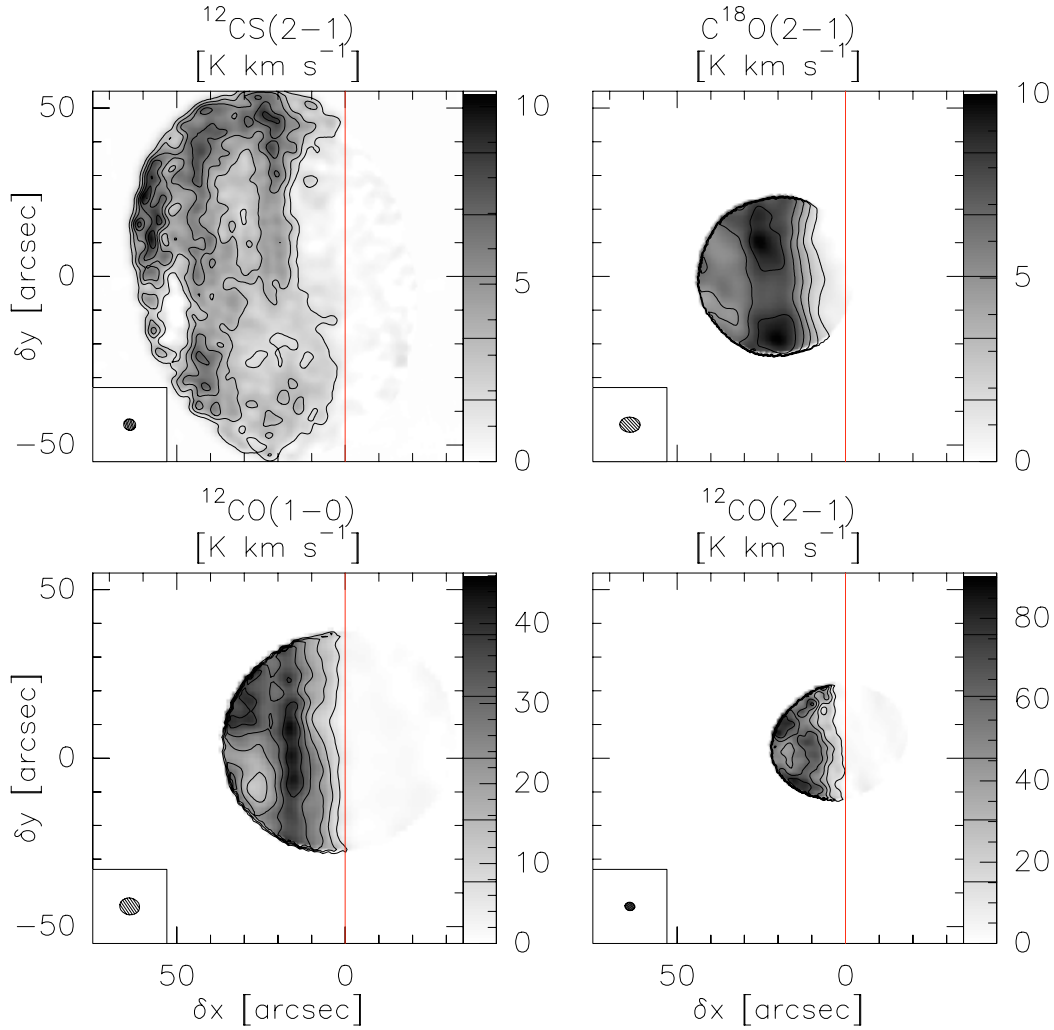
Fig. 1. Integrated emission maps obtained with the Plateau de Bure Interferometer. The center of all maps has been set to the mosaic phase center: RA(2000) = 05h40m54.27s, Dec(2000) = -02^{\circ}28'00'' . The map size is 110'' \times 110'' , with ticks drawn every 10'' . The synthesized beam is plotted in the bottom left corner. The emission of all lines is integrated between 10.1 and 11.1 km s ^{-1} . Values of contour level are shown on each image wedge. The four panels are shown in a coordinate system adapted to the source: i.e. maps have been rotated by 14^{\circ} counter-clockwise around the image center to bring the exciting star direction in the horizontal direction as this eases the comparison of the PDR models. Maps have also been horizontally shifted by 20'' to set the horizontal zero at the PDR edge, delineated by the vertical line.
