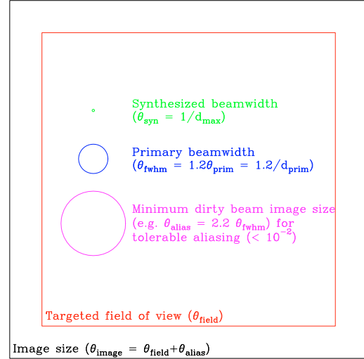
Fig. 1. Visualization of the different angular scales relevant to wide-field interferometric imaging. The notion of anti-aliasing scale ( \theta_{\text{alias}} ) is introduced and discussed in Sect. 4.2.
