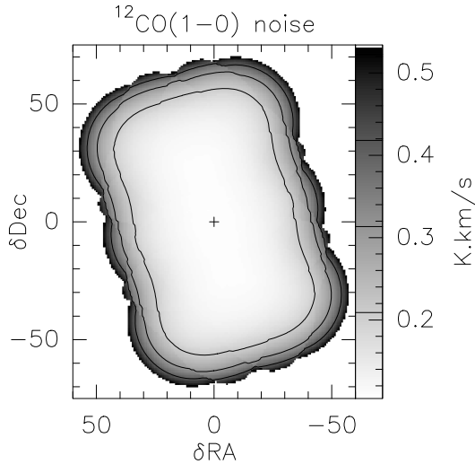
Fig. A.1. Map of the noise level in \text{K km s}^{-1} over the 13-field mosaic.
