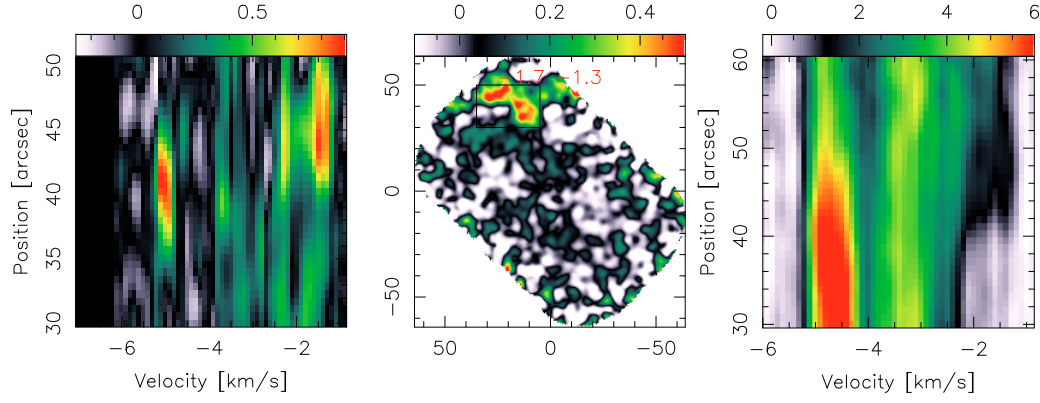
Fig. 7. Position-velocity diagrams across the pair of structures [#3, #8]. Left: cut across the PdBI-only map. Center: rotated PdBI channel-map [-1.7, -1.3] km s ^{-1} , showing the direction and distance (horizontal size of the box) over which the CO emission is averaged for the cut. The cut runs from the southern to northern edge of the box. Right: same across the PdBI+30m data cube.
