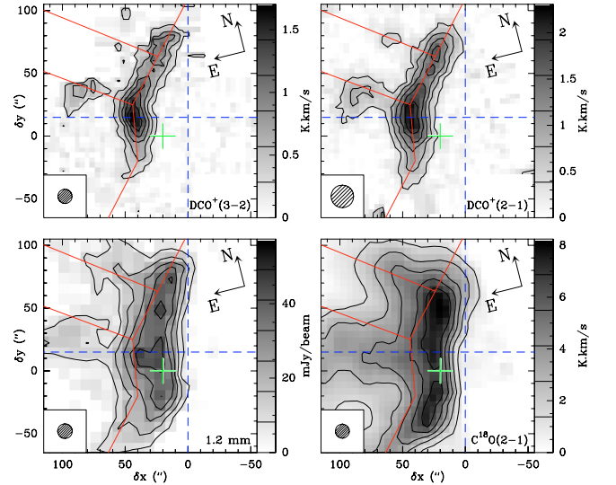
Fig. 1. IRAM-30 m integrated intensity maps. Maps have been rotated by 14^\circ counter-clockwise around the projection center, shown as the green cross at (\delta x, \delta y) = (20'', 0'') , to bring the exciting star direction in the horizontal direction and the horizontal zero has been set at the PDR edge, delineated by the dashed blue vertical line. The spatial resolution is plotted in the bottom left corner. Values of contour levels are shown on each image lookup table. The emission of all lines is integrated between 10.1 and 11.1 km s -1 .
