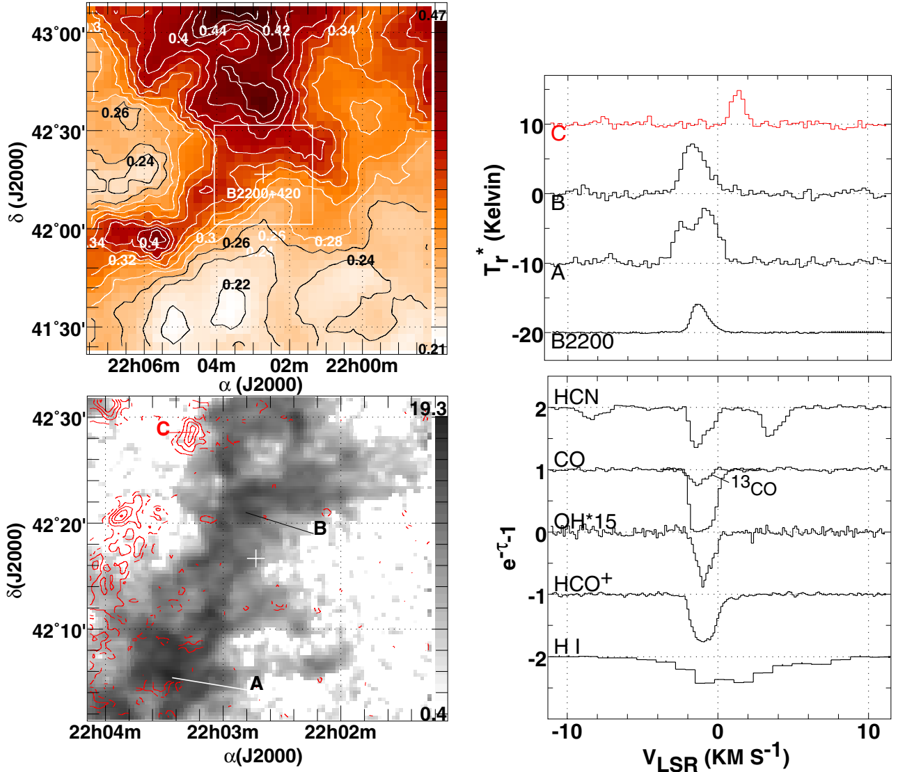
Fig. 9. The sky field around the position of B2200+420 (BL Lac), as in Fig. 2. The map of CO emission at lower left superposes the integrated intensity in the range v = 0 – 2 km s -1 as red contours against a background grayscale representing emission at v \leq 0 km s -1 . Molecular absorption and most emission is sequestered in the blue wing of the core of the HI absorption profile but a red-shifted emission component is present to the Northeast as illustrated by the spectrum at position “C” indicated at lower left .
