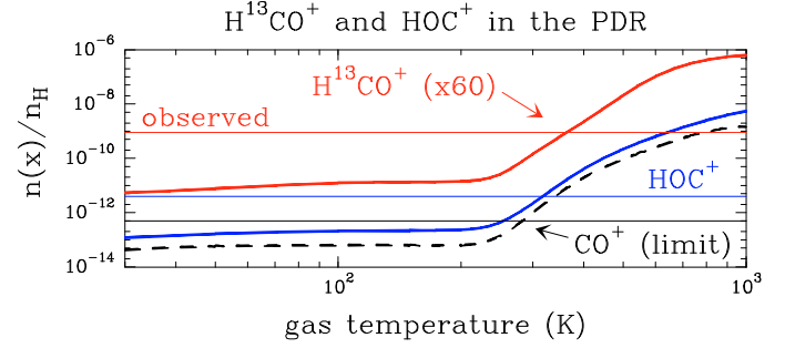
Fig. 3. Predicted \text{H}^{13}\text{CO}^+ , \text{HOC}^+ and \text{CO}^+ peak abundances in the PDR ( A_V \approx 0.5\text{--}1.5 ) as a function of gas temperature. \text{H}^{13}\text{CO}^+ and \text{HOC}^+ abundances (and \text{CO}^+ abundance upper limit) derived from observations towards the PDR position are shown with horizontal thin lines.
