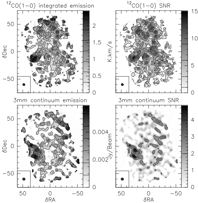
Fig. 2. Map of integrated emission of the PdBI data ( top left ), and signal-to-noise ratio ( top right ) for the ^{12}\text{CO}(J = 1-0) line. Same for the 3 mm continuum emission ( bottom panels ). The synthesized beam is shown in the bottom left inserts.
