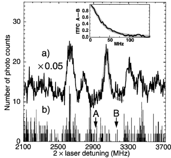
Figure 5.17: a) integrated TPE spectrum. b) one scan spectrum. A and B are the two extreme frequencies for the scan series necessary for the ITFC integration. Inset: ITFC graph.
