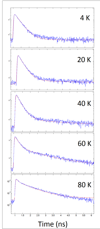
Figure 2.5: Temperature dependent decay time curves from 4K to 80K
