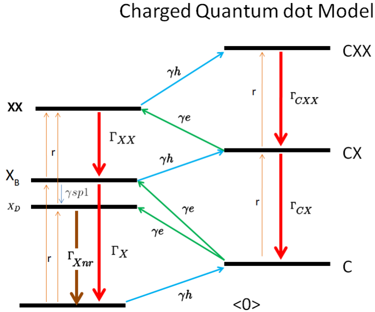
Figure 4.3: Model for a charged quantum dot
