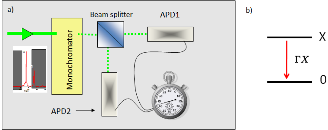
Figure 1.13: a) autocorrelation (antibunching) setup, b) two level system model
