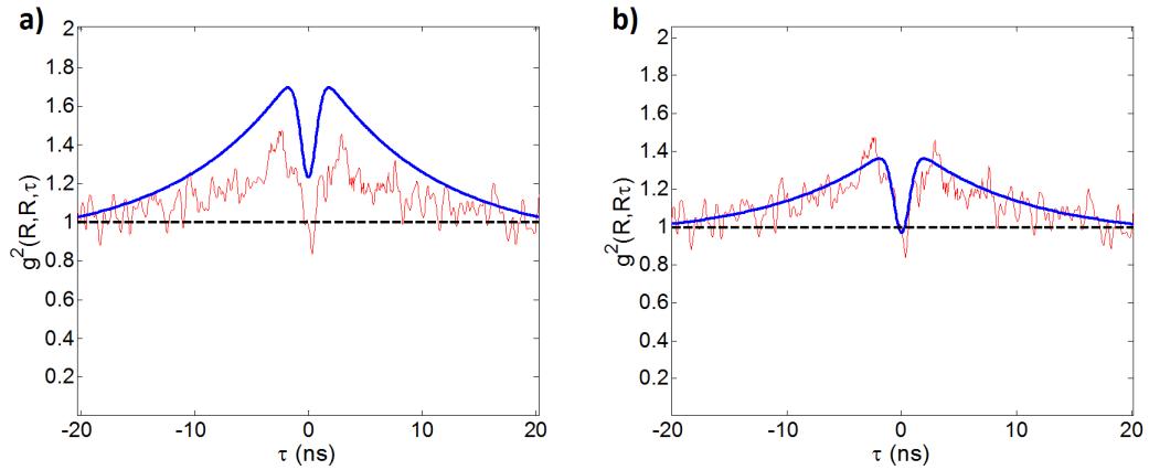
Figure 5.21: a) Autocorrelation of the half-line. The theoretical curve calculated with the infinitely sharp homogeneous line model is plotted in blue, experimental data in red. b) Theoretical curve corrected with the parameter \beta = 0.5 .
