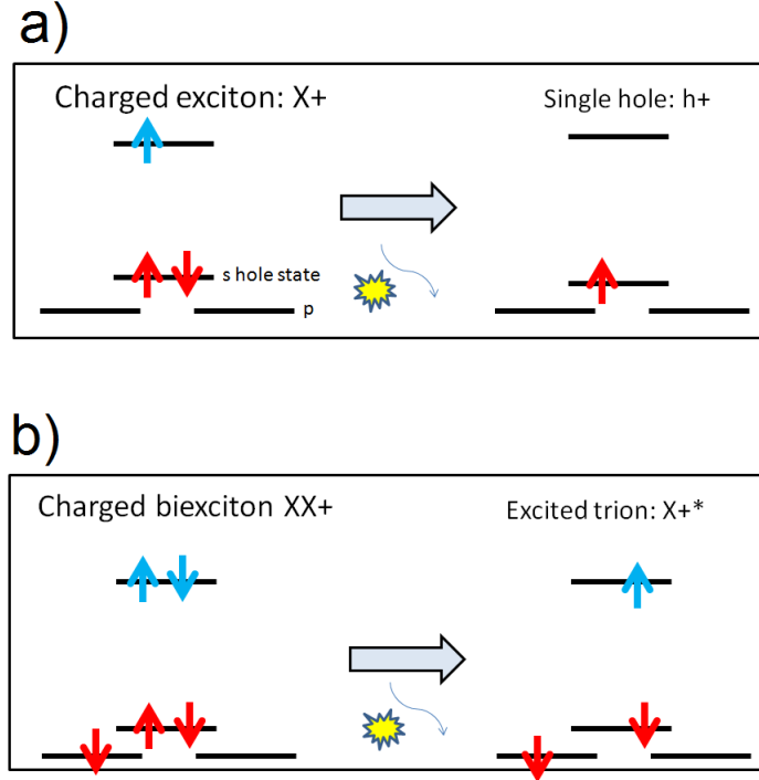
Figure 4.7: Scheme of the transition between a) charged exciton and single hole, b) charged biexciton and excited trion
