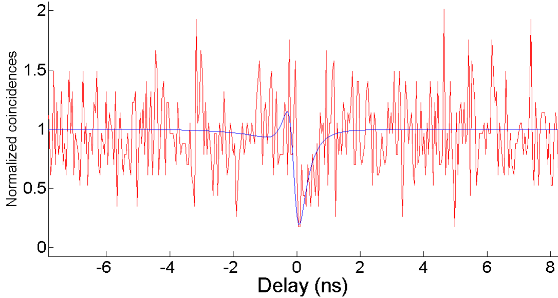
Figure 4.6: Charged biexciton ( CXX1 + CXX2 ) / biexciton cross correlation
