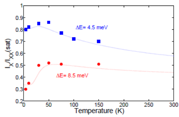
Figure 2.12: Exciton/biexciton intensity ratio as a function of the temperature for two different \Delta E . Squares and dots are experimental values for 2 different quantum dots.
