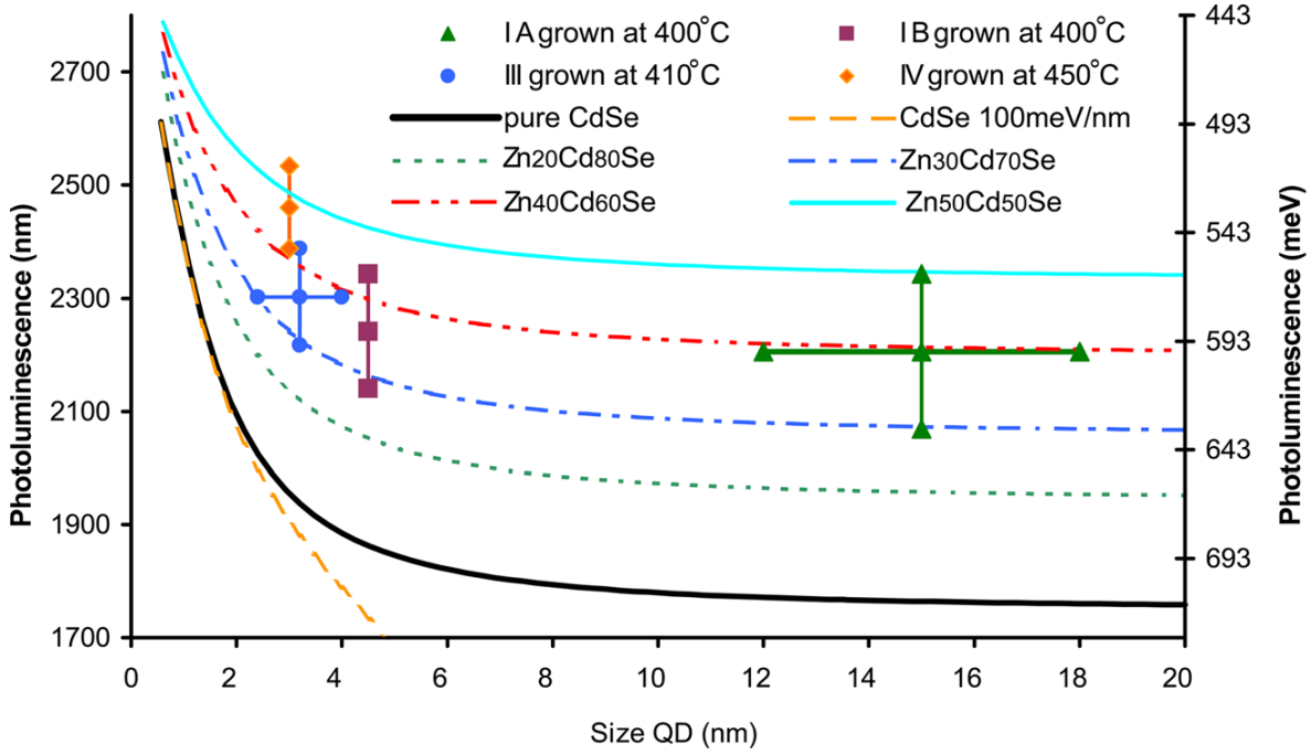
Figure 1.7: Photoluminescence energy vs QD size for different samples. Size error bars are based on the distribution of values obtained by TEM observations, and energy error bars are based on the PL emission range of a given sample. Calculations were done by Regis Andre.
