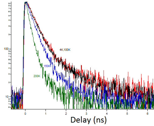
Figure 3.8: Temperature dependence of biexciton decay time
