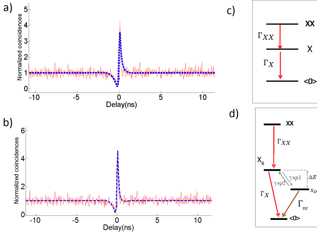
Figure 2.4: a) exciton/biexciton cross correlation figure, (dashed line) simulation obtained from the 3 levels model (c)). (b) exciton/biexciton cross correlation figure, (dashed line) simulation obtained from the 4 levels model (d)) including the dark exciton. For both models, the pump rate was fixed at r = 3ns^{-1}
