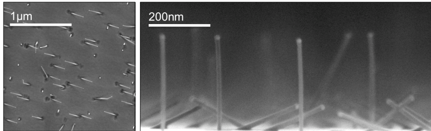
Figure 1.5: ZnSe/CdSe/ZnSe NWs grown a ZnSe buffer. a, Top view SEM image showing a majority of uniform NWs inclined respect to the substrate surface. The bright dots are the NWs standing straight up. b, Perpendicular SEM view of the same sample.
