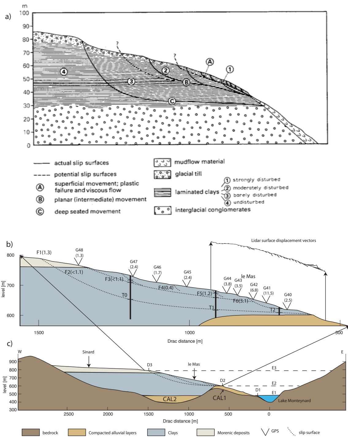
Figure 4.51: a) Idealised section across a slope in laminated clays to show potential and actual slip surfaces.(Giraud et al., 1991) b) Interpreted cross-section of the Avignonet landslide. G40-48 show the average GPS-velocities from 1995-2009 in cm/a. F1-6 are scarps identified on the shaded Lidar-DEM. In brackets an average displacement rate calculated from the difference of GPS-velocities of the accompanying blocks. T0-T2 are boreholes with inclinometric measurements and slip surfaces marked as small horizontal lines. c) Extended cross-section after (Monjuvent, 1973; Bièvre, 2010). D1: contact bedrock/CAL, D2: contact CAL/clays, D3: upper landslide limit, E1-3: accompanying elevation levels before incision.
