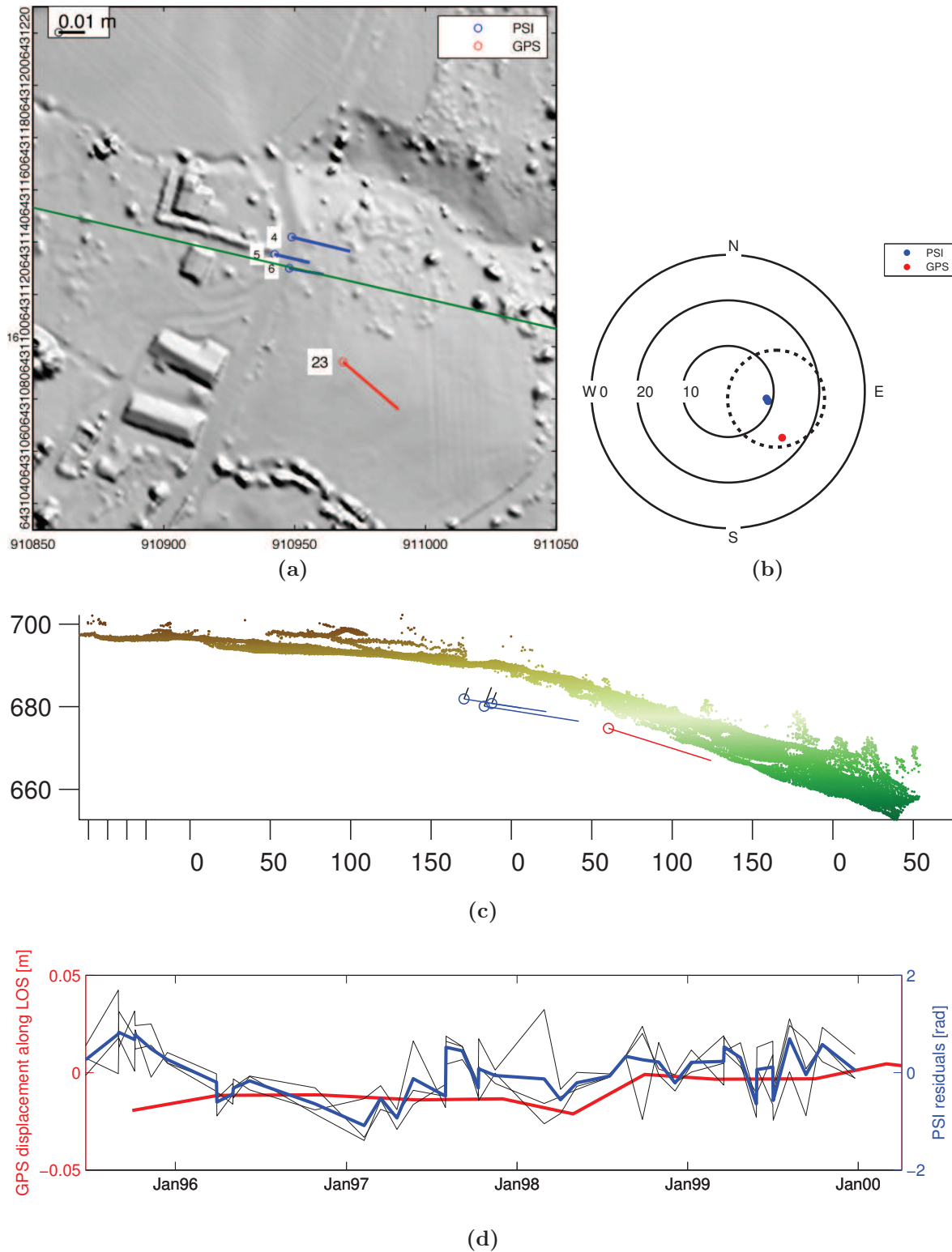
Figure 4.47: PSI results at A3 (overview in Fig. 4.44) a) unfiltered Lidar DEM with interpreted LOS-displacements (blue), GPS-displacement (red) and profile location (green) b) circular plot of PSI- and GPS-displacement orientation c) DEM cross-section with PSI- and GPS-displacements, the displacements are plotted below the terrain-surface for better visualisation, the shorter black lines at the PSI-displacements indicate the LOS-displacements. d) time-series of the portion in LOS-direction from the GPS-displacement (red), the PSI-residual phases per point (black) and the average PSI-residuals (blue)
