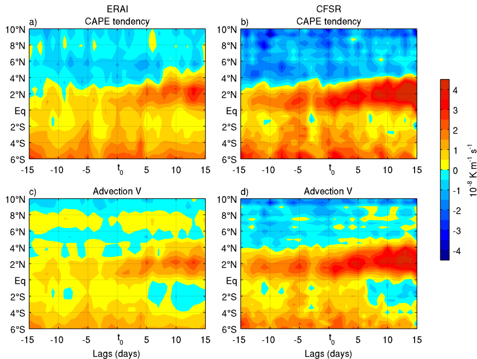
Figure 58. – Mean composites computed from t_0 of each year between 10–6°W of (a-b) the CAPE tendency field and the (c-d) meridional advection term contributing to the CAPE tendency with ERAI (left) and CFSR (right).
