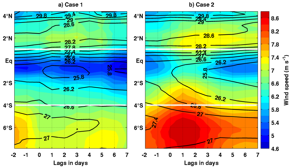
Figure 32. – QuikScat wind speed (colours, \text{m s}^{-1} ) and TMI SST (black contours, ^{\circ}\text{C} ) composites for (a) case 1 and (b) case 2 (see text for details). White lines limit the various areas of the Gulf.
