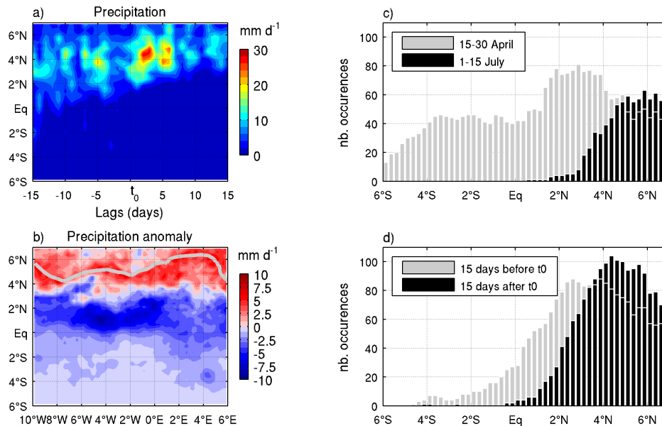
Figure 57. – (a) Composites computed from t_0 of each year (2000-2009), in average between 10^{\circ}\text{W} - 6^{\circ}\text{W} . (b) Difference maps between the mean composite of 15 days after t_0 minus the mean composite of 15 days before t_0 for TRMM precipitations ( \text{mm d}^{-1} ). (c) TRMM daily precipitation occurrences during the 15 last days of April (grey bars) and the 15 first days of July (black bars). (d) TRMM daily precipitation occurrences during the 15 days before t_0 (grey bars) and the 15 days after t_0 (black bars). An occurrence is define as a daily precipitation higher than 5 \text{ mm d}^{-1} averaged between 10^{\circ}\text{W} - 6^{\circ}\text{W} .
