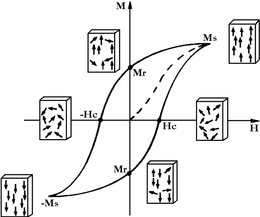
Figure 3.1.2: Ferromagnetic hysteresis curve showing the evolution of magnetization M with the external field H . Arrows correspond to magnetic domain orientation. M_s = saturation magnetization, M_r = remanant magnetization and H_c = coercive force or coercivity of remanence.
