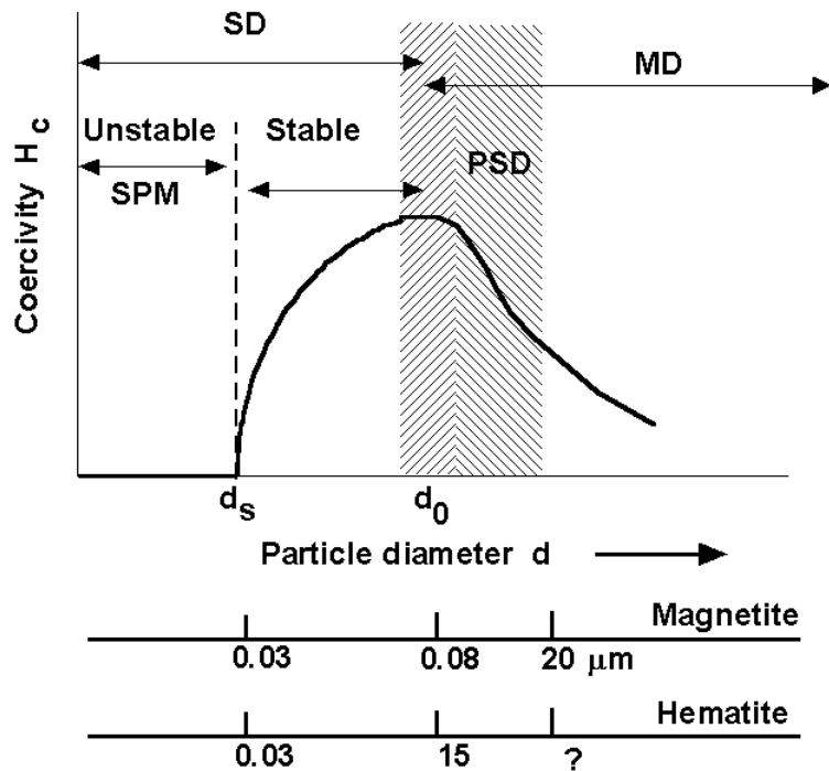
Figure 3.1.4: Evolution of the coercive force H_c within magnetite and hematite grain size allowing the definition of different magnetic behaviours: super paramagnetic (SP), single domain (SD), pseudo single domain (PSD) and multi domain (MD). (IRM Minnesota).
