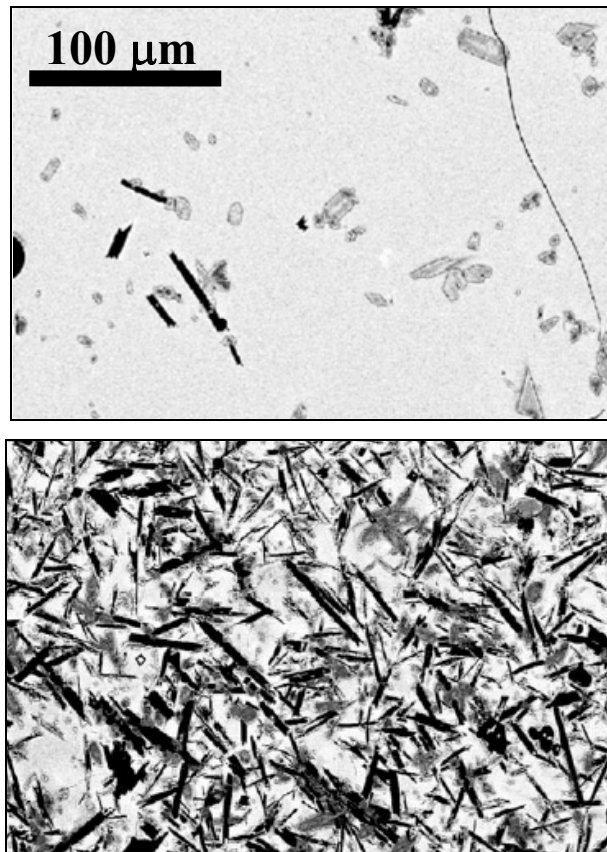
Figure 1.1.8: Typical BSE images on artificial quenched lava samples of the pāhoehoe (top) and the ‘ā’ā (bottom) type (Cashman & al. 1999).
