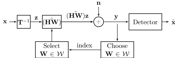
Figure 5.7: LRA detector bloc-scheme with precoding.
