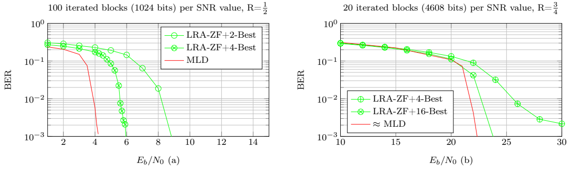
Figure 4.4: BER as a function of E_b/N_0 , Complex Rayleigh 4 \times 4 SM-MIMO-SC system, LRA-ZF+ K -Best and ML detectors, 4-QAM modulations at each layer (a) and 64-QAM modulations at each layer (b).
