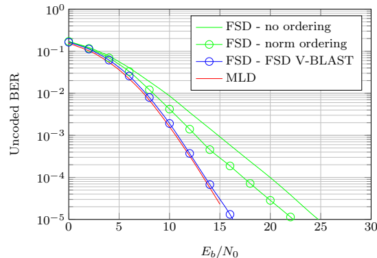
Figure 3.8: Unencoded BER as a function of E_b/N_0 , Complex Rayleigh 4 \times 4 SM-MIMO-SC system, FSD algorithms with p = 1 and ML detectors, 4-QAM modulations at each layer.
