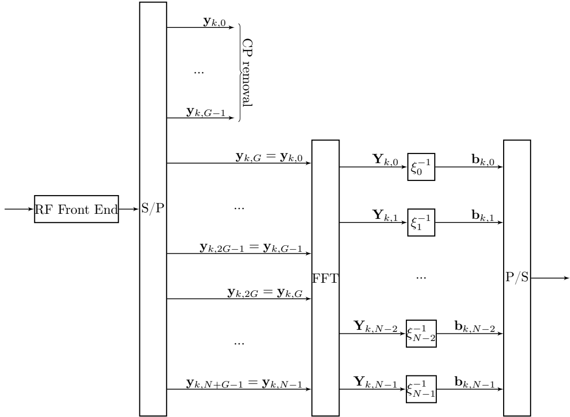
Figure 2.5: OFDM receiver.
