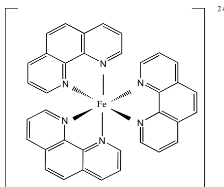
Figure 83 Complexe fer (II)- 1,10-phénanthroline
