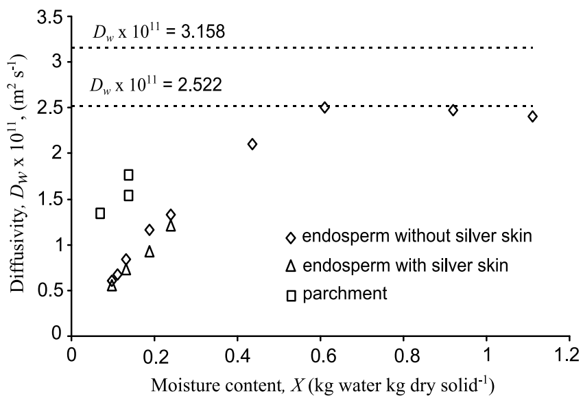
Figure 72. Variation of the diffusivity as a function of moisture content for the coffee bean endosperm and parchment.
