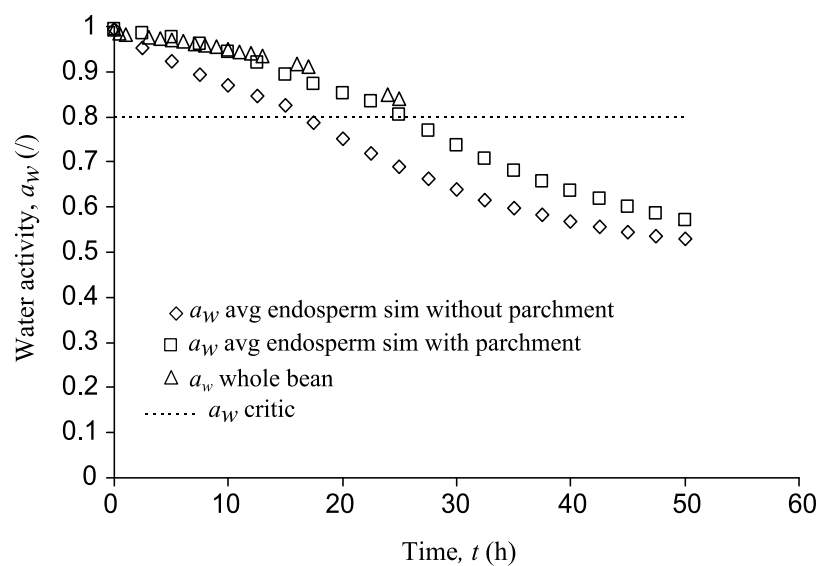
Figure 81. Simulation of water activity values of endosperm with and without parchment.
