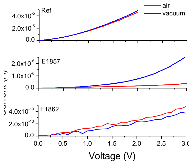
Figure 4.8 The dark I-V curves at RT in vacuum (blue line) and in air (red line) for a single wire from a reference sample (nanowire diameter dNW = 50 nm), E1857 sample (dNW = 55 nm), and E1862 sample (dNW = 60 nm).
