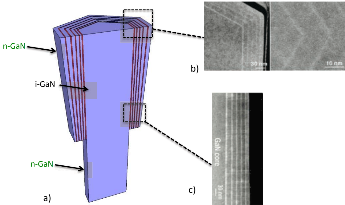
Figure 5.3 a) Diagram of the core-shell MQW structure b) HAADF STEM images of the InGa N MQW cross-section orthogonal to the wire length direction show a hexagonal shape with m-plane facets c) HAADF STEM image of a cross-section of a wire parallel to the growth direction taken along the [1120] zone axis.
