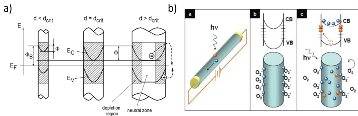
Figure 1.10 a) Dependence of the depletion region on the nanowire diameter. b) Trapping and photoconduction mechanism in ZnO nanowires.
