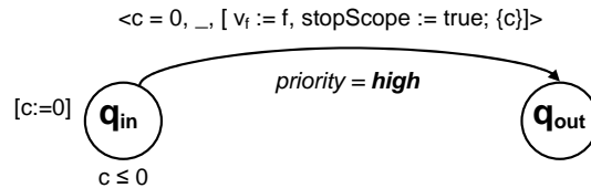
FIGURE 3.10 – La machine &lt;throw&gt;
