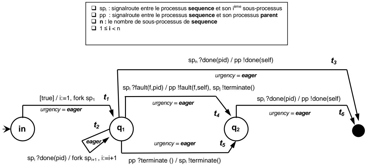
FIGURE 4.18 – Le processus <sequence>
