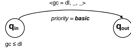
FIGURE 3.9 – La machine &lt;wait until&gt;
