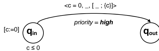
FIGURE 3.7 – La machine <empty> instantanée
