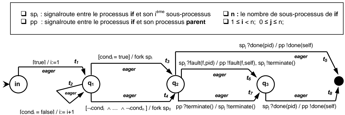
FIGURE 4.19 – Le processus <if>
