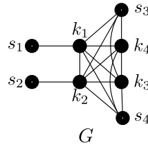
Figure 2.2: example of split graph G with partitioning S'(G) = \{s_1, s_2\} , K'(G) = \{k_1, k_2\} and R'(G) = \{s_3, s_4, k_3, k_4\} .
