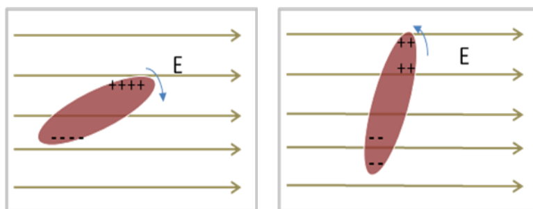
Figure 1- 12: RESPONSE TO ELECTRIC FIELD BY POSITIVE AND NEGATIVE ANISOTROPIC LIQUID CRYSTAL
