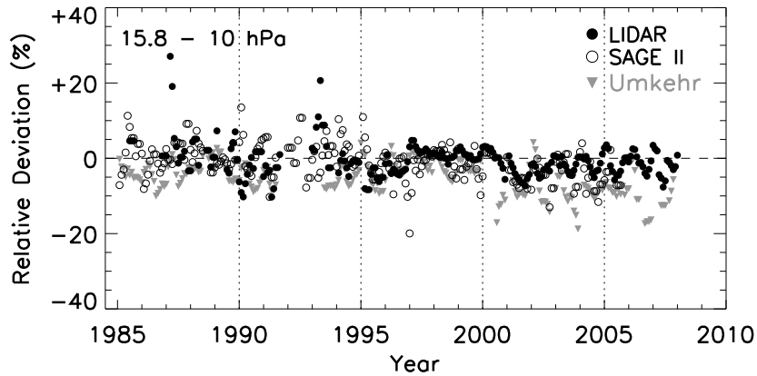
Figure 3.9: Monthly averaged differences of SBUV(/2) with lidar, SAGE II and Umkehr at 15.8–10 hPa. The dashed line represents 0 % and the dotted lines represent year 1990, 1995, 2000, and 2005. Data are smoothed by 3 month running mean.
