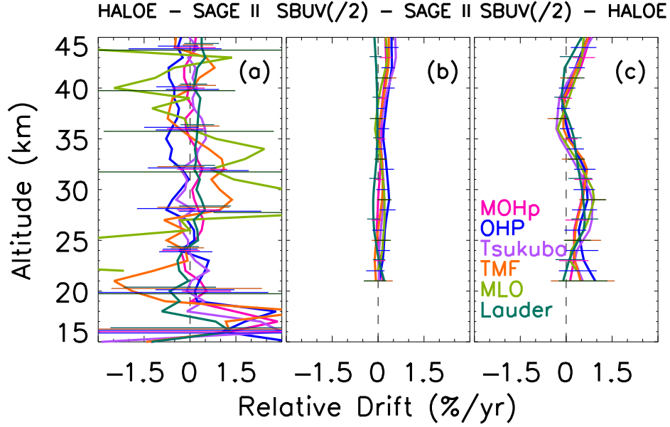
Figure 4.7: a) The drifts of HALOE in comparison with SAGE II as reference (see Eq. 4.2) at various stations. b) The drifts of SBUV(2) with SAGE II as reference (see Eq. 4.2). c) Same as (b), but with HALOE as reference (see Eq. 4.3). The error bars represent twice the standard deviation of the slope.
