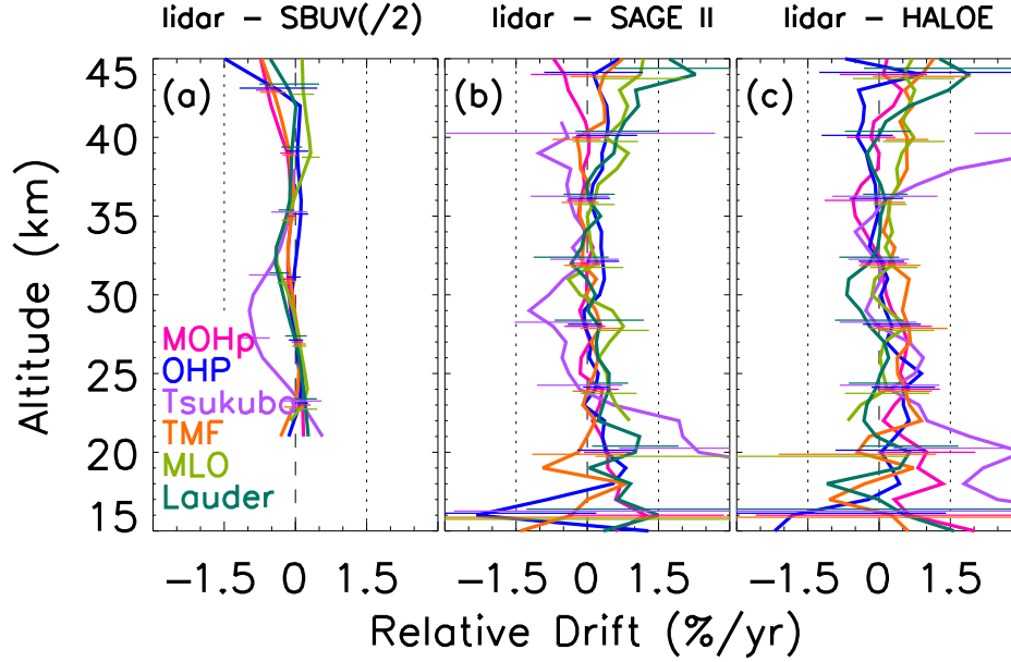
Figure 4.6: The drifts of various lidars for the comparison with SBUV(/2), SAGE II and HALOE as references \left(100 \times \frac{\text{lidar} - \text{ref}}{\text{ref}}\right) . The error bars correspond the 95% confidence interval of the slope.
