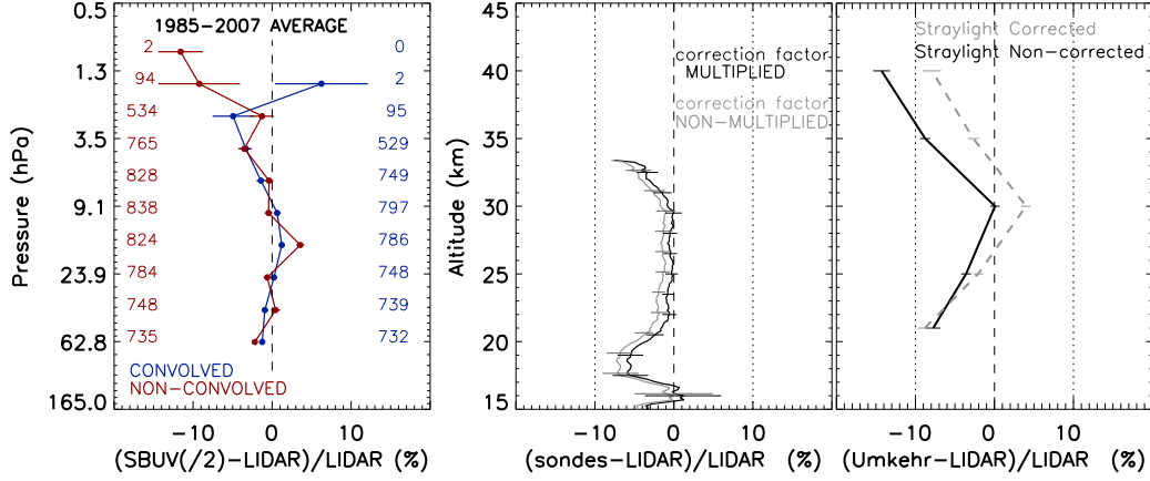
Figure 3.4: Left: Average bias between SBUV(/2) and lidar (with and without convolution using AKs and a priori). The number of analysed profiles with and without convolution are also provided in respective colours. Middle: Average relative deviation of ozone from lidar and ozonesondes, with and without multiplying by correction factor. Right: Average bias from the comparison of lidar with the original and stray light corrected Umkehr. The error bars represent twice the standard error. The dashed line represents 0% and the dotted lines represent -10 and 10%.
