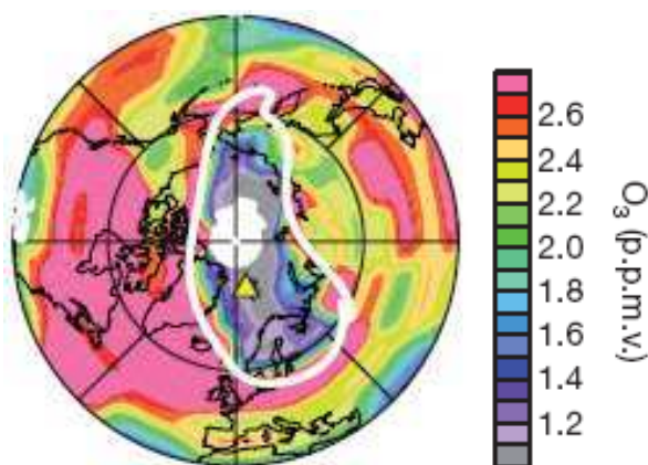
Figure 1.9: Arctic ozone loss in mid-March 2011 at an altitude of ~20 km (Taken from Manney et al., 2011).
