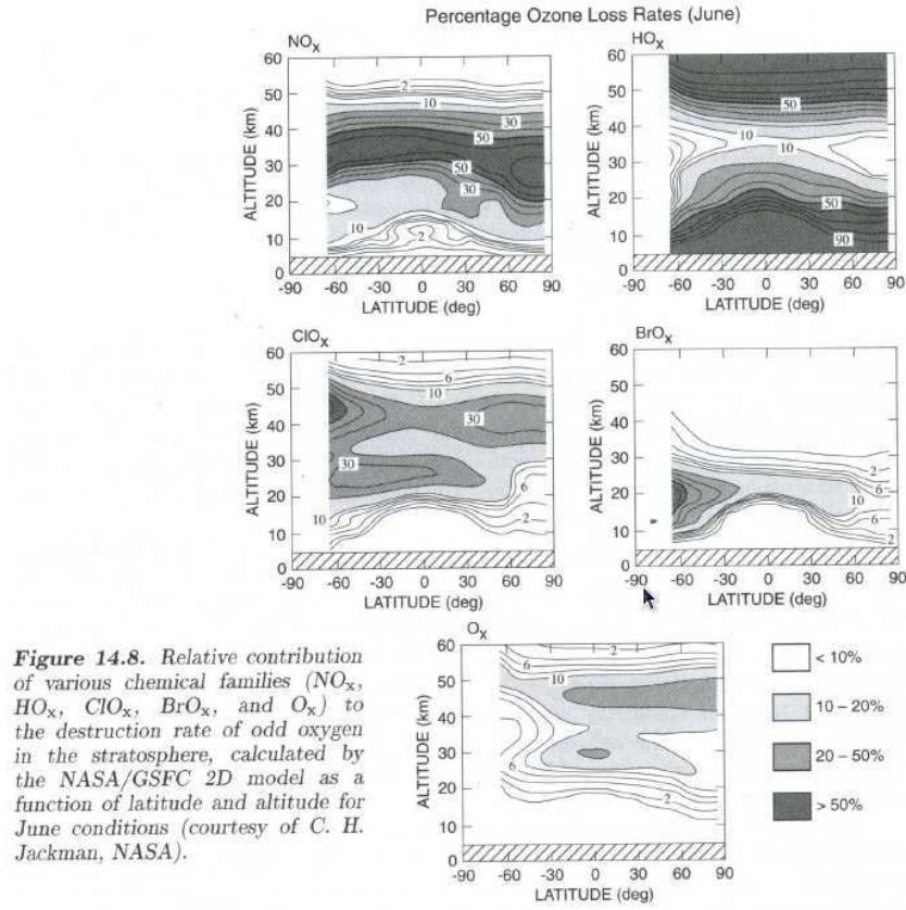
Figure 1.2: Vertical distribution of the relative contribution of various reaction cycles in depleting ozone at various latitudes (from Brasseur et al., 1999).
