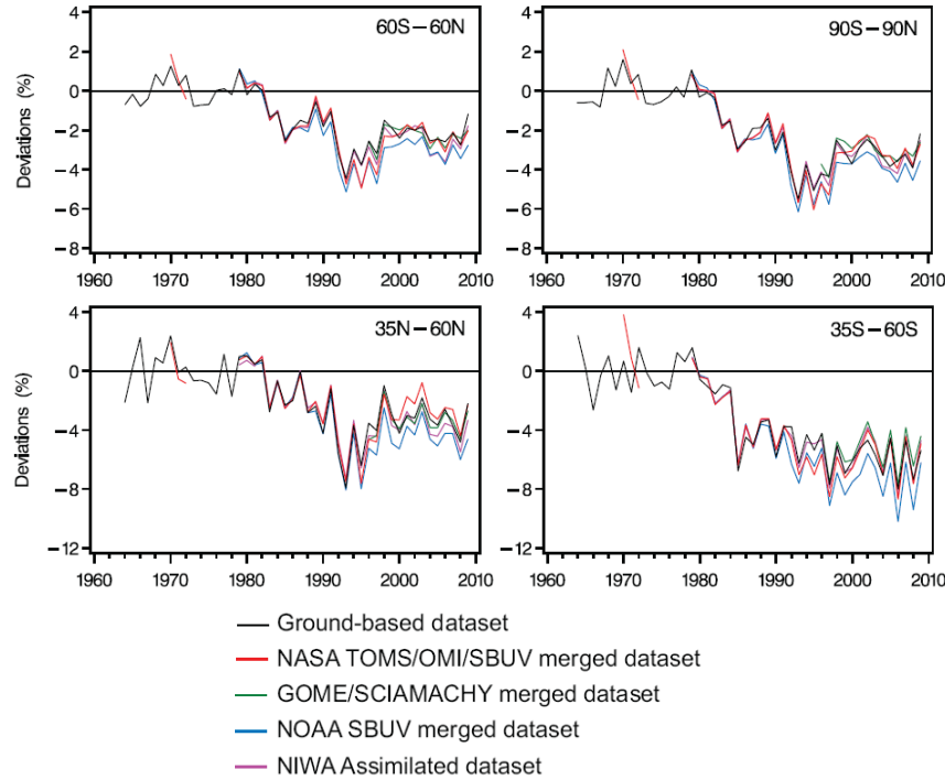
Figure 1.11: The deseasonalised total ozone deviations in 1964–2009 for the latitude bands (60°S–60°N, 90°S–90°N, 35°N–60°N and 35°S–60°S) estimated from different data sets. The zero line indicates the pre-1980 level (Taken from WMO, 2011 ).
