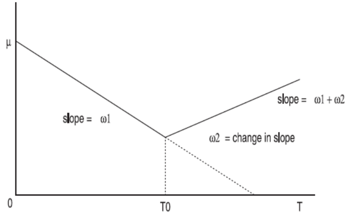
Figure 5.3: Demonstration of the PWLTs before the turnaround year ( T_0 ) and afterwards (Adapted from Reinsel et al., 2002).
