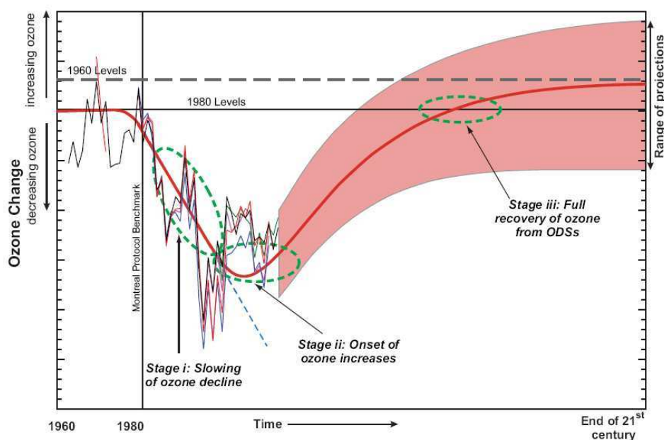
Figure 1.14: Schematic picture showing the evolution of ozone column between 60°S and 60°N in 1960–2100. The red curve shows the ozone observed to date and projected to future and the shaded region represents the simulation results of the ozone level for the future. The green circles denote different stages of ozone evolution (courtesy : WMO, 2011).
