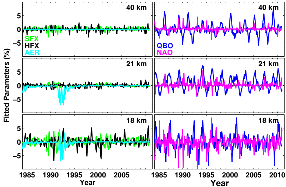
Figure 5.21: Time series of the fitted signals of solar flux, heat flux, aerosols, QBO and NAO at 18, 21 and 40 km computed for the average data at OHP.
