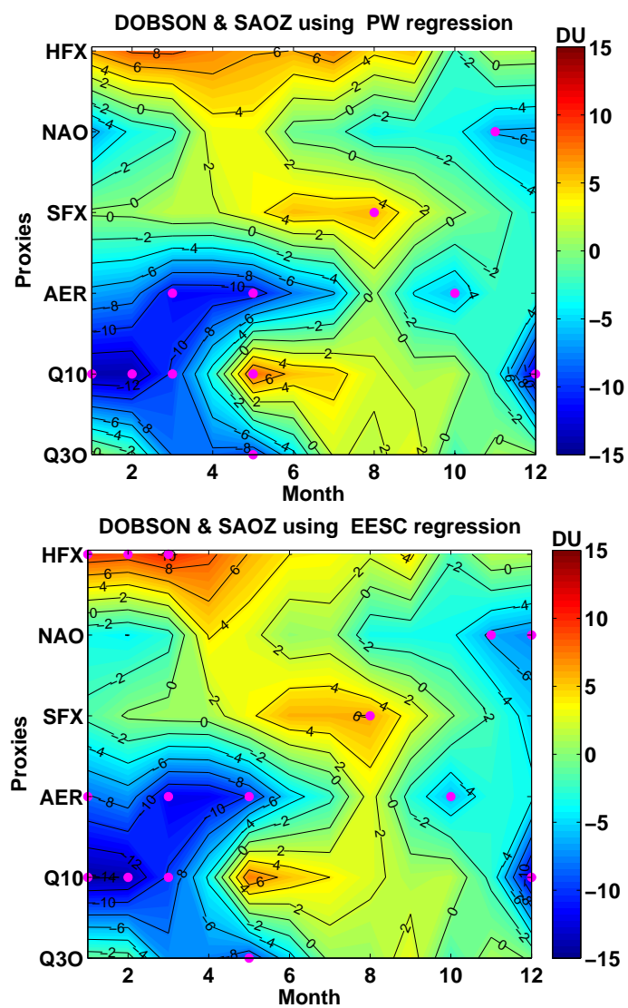
Figure 5.10: The influence of individual explanatory variables on the variability of combined Dobson and SAOZ ozone column data at OHP analysed using both PW (top panel) and EESC (bottom panel) regressions.
