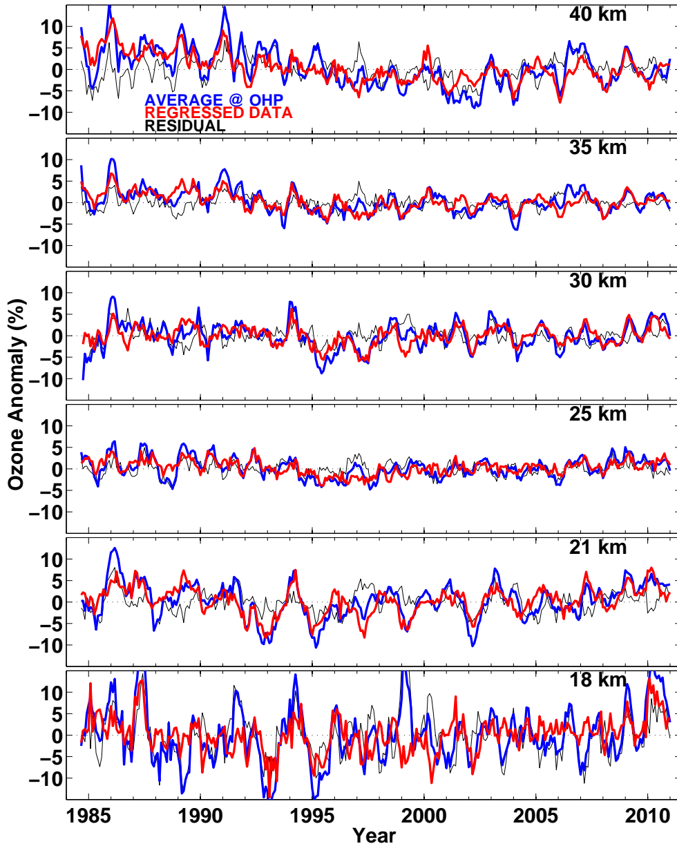
Figure 5.20: Time series of the ozone anomaly, the PW regression model and the residual at 18, 21, 25, 30, 35 and 40 km calculated from the average data at OHP.
