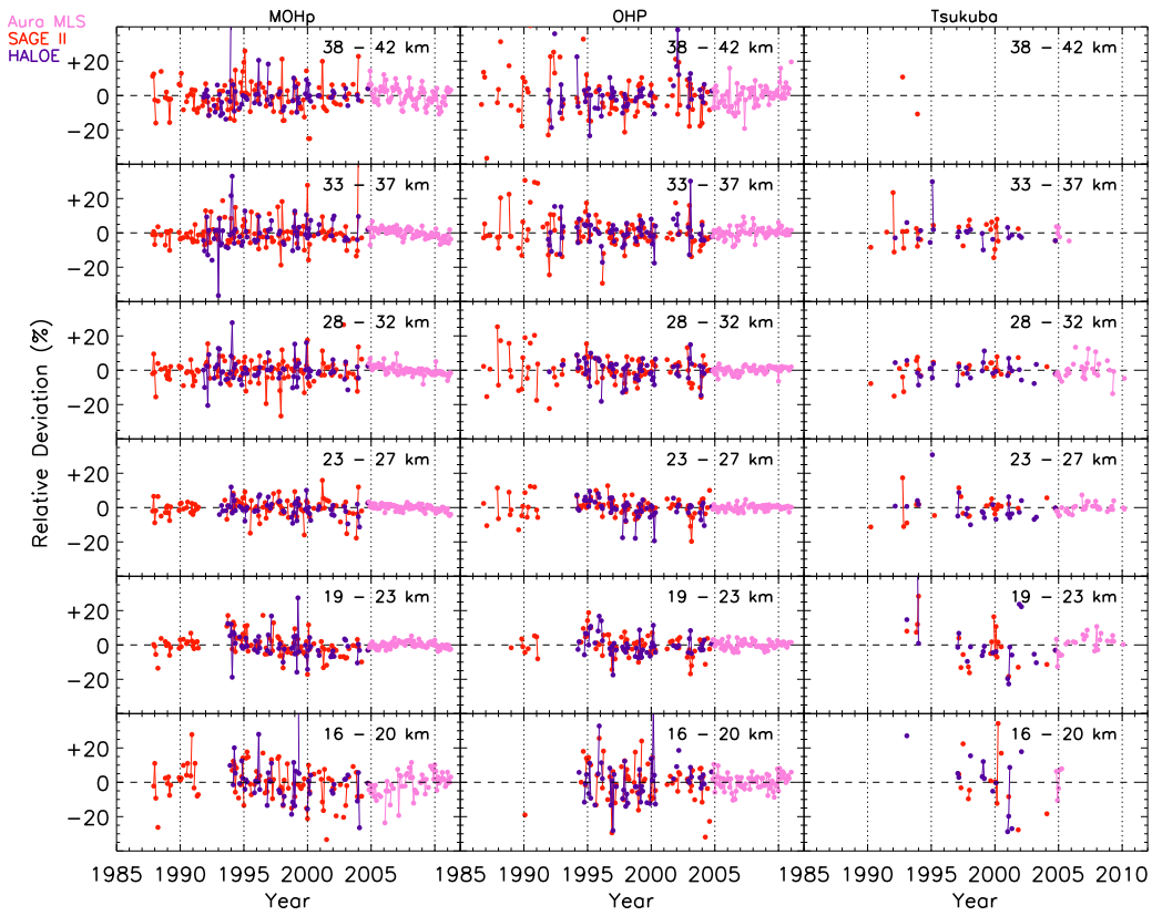
Figure 4.9: Temporal evolution of the bias removed monthly averages of the relative differences of SAGE II, HALOE and Aura MLS with ozone lidar at MOHp (left panel) , OHP (middle panel) and Tsukuba (right panel). The dashed horizontal line represents 0%.
