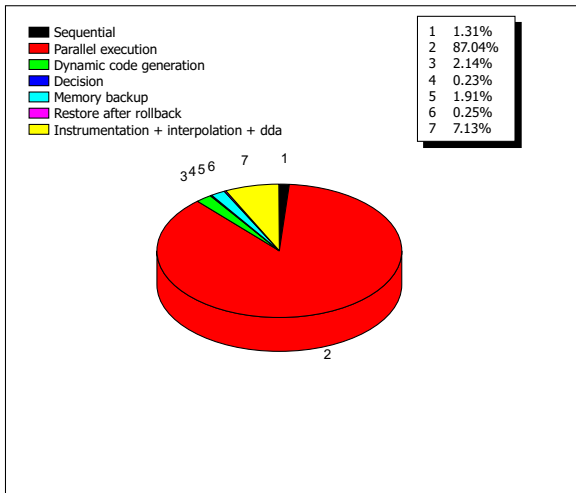
(a) Covariance
