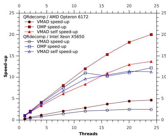
(c) QRdecomp
