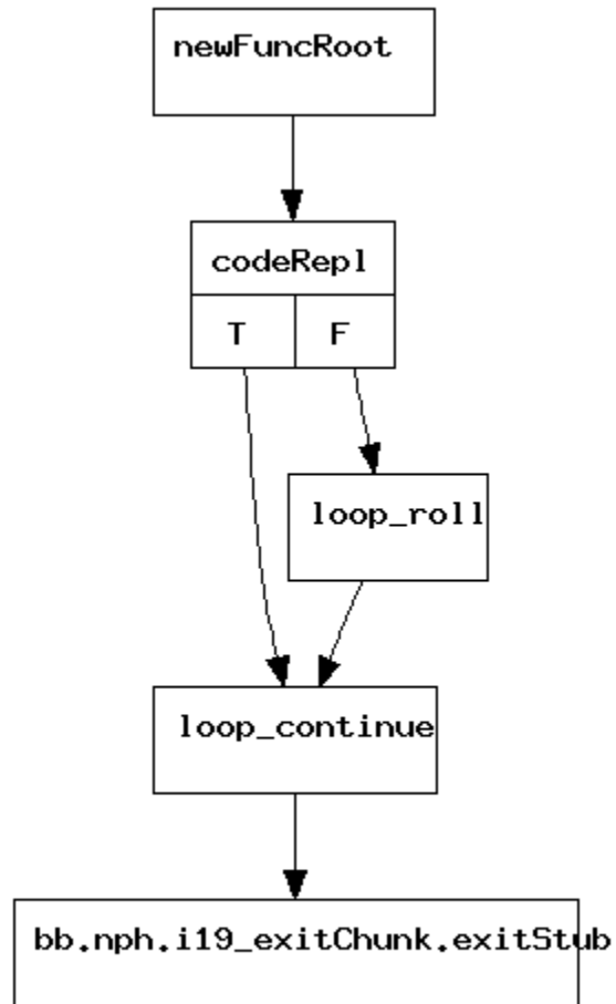
CFG for 'main_bb.nph.i19_viCond_par_1_Orig' functi
