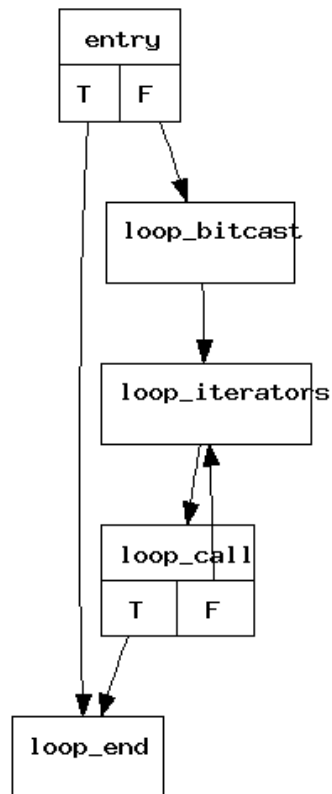
CFG for 'main_bb.nph.i19_viCond_par_1_Orig_bb.nph.i19_viCond_par_1_structArg_omp' func
