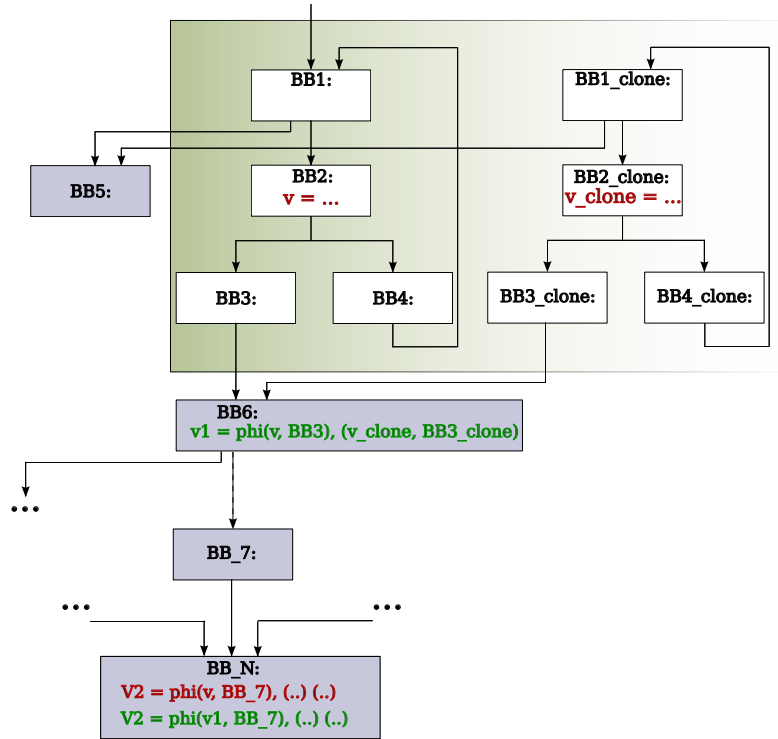
Figure 5.14: Control flow graph with \phi – nodes
