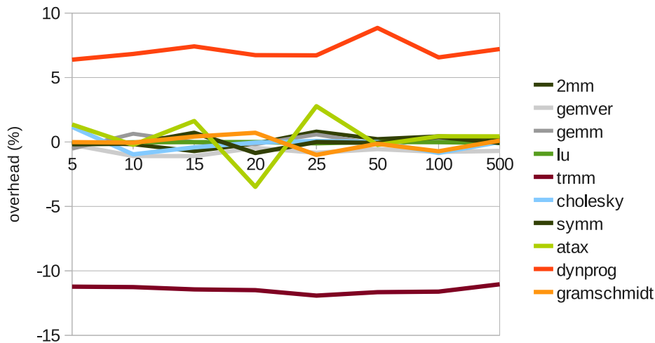
Figure 4.4: Chunking time overhead
