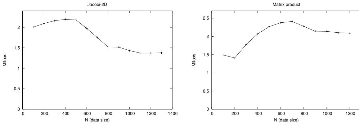
Figure 4.2: Performance of a simple parallel version relative to the data size.
