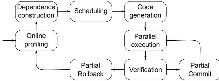
Figure 5.1: Main phases of the speculative system.
