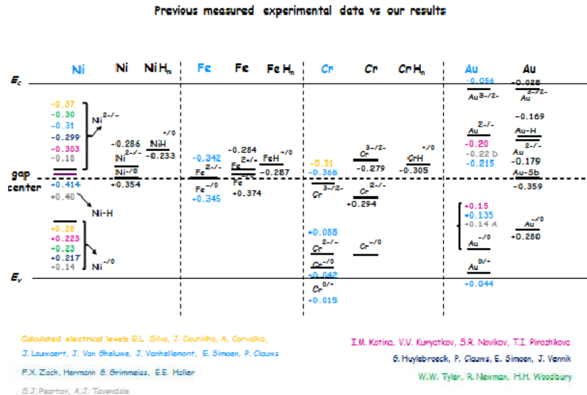
Fig. S.9. Deep-level parameters and assignments of electron and hole traps in Fe-, Cr-, Ni- and Au-implanted Ge [2-5, 7-10, 12, 17, 23-27].
