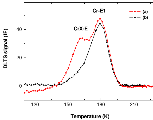
Fig. 4.14. DLTS spectra of Cr contaminated n -type Ge samples annealed 5 hours at 500 °C, treated 2 min by \text{HNO}_3 and (a) not annealed or (b) annealed 30 min at 450 °C. The scans were recorded with the pulse sequence (-10V; -5V) and at a rate window of 100 s -1 with pulse duration t_P = 200 \mu\text{s} .
