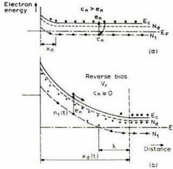
Fig. 2.4. A Schottky contact on n-type semiconductor (a) at low bias and (b) under the reverse bias V_r .
