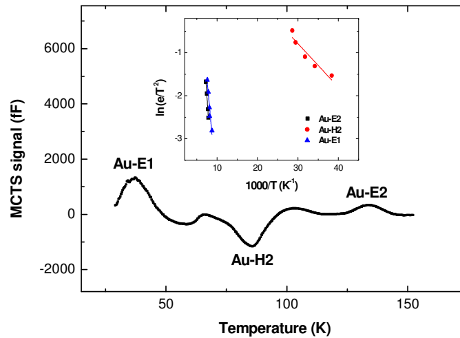
Fig. S.6. MCTS scan recorded in the Au-diffused sample at -5V with an optical pulse duration of 5 ms and rate window of 200 \text{ s}^{-1} .
