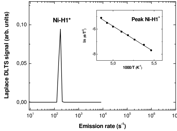
Fig.S.8. Laplace DLTS spectrum recorded in the Ni-diffused p-type Ge sample. The analytical parameters are: t_F = 200 \mu\text{s} , bias (-5\text{V}, -2\text{V}) and T = 200 \text{ K} . The inset displays the Arrhenius plot of the hole trap Ni-H1*.
