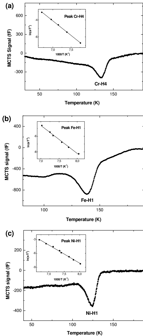
Fig.S.5. MCTS scan for (a) Cr-, (b) Fe- and (c) Ni –contaminated n -type Ge at -5V with an optical pulse duration of 5 ms and rate window of 80 s -1 . The inset displays the Arrhenius plot of the hole trap TM-H1.
