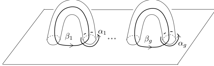
Figure 2.1: The standard surface \Sigma_{g,1} and its system of meridians and parallels (\alpha, \beta) .
