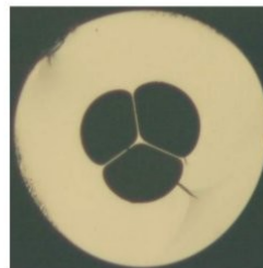
Fig. 1. (Color online) Microscope image of the manufactured SWF.
