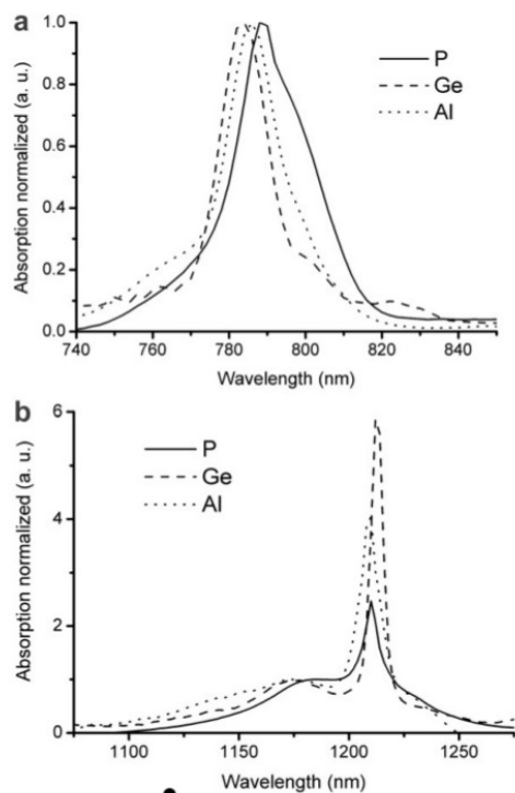
Fig. 3. Normalized GSA spectra of the (a) {}^3\text{H}_6 \rightarrow {}^3\text{H}_4 and (b) {}^3\text{H}_6 \rightarrow {}^3\text{H}_5 transitions in the Tm(Al), Tm(Ge) and Tm(P) samples, respectively. Curves in (b) are normalized to the height of the shoulder around 1175 nm (see text).
