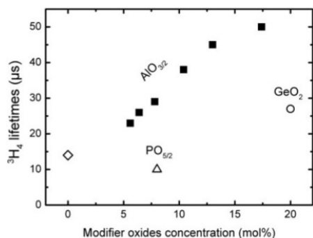
Fig. 5. {}^3\text{H}_4 -level lifetime ( \mu\text{s} ) from Tm(Al) (filled squares), Tm(Ge) (circle) and Tm(P) (triangle) samples.
