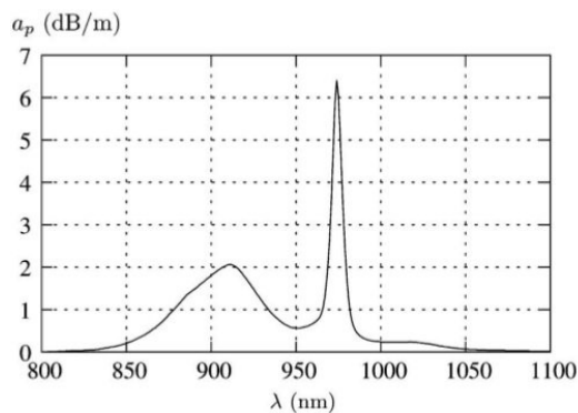
Fig. 7. Absorption spectrum measured in the fiber.
