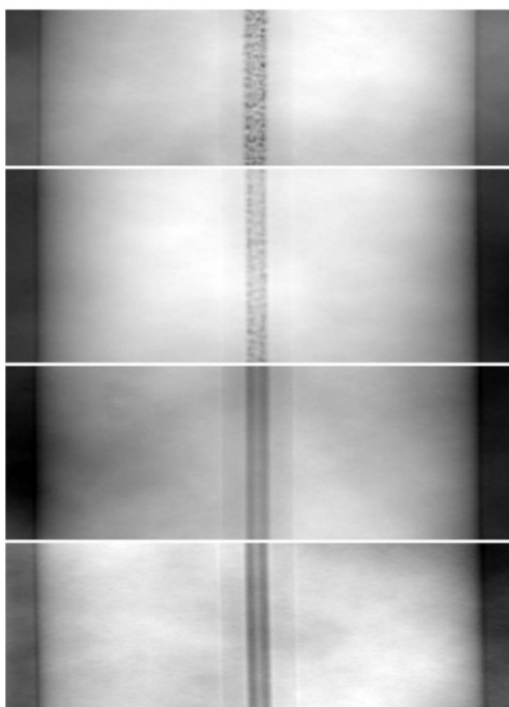
Fig. 1. QPM measurement of calcium-doped fibers. The bright region is the 125\ \mu\text{m} diameter cladding, and the core is the dark central region (diameter \sim 8\ \mu\text{m} ). The calcium concentration in the doping solution is (from top to bottom) 1 , 0.1 , 0.01 , and 0\ \text{mol/l} .
