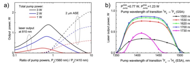
Fig. 7. (a) Laser output at 810 nm and total power of the ASE originated from the {}^3\text{F}_4 level vs. ratios of pump power at 1560 and 1410 nm. (b) Dependence of the laser output on the pump laser wavelengths.
