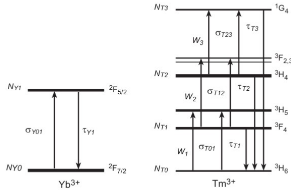
Fig. 4. Energy manifold labeling for the rate equation analysis of the \text{Tm}^{3+}/\text{Yb}^{3+} co-doped system.
