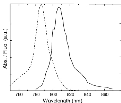
Fig. 2. Normalized absorption (dash) and emission (solid) spectra of the \text{Tm}^{3+}: {}^3\text{H}_6 \Rightarrow {}^3\text{H}_4 transition in a silica fiber.
