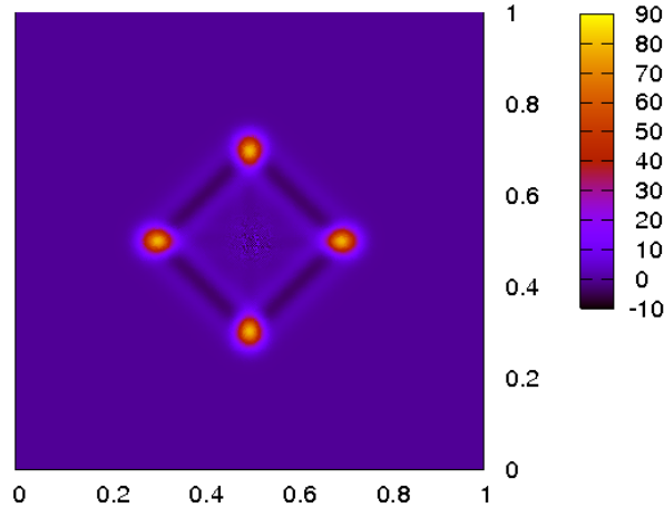
FIGURE 4.2 – Solution fondamentale. On trace la quantité E(t, \mathbf{x}) = \sum_{i=1}^4 U^i(t, \mathbf{x})
