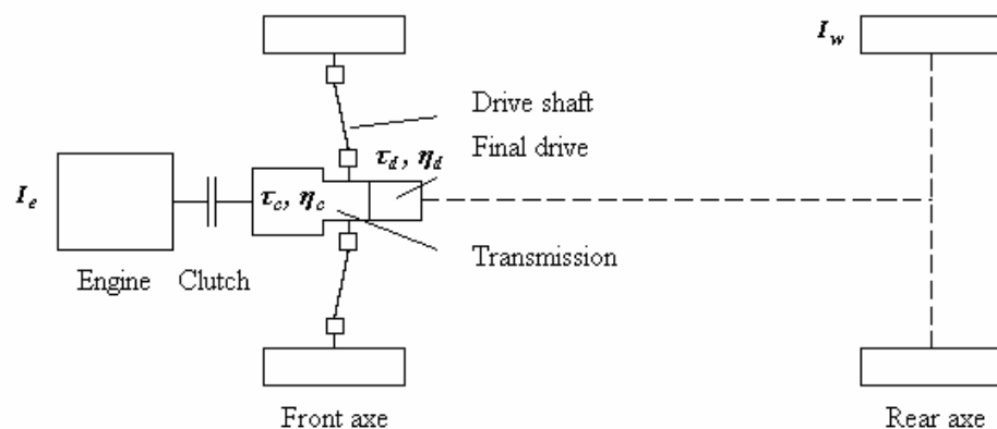
Figure 4.6: Driveline Notations
