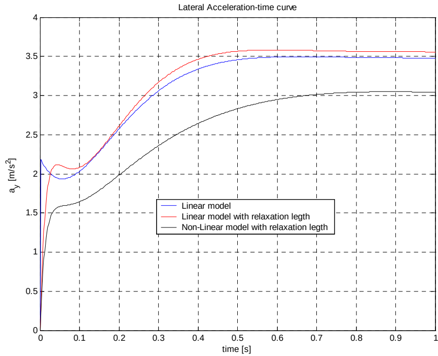
Figure 5.26: Lateral Acceleration-time curve.
