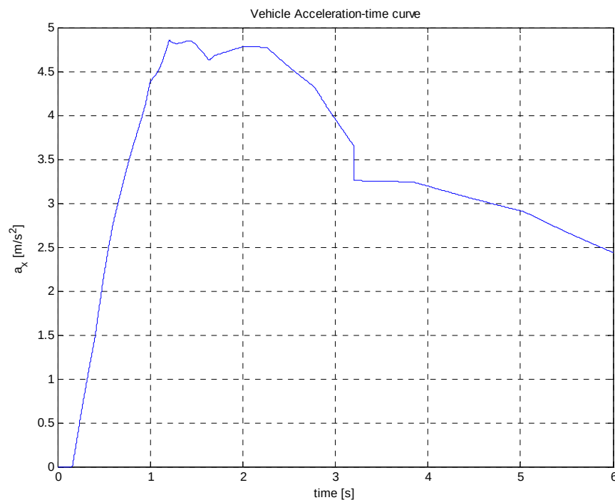
Figure 4.27: Acceleration-time curve.
