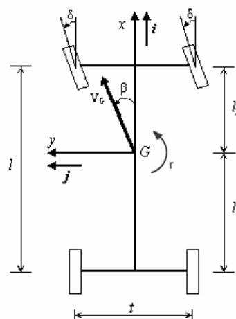
Figure 5.1: Vehicle Model.
