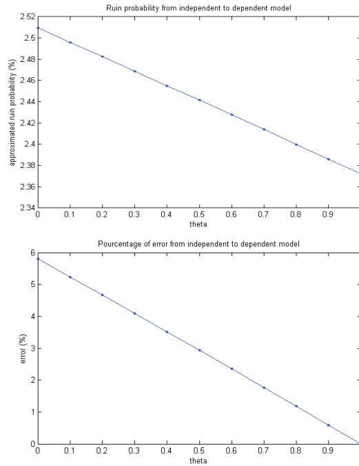
FIGURE 3.6 – Comparaison between the dependent model and the independent model
