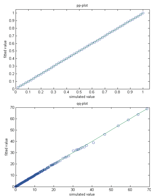
FIGURE 3.5 – PP-plot and QQ-plot for the simulated data versus the fitted distribution
