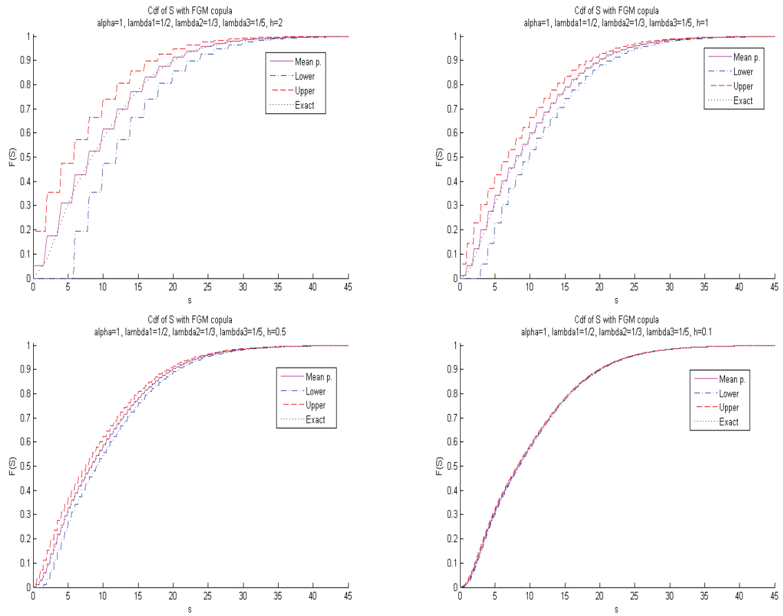
FIGURE 1.4 – Discretized cdf's vs exact cdf for 3 risks
