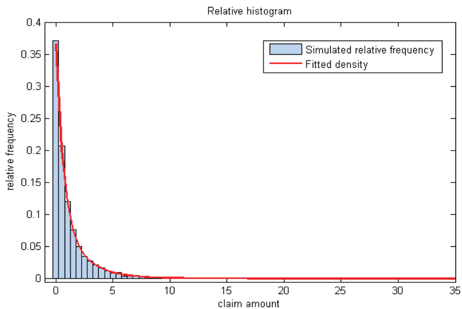
FIGURE 3.4 – Comparison between a relative histogram for the simulated data and the fitted density
