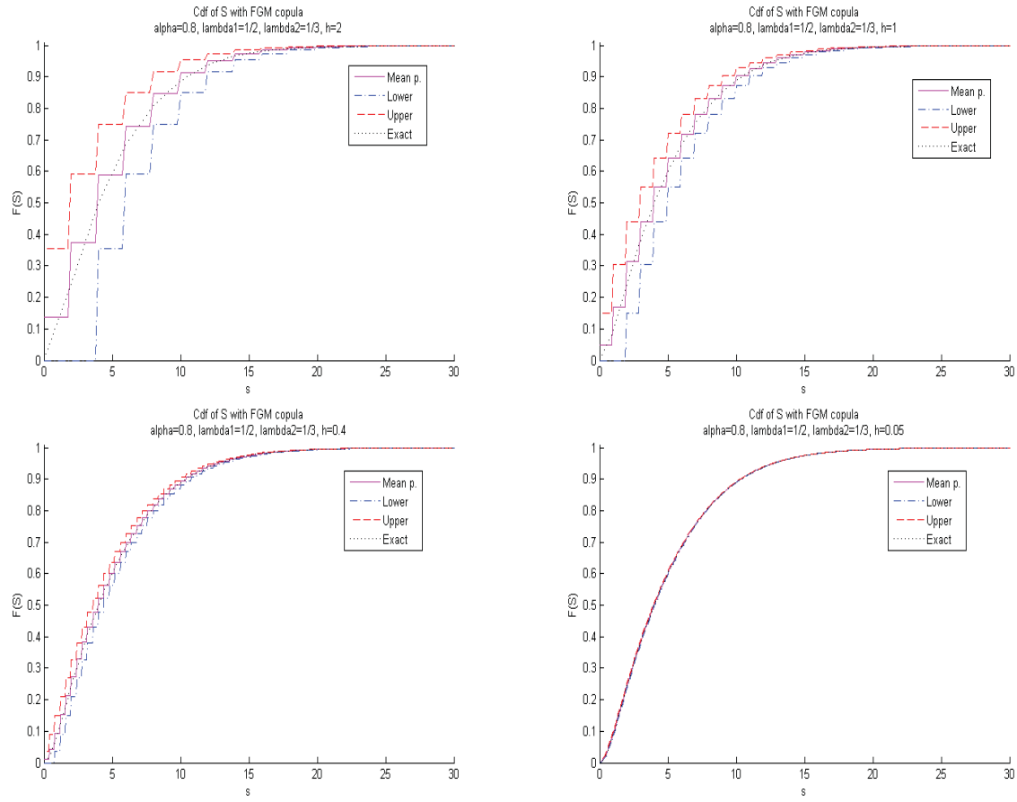
FIGURE 1.1 – Discretized cdf's vs exact cdf for 2 risks
