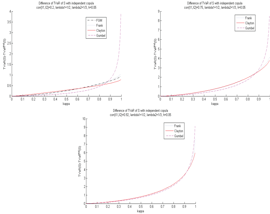
FIGURE 1.3 – TVaR of S with different copulas and correlation coefficients
