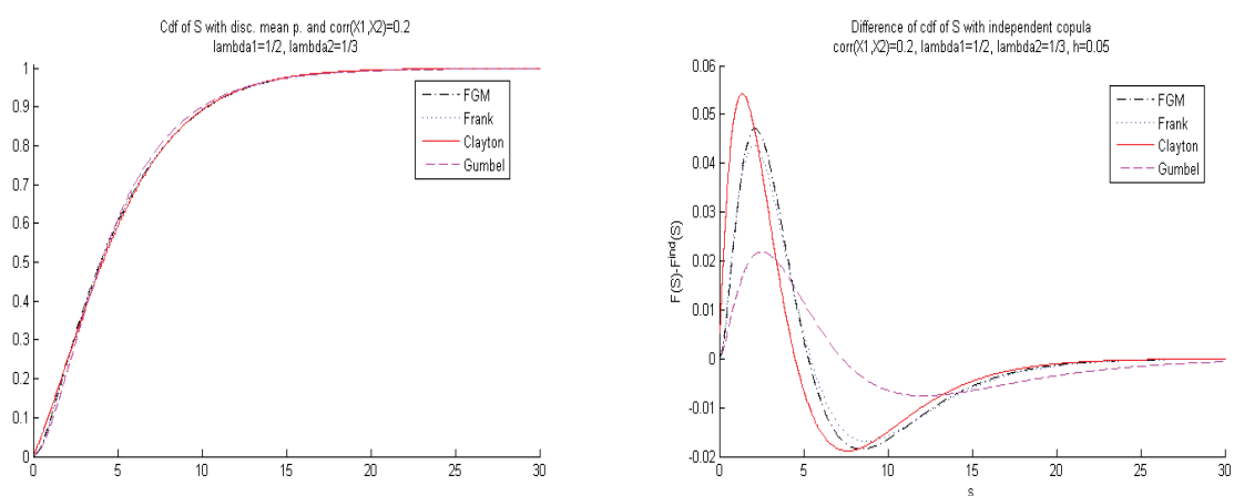
FIGURE 1.2 – Comparison of copulas with Corr(X_1, X_2) = 0.2
