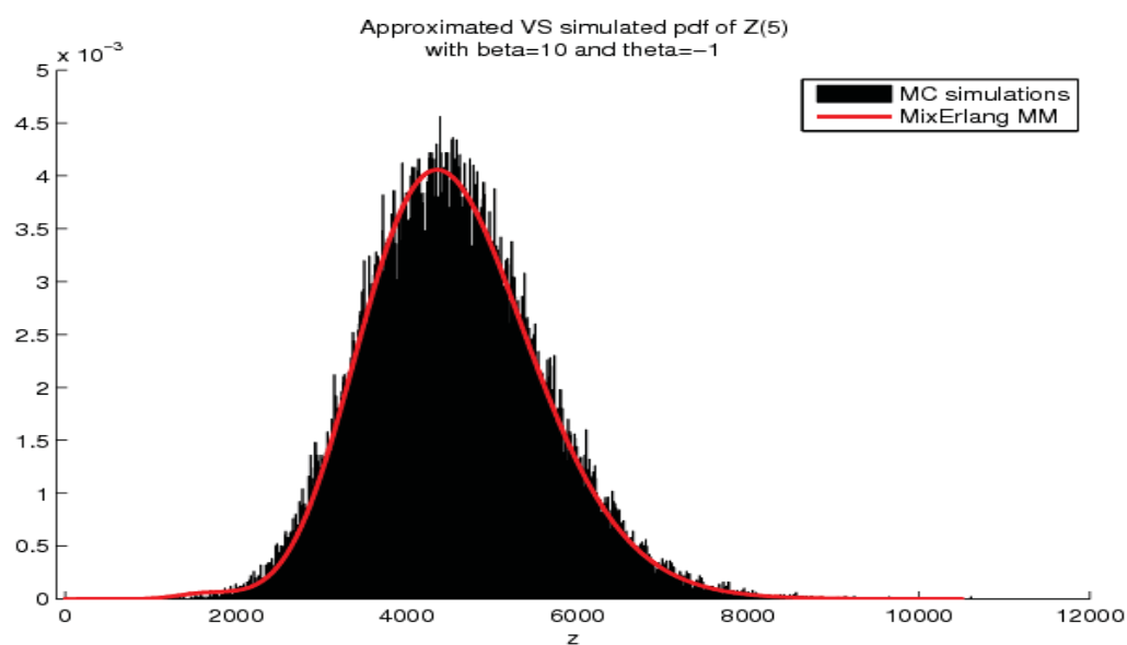
FIGURE 2.1 – Comparison between the simulated pdf and the approximated pdf with \theta = -1
