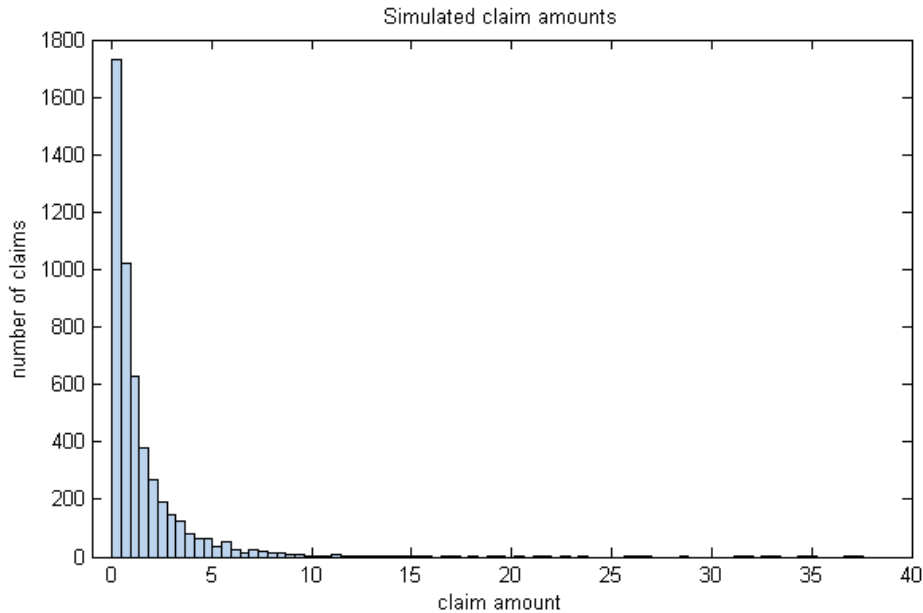
FIGURE 3.3 – Simulation of claim amounts from a GPD
