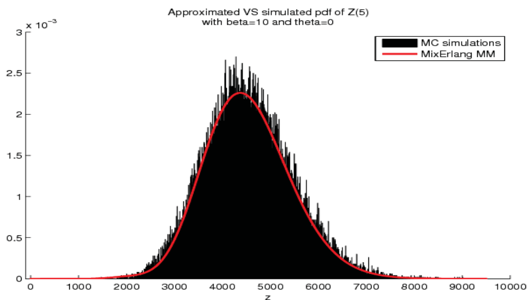
FIGURE 2.2 – Comparison between the simulated pdf and the approximated pdf with \theta = 0
