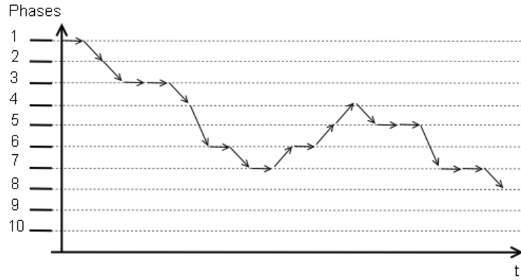
FIGURE 3.2 – Example of a cycle path with 10 phases
