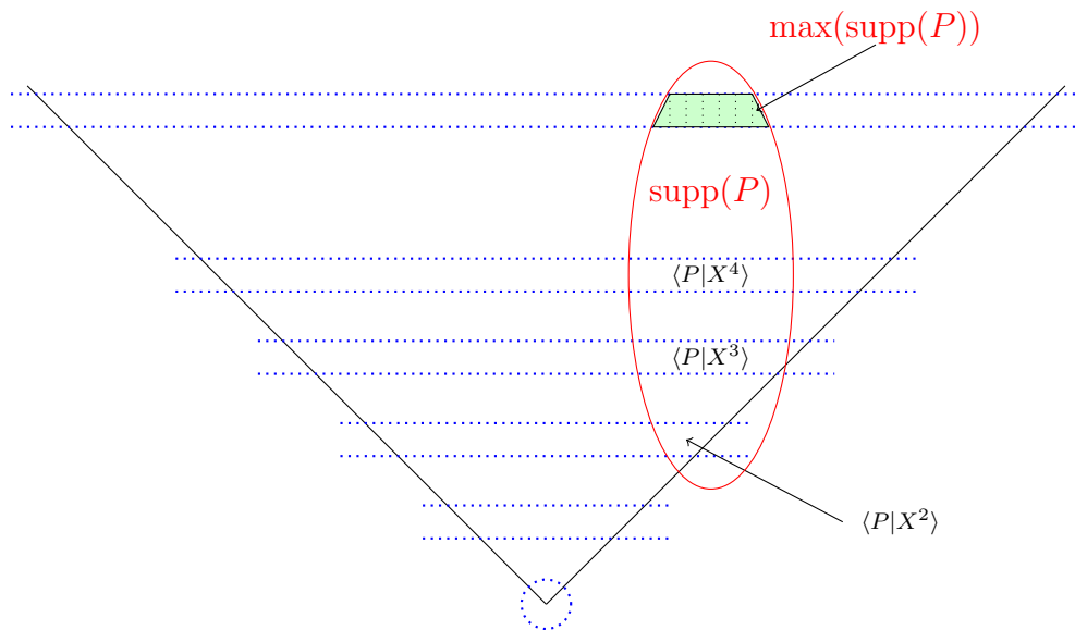
FIGURE 6 – Illustration de \max_{<}(P)
