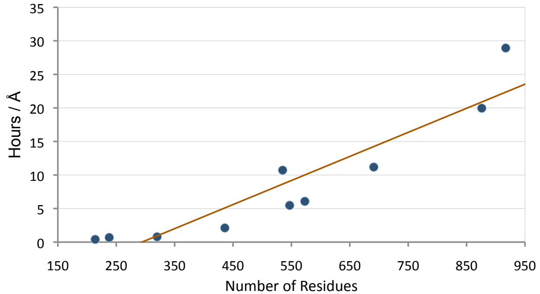
Figure 4.3: Relationship between the number of residues and the time (in hours) required to compute a path that is 1\text{\AA} long.
