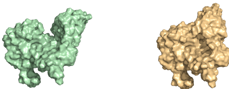
Figure 4.9: DAP: 1dap (left) and 3dap (right)
