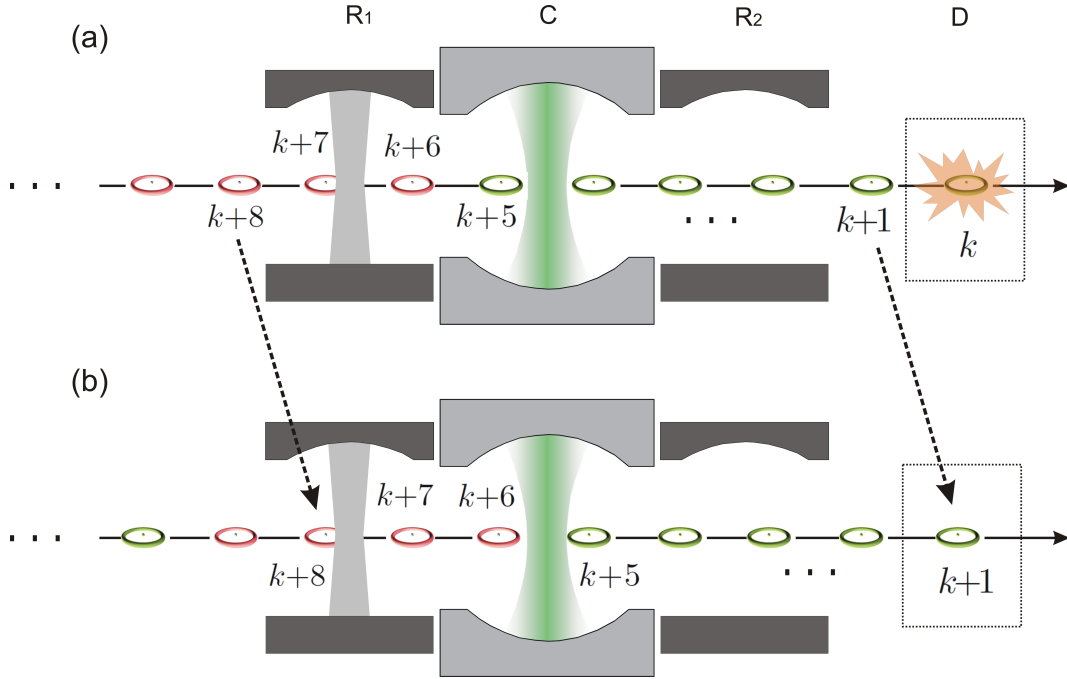
Figure III.1. Spatial configurations of the atomic samples when the sample k is detected (a) and when the controller chooses a feedback action (b). C: the cavity; R_1 and R_2 : the first and second Ramsey zones; D: the detector. The torus-shape elements represent the atomic samples: sensor samples (green) and control samples (red). The black solid arrow shows the atomic beam. The black dashed arrows link the same samples at the two moments. Several samples are labeled with their corresponding numbers.
