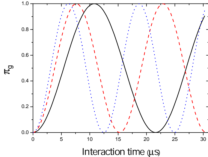
Figure I.15. Quantum Rabi oscillations in different photon number states |n\rangle . The photon numbers are n = 0 (black solid), 1 (red dashed), and 2 (blue dotted). The atom is prepared in the state |e\rangle before entering the cavity.
