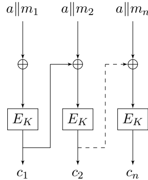
FIGURE 4.11 – Mode CBC-AREA
