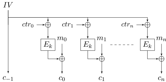
FIGURE 1.13 – Mode CTR
