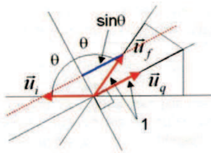
FIGURE II.14 – Relation entre \vec{u}_f , \vec{u}_i , \vec{u}_q et \theta (image O. Robach).
