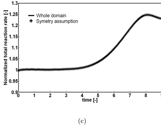
Figure 8.9: Snapshot comparison between two direct numerical simulations of flame-vortex interactions considering on the one hand the whole domain (a) and on the other hand an half of the domain (b). Both computations lead to the same flame temperature and vorticity fields shapes (a,b) and total reaction rate evolution (c).
