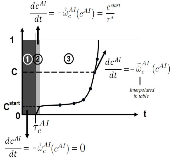
Figure 7.4: TKI model principle. Step 1: the AI delay is not reached yet and the progress variable reaction rate \widetilde{\omega}_c^{AI} = 0 . Step 2: the AI delay is reached and \widetilde{\omega}_c^{AI} = -c^*/\tau^* . Step 3: The progress variable reaches the value c^* and \widetilde{\omega}_c^{AI} is interpolated in the table.
