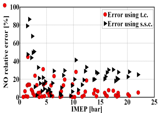
Figure 5.21: NO emissions relative errors, using a single step or a tabulated chemistry for the fuel oxidation in the flame, for the 59 operating points.
