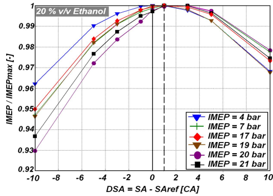
Figure 4.35: Spark advance variation around optimal engine settings at 3500 rpm for different loads (results from simulations): differences between the maximum IMEP and the IMEP at spark advance SA.
