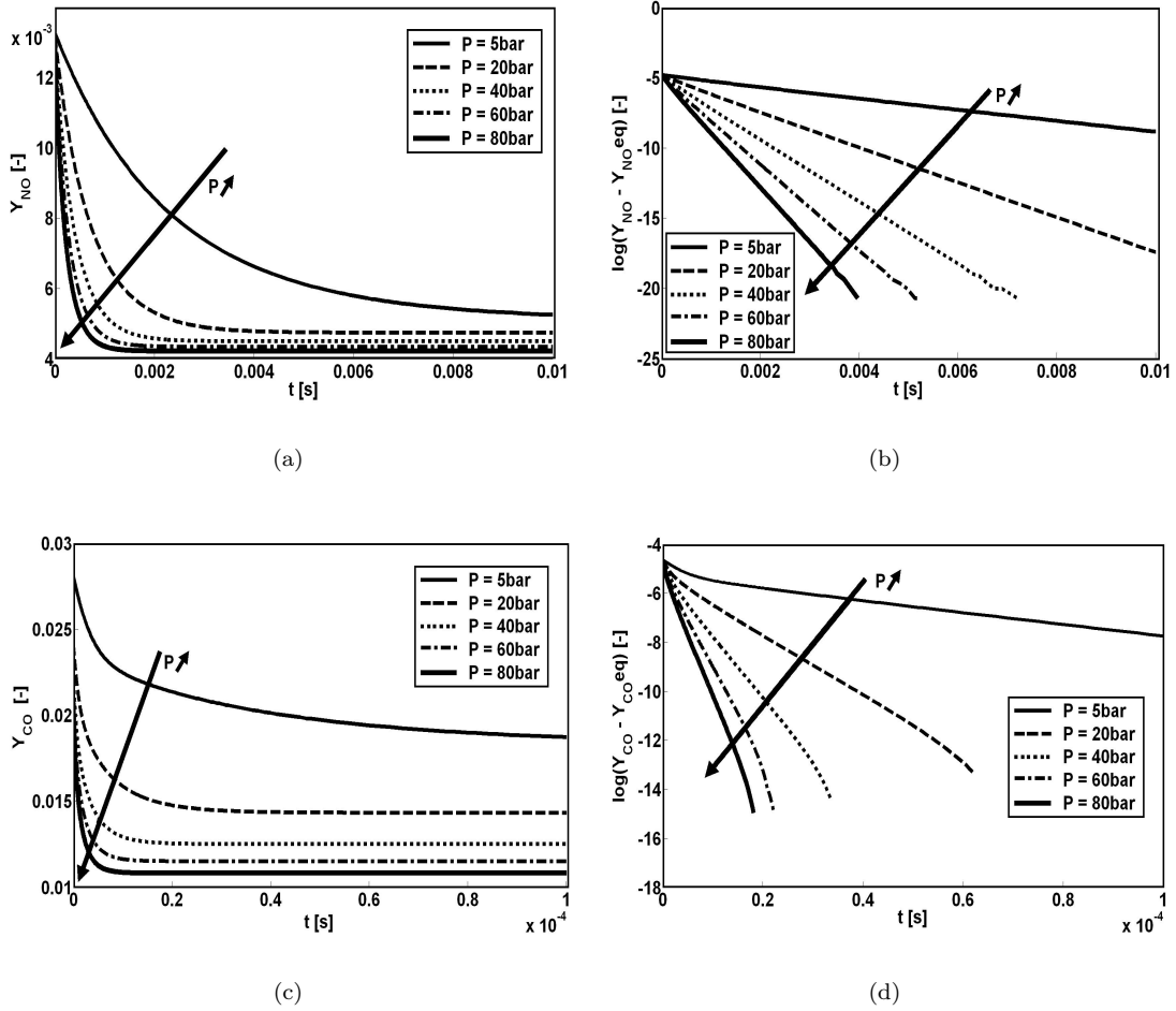
Figure 6.7: NO and CO evolutions at different pressures for \Delta_{NO} = \Delta_{CO} = 10^{-2} , \varphi = 1.0 , Y_{res}^u = 0\% and T_{eq}^b = 2500 K – (a) Y_{NO} , – (b) \log(Y_{NO} - Y_{NO}^{eq}) , – (c) Y_{CO} , – (d) \log(Y_{CO} - Y_{CO}^{eq}) .
