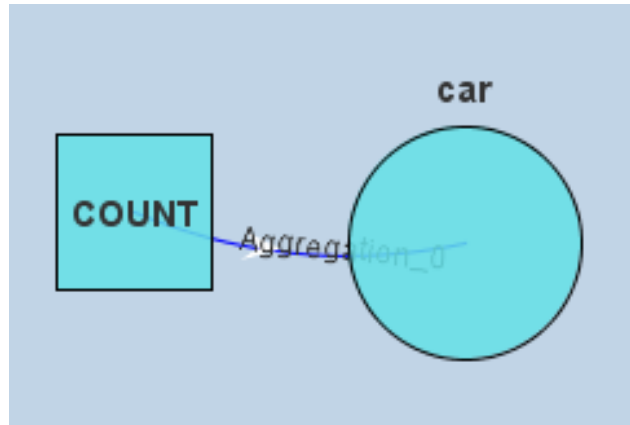
Figure 5.5: Aggregation query
